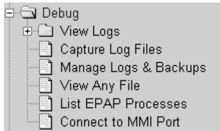
Figure 3-41. Debug Menu
