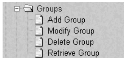
Figure 3-190. Groups Menu
