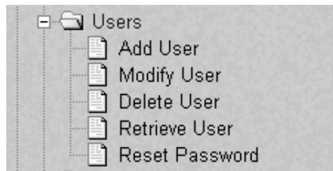
Figure 3-169. Users Menu
