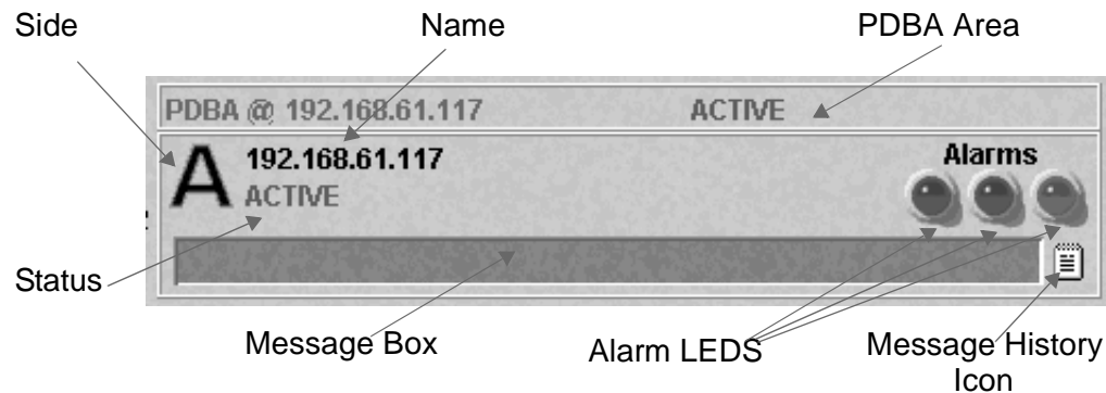
Figure 3-6. EPAP Area
