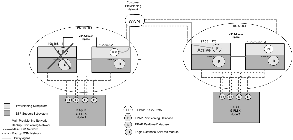
Figure 2-5. Virtual IP-Failure of Active PDBA
