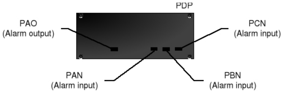
Figure 12: PDP Alarm Connectors (rear)
