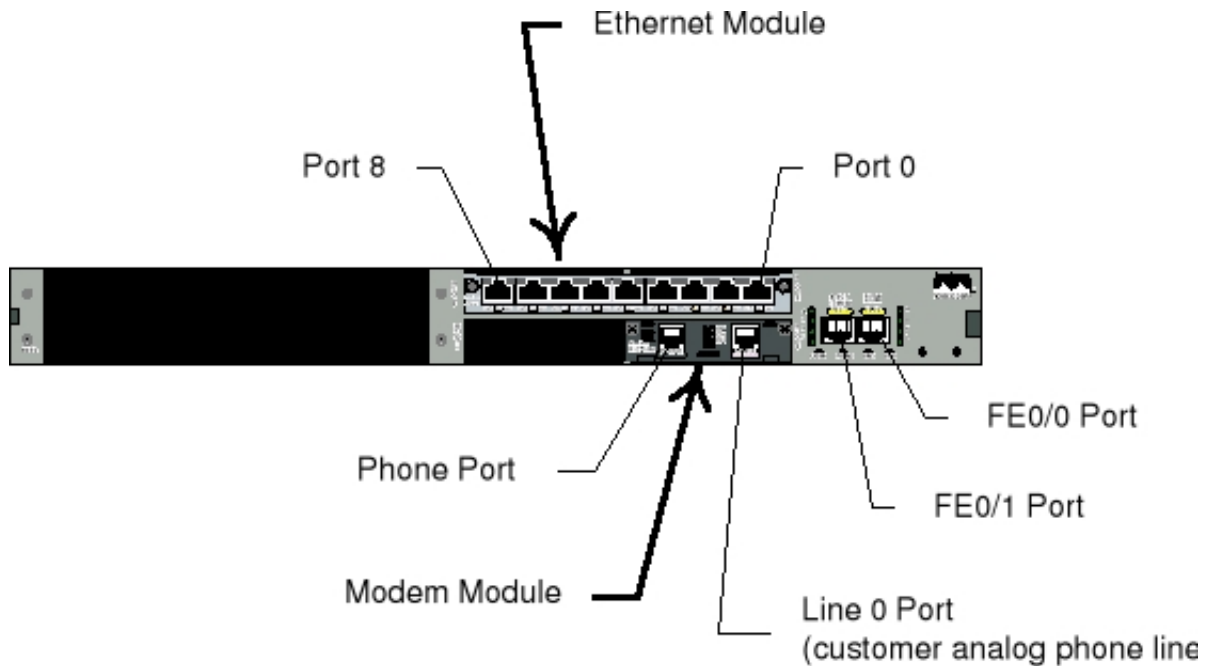
Figure 13: Modem Router (front view - as mounted?)
