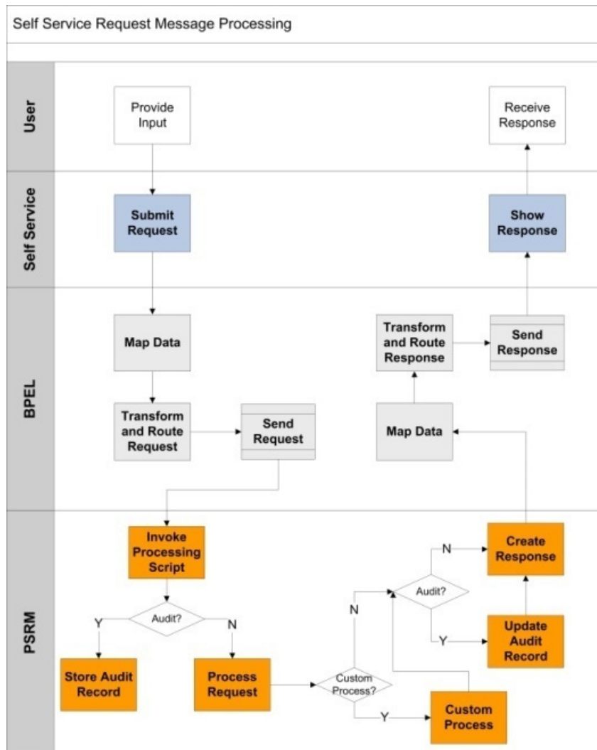
Figure 1: Message Processing
