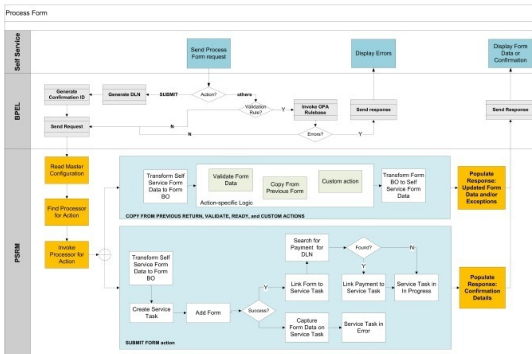
Figure 2: Handling Form Actions in PSRM
