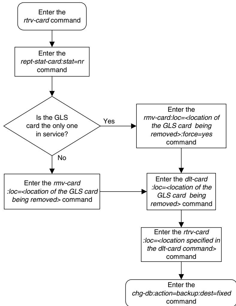
Flowchart 2-2. Removing a GLS Card
