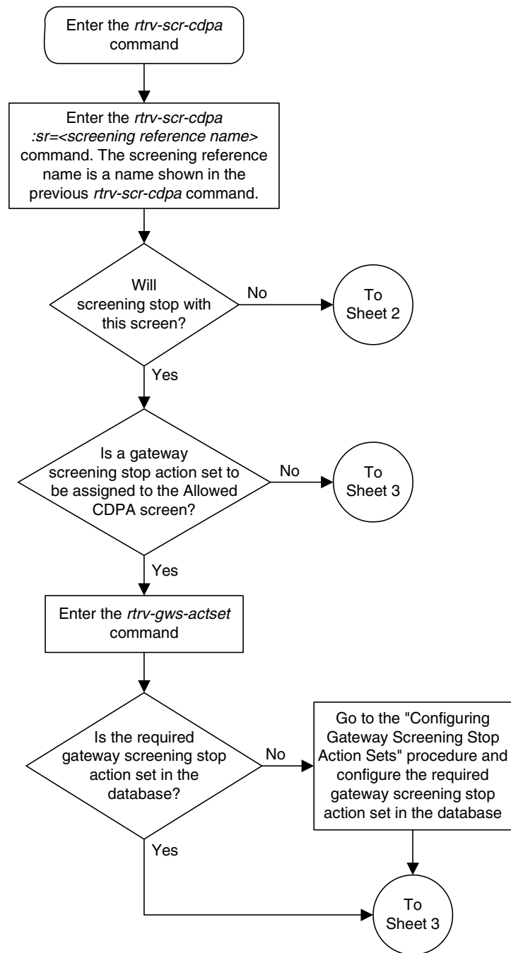
Flowchart 4-4. Changing an Allowed Called Party Address Screen (Sheet 1 of 5)
