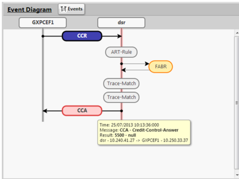
Figure 7: Event Diagram
