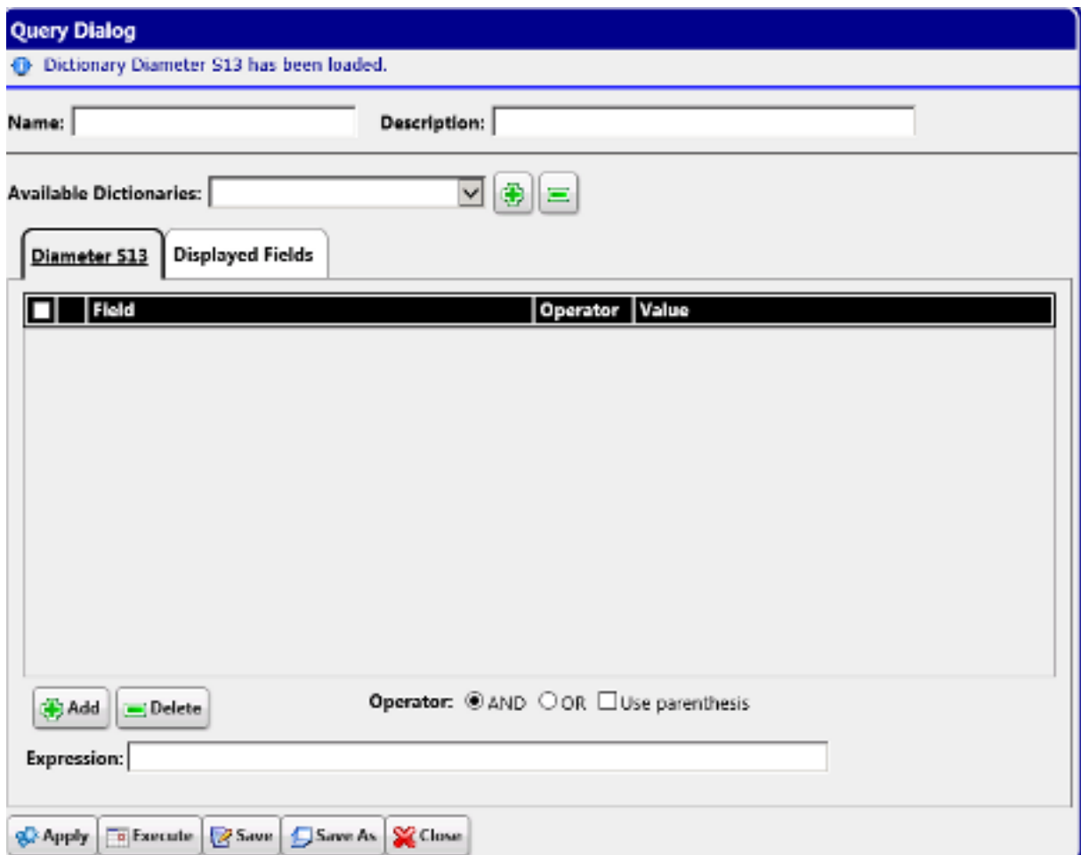
Figure 4: Query Dialog
