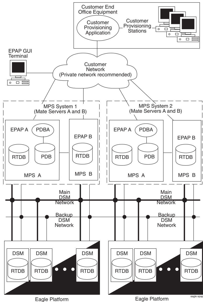
Figure 6-1. MPS on Tekelec 1000/EAGLE Overview
