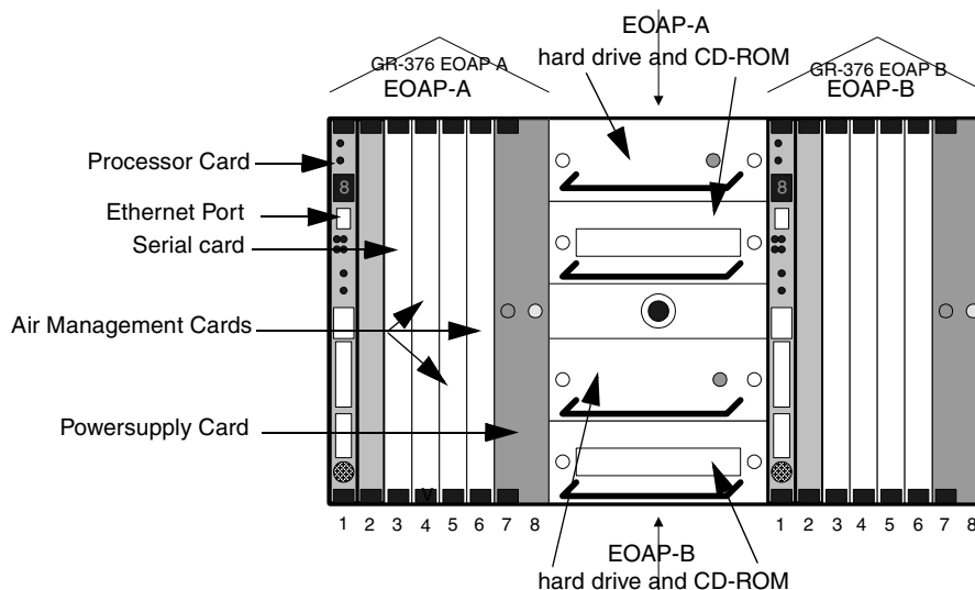
Figure 8-2. EOAP Shelf
