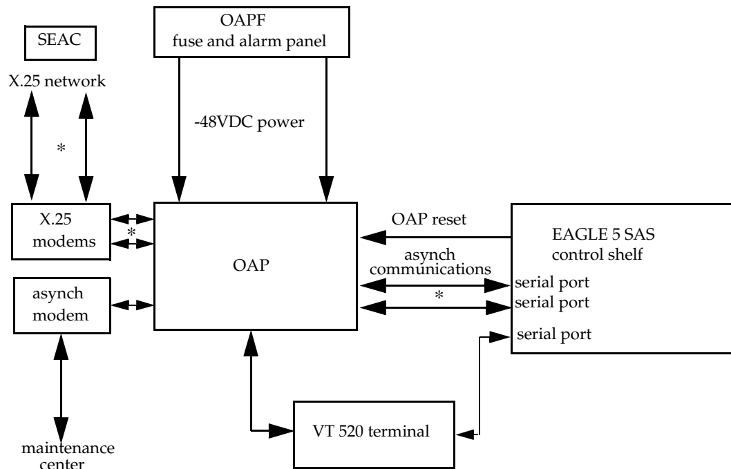
Figure 3-5. SEAS Subsystem
