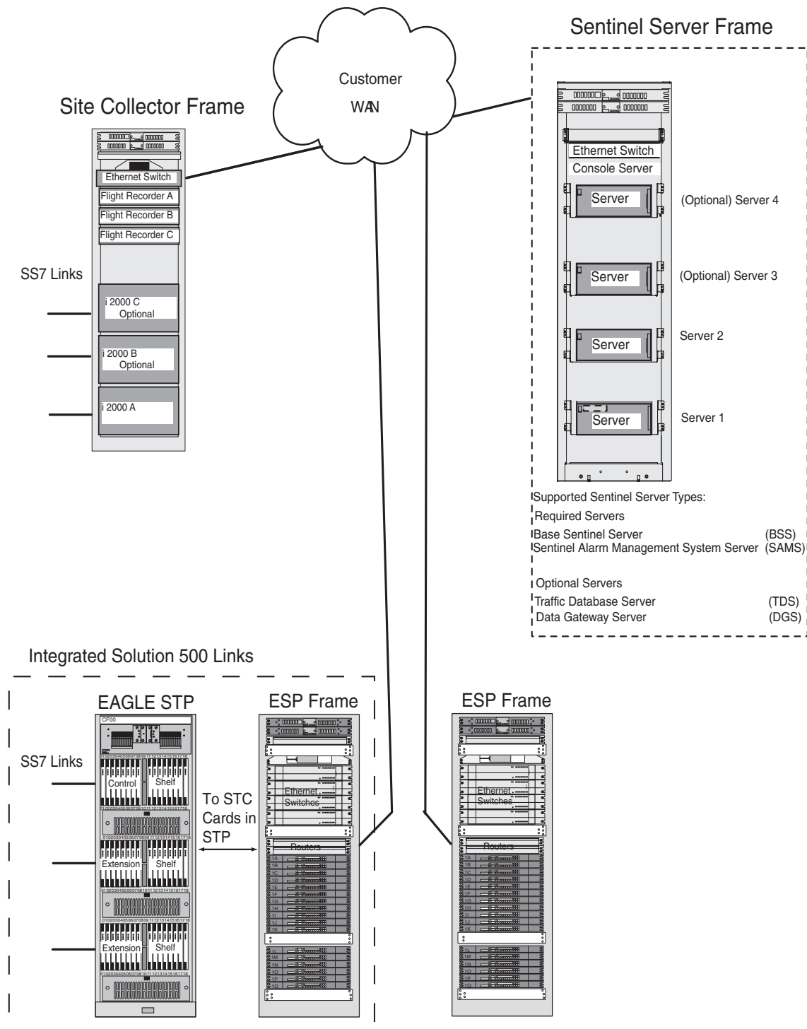
Figure 5-2. Sentinel Components
