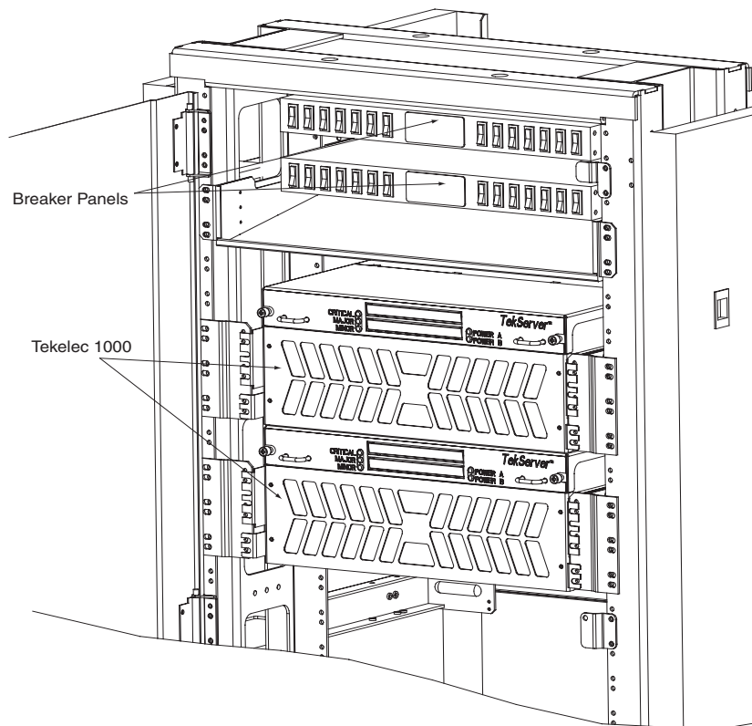
Figure 7-1. Tekelec 1000 in Tekelec Heavy-Duty Frame
