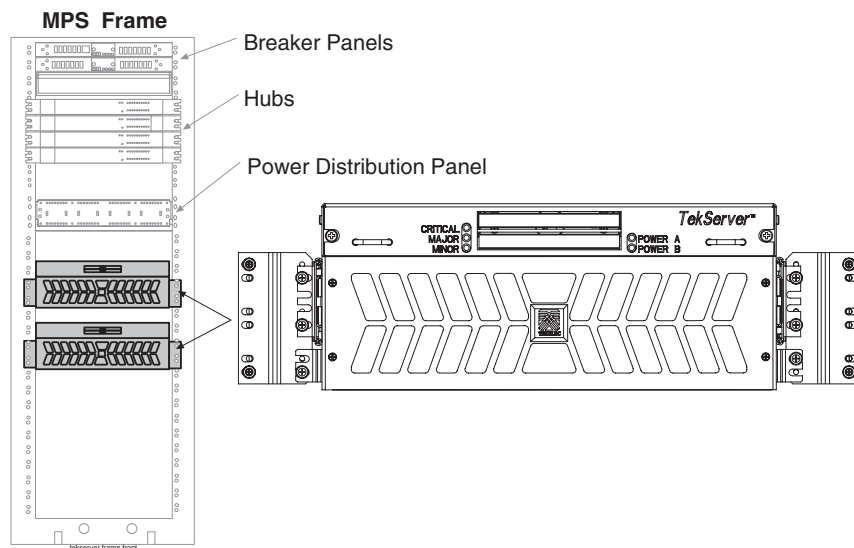
Figure 6-2. Rear View of Tekelec 1000
