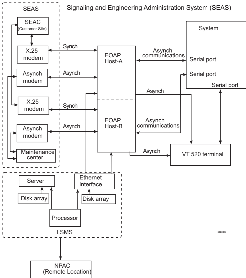
Figure 8-1. EOAP Communication
