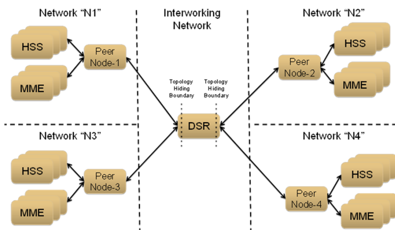
Figure 5: TH Network Deployment with DSR in an Interworking Network
