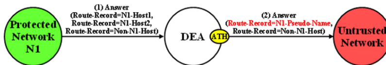
Figure 11: Route-Record Hiding - Answer Message
