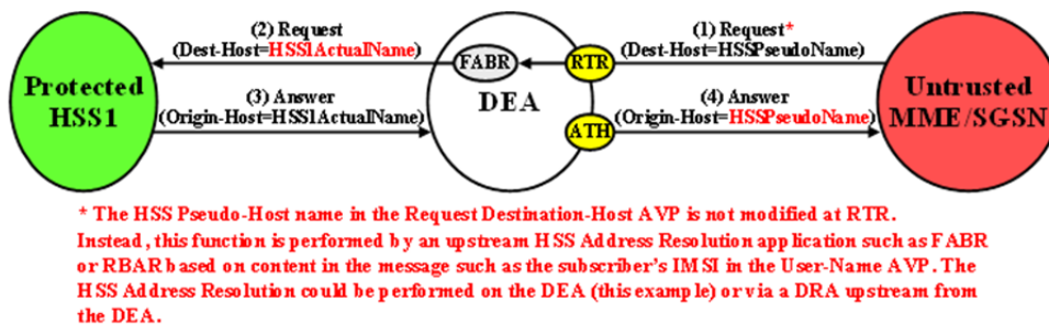
Figure 7: S6a/S6d HSS TH Untrusted-MME/SGSN to Protected-HSS Transaction
