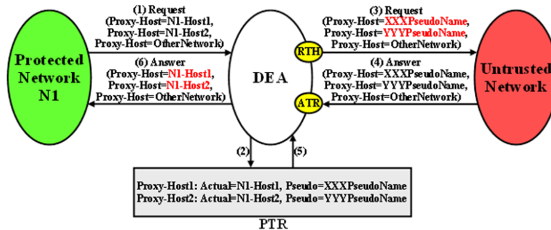
Figure 14: Proxy-Host Hiding
