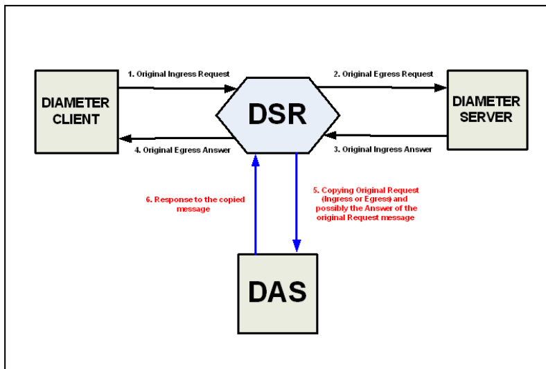
Figure 16: Diameter Message Copy Message Flow
