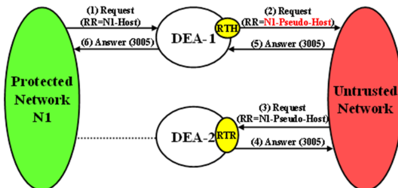
Figure 12: Multi-DEA Route-Record Message Loop Detection
