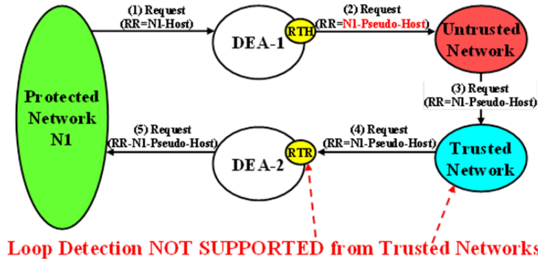
Figure 13: Unsupported Pseudo-Host Route-Record Loop Detection
