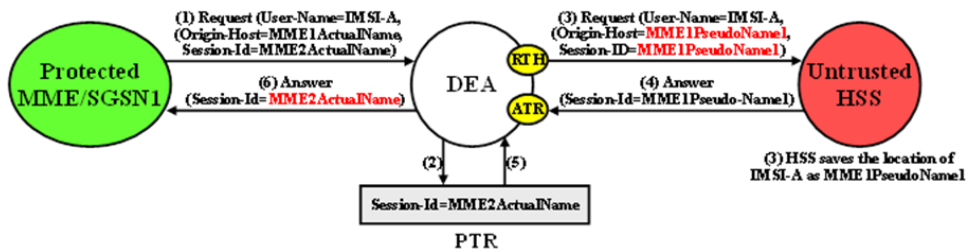
Figure 8: MME/SGSN TH Protected-MME/SGSN to Untrusted HSS Transaction
