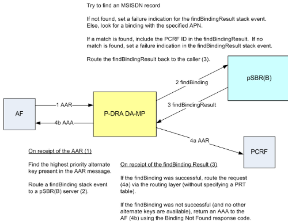
Figure 13: Binding Dependent Session Initiation Request Processing Overview
