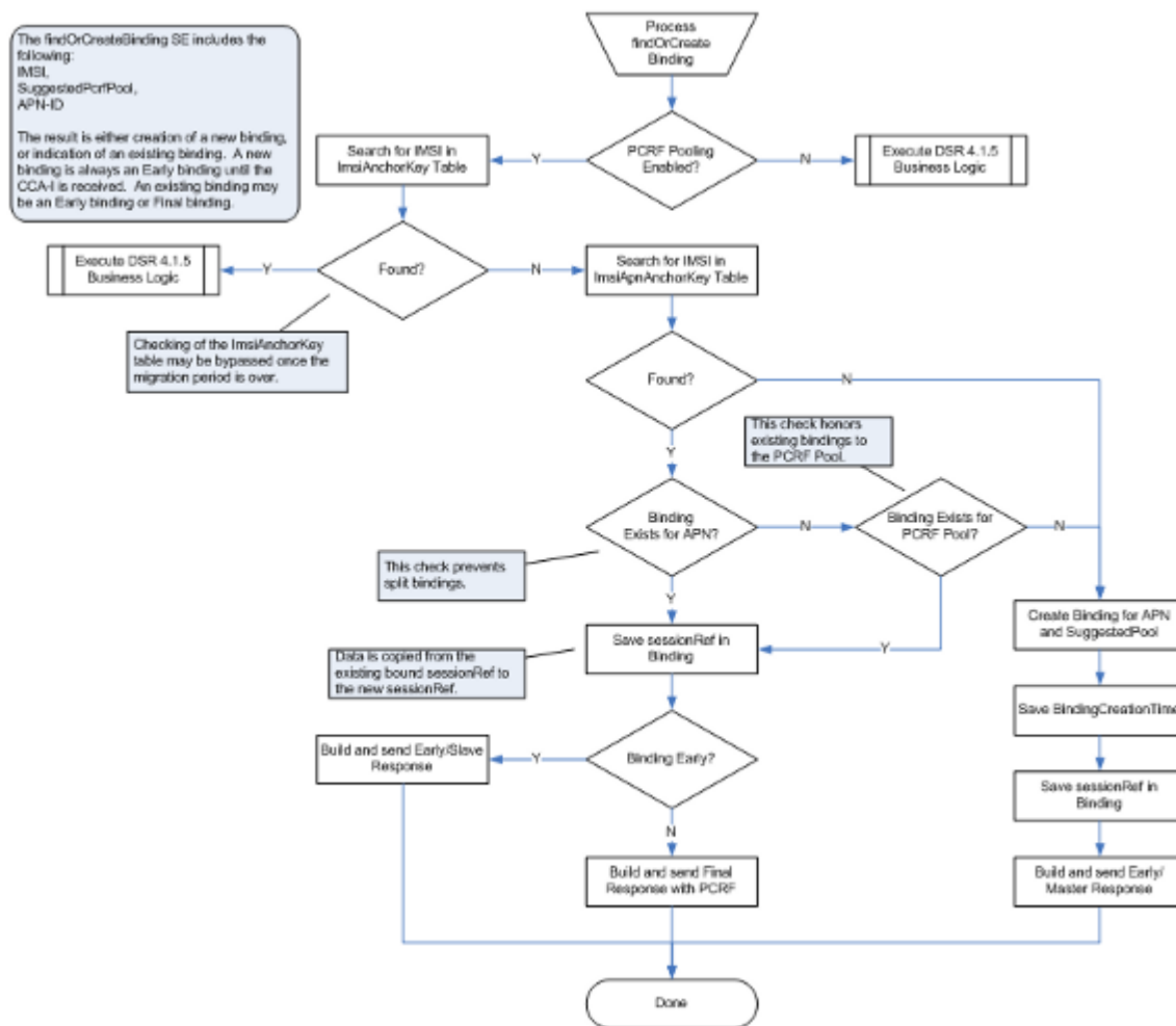
Figure 12: Find or Create a Binding
