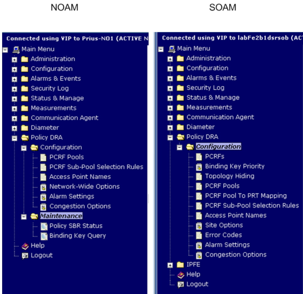
Figure 26: GUI Structure for 3-tiered DSR Topology with Policy DRA
