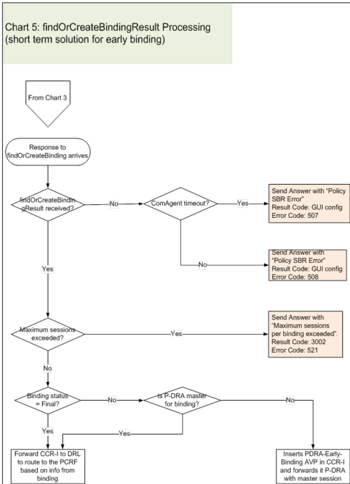
Figure 35: findOrCreBindResShort Processing Error Resolution Flowchart
