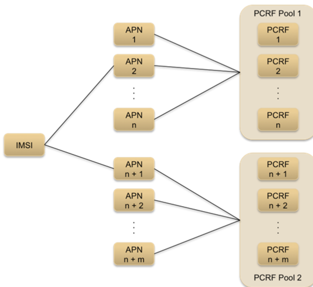
Figure 8: Relationship between IMSIs and PCRF Pools
