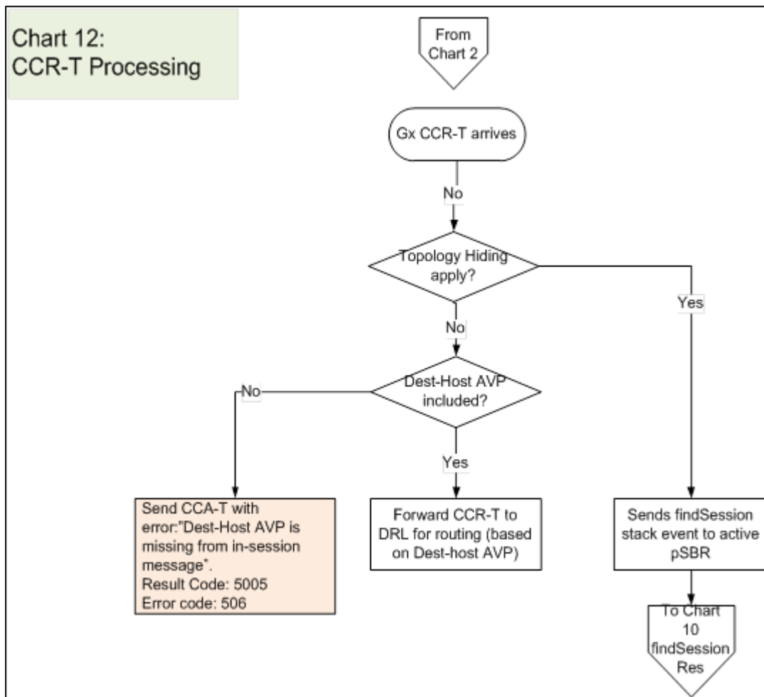
Figure 42: CCR-T Processing Error Resolution Flowchart
