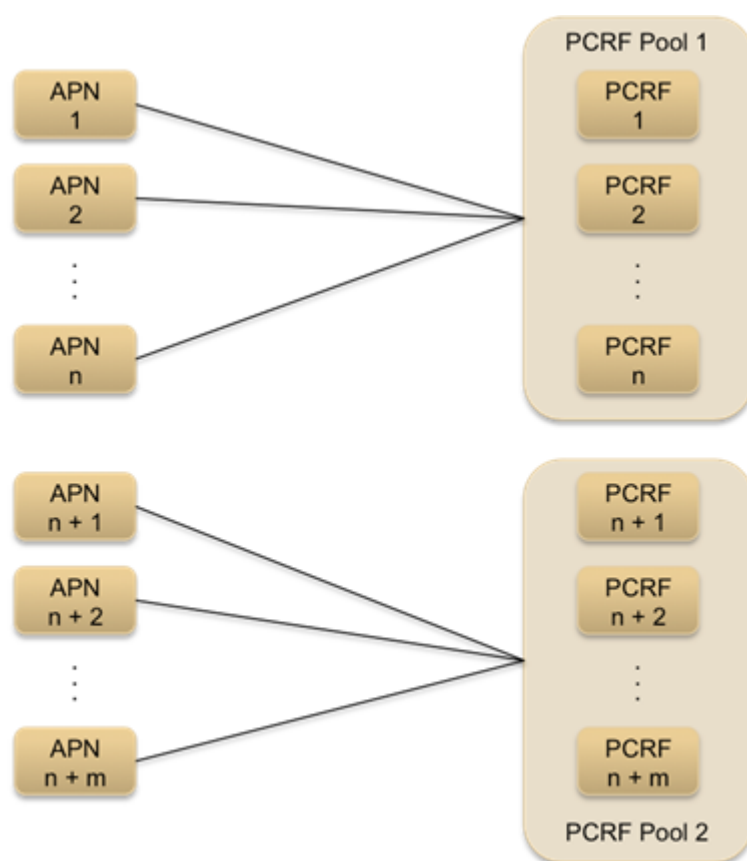
Figure 7: Relationship between APNs and PCRF Pools
