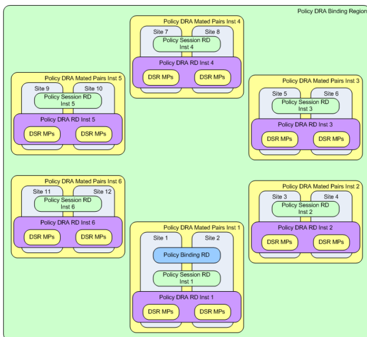
Figure 14: Sites, Mated Pairs, and Region
