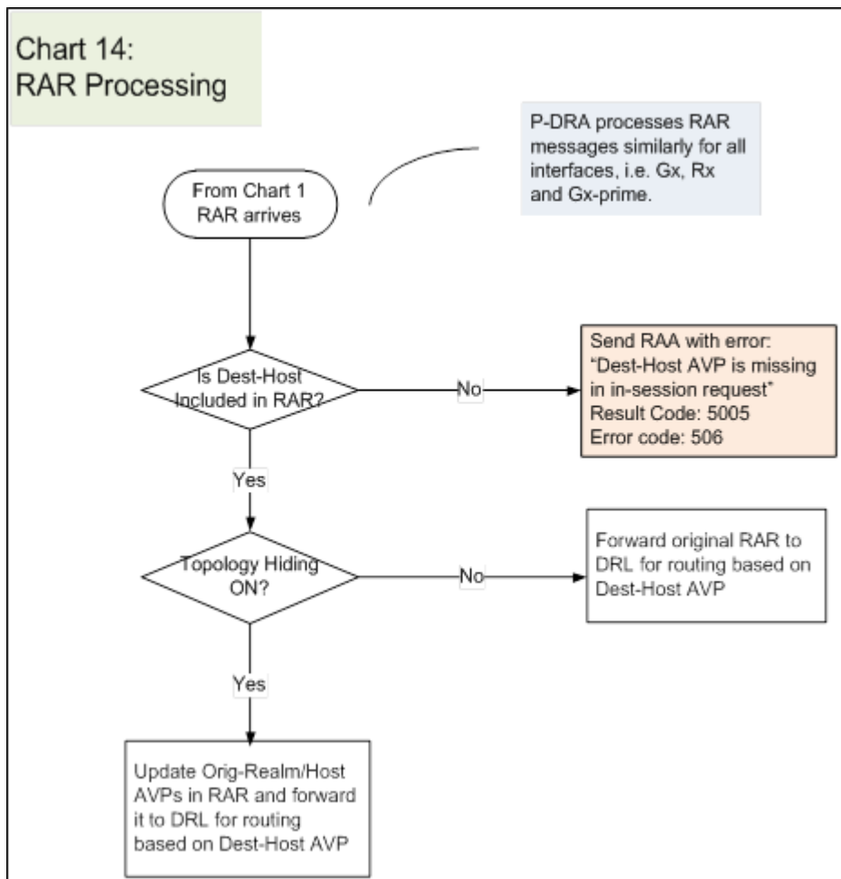
Figure 44: RAR Processing Error Resolution Flowchart
