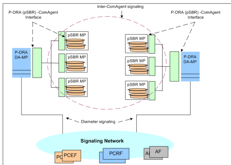
Figure 1: Communication between ComAgents, Policy DRA, and Policy SBR
