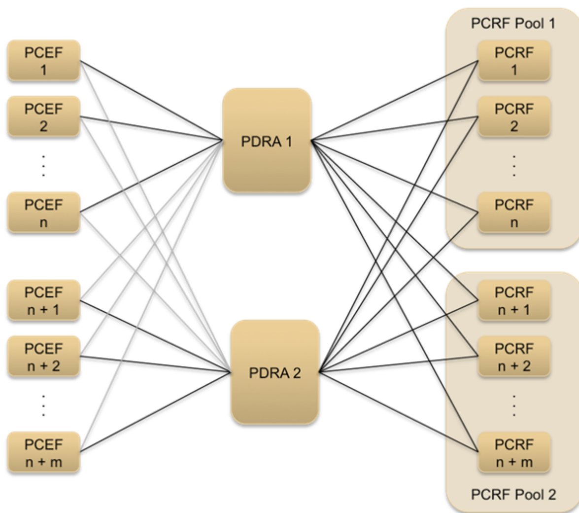
Figure 9: Multiple PCRF Pools
