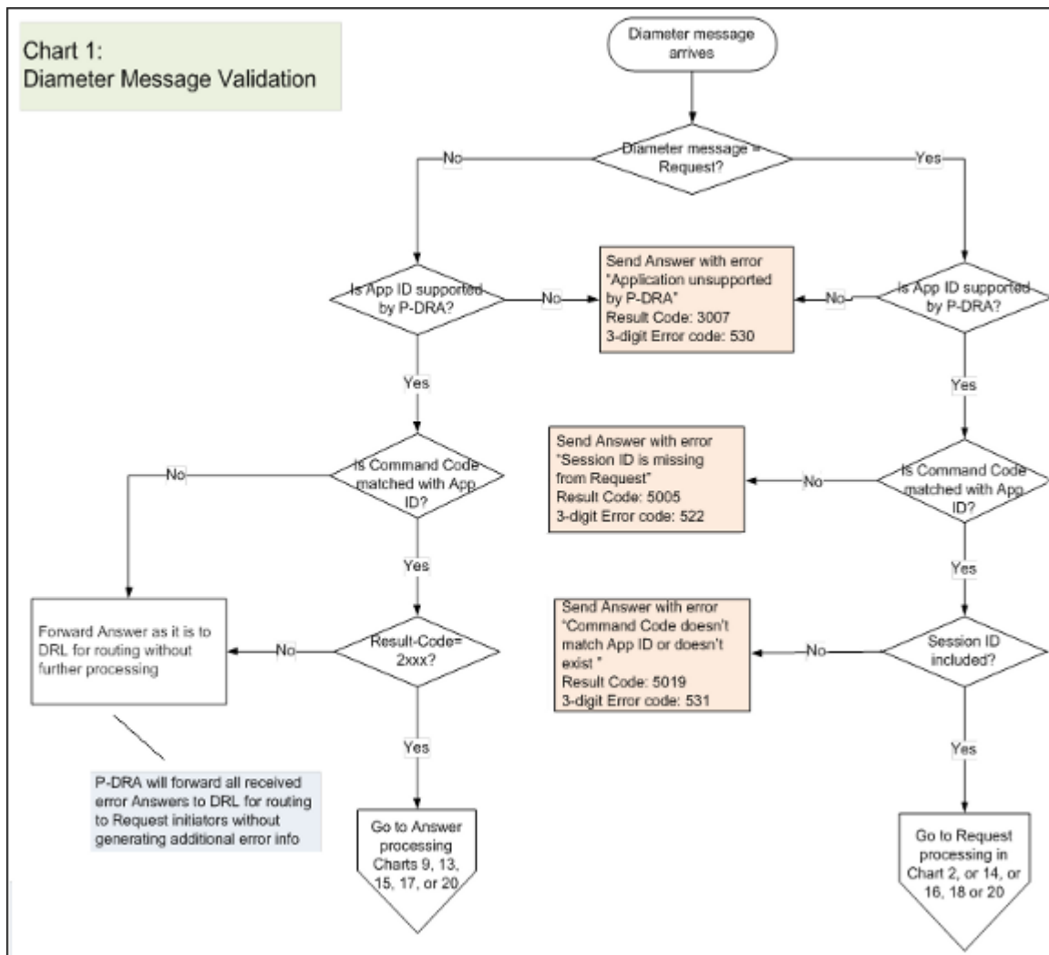
Figure 31: Diameter Message Validation Error Resolution Flowchart
