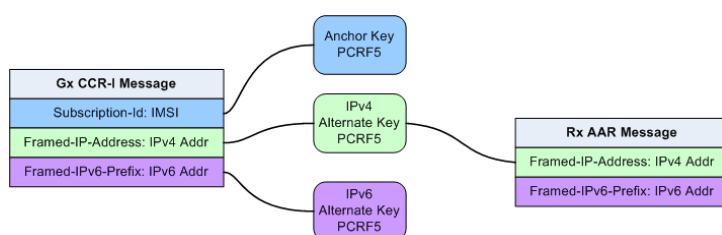
Figure 2: Subscriber Key Usage
