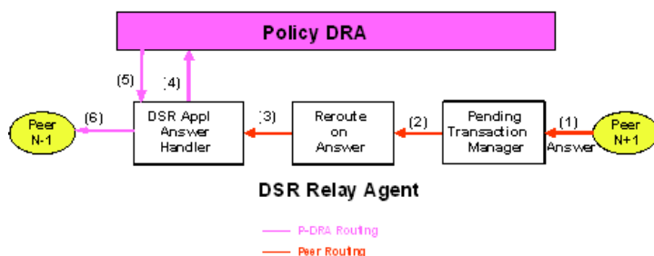
Figure 4: Answer Processing at the Diameter Routing Function and Policy DRA
