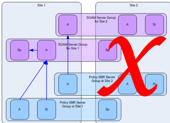
Figure 24: Data merging - Redundant Site Failure
