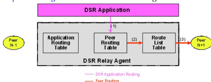
Figure 6: Policy DRA Generated Request Routing
