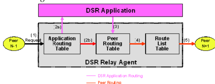
Figure 3: Request Processing at the Diameter Routing Function and Policy DRA
