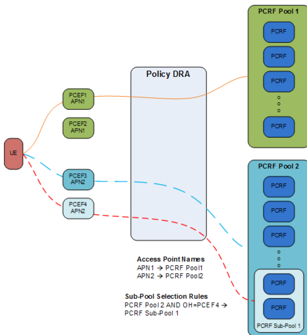
Figure 11: PCRF Pools and Sub-Pools Routing Scenarios
