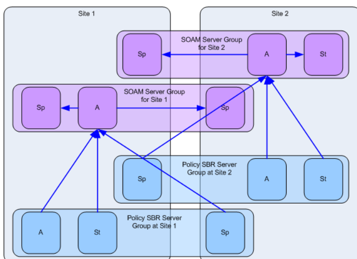
Figure 23: Data Merging - Normal Case
