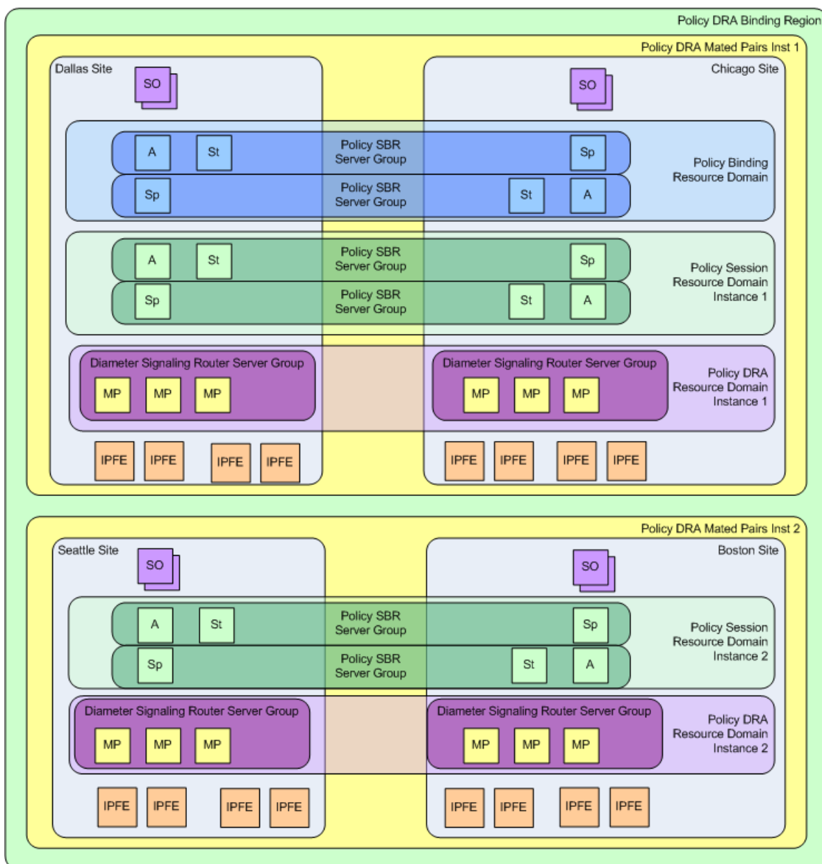
Figure 16: Policy DRA Component Relationships
