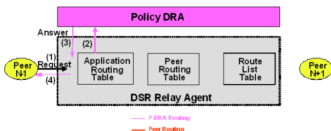
Figure 5: Policy DRA Generated Answer Routing
