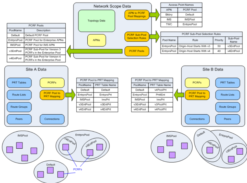
Figure 27: PCRf Pooling Data
