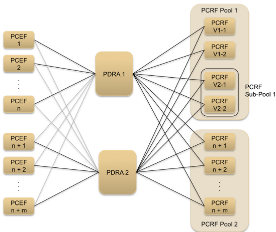
Figure 10: Multiple PCRF Versions in a PCRF Pool
