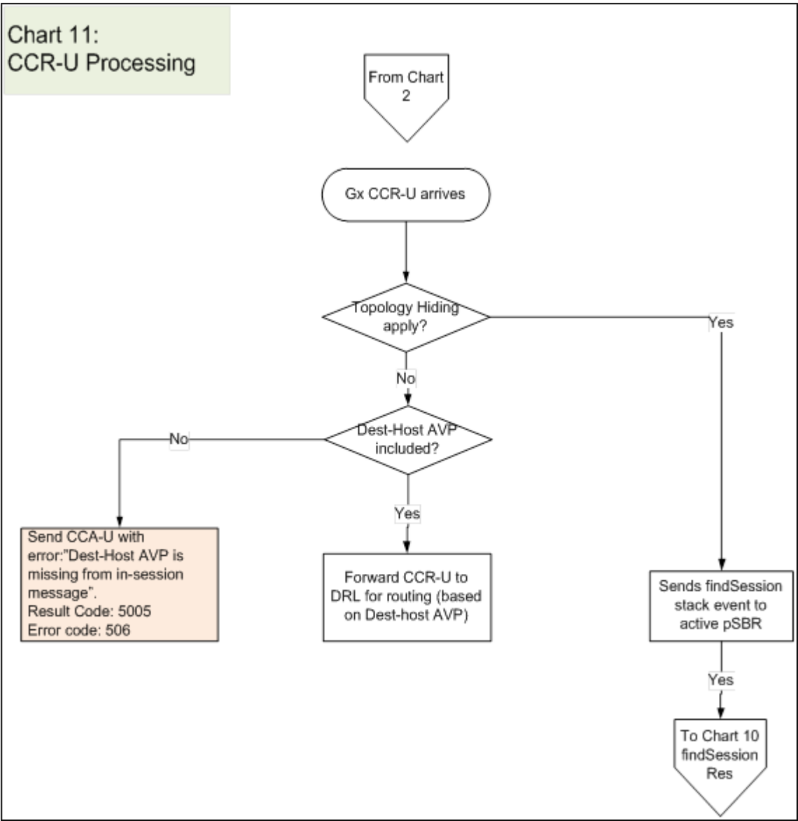
Figure 41: CCR-U Processing Error Resolution Flowchart
