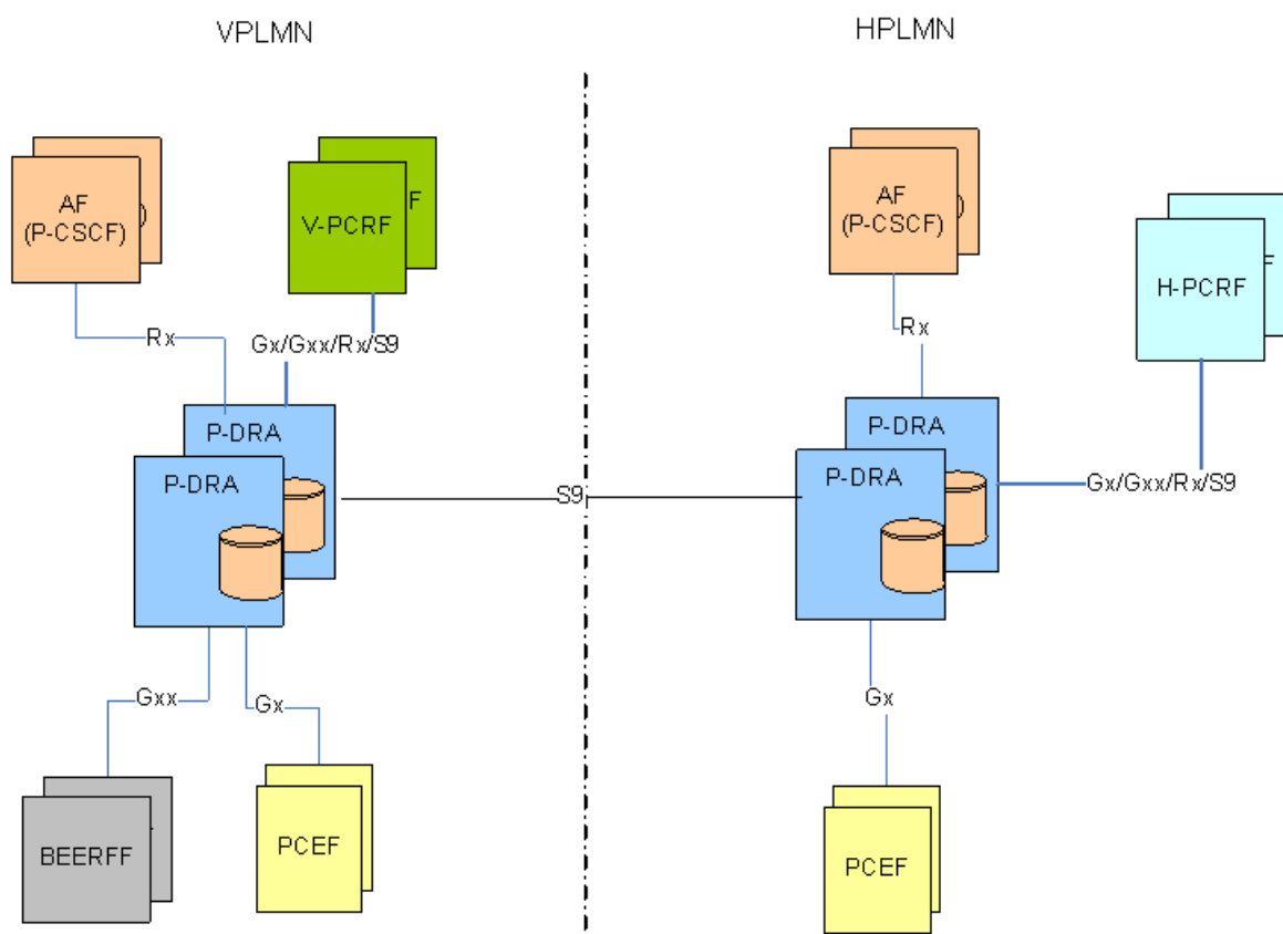
Figure 15: Policy DRA in Roaming Scenarios
