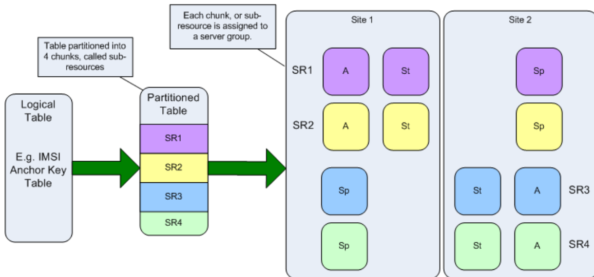
Figure 21: Binding Table Partitioning Across Server Groups
