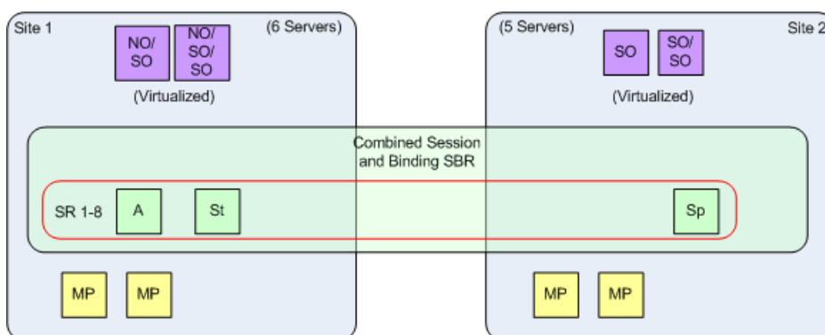
Figure 25: Smallest Supported Policy DRA Mated Pair
