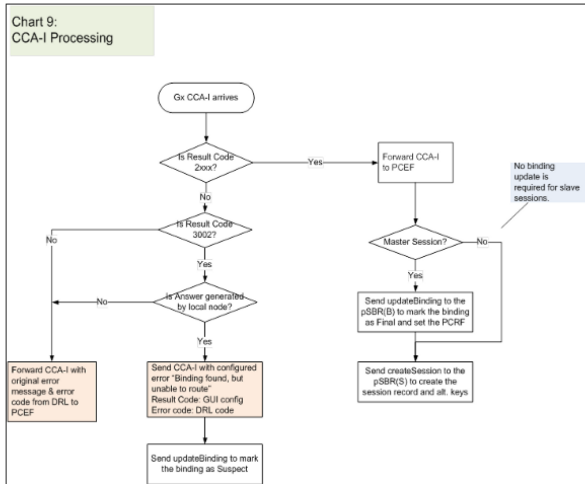
Figure 39: CCA-I Processing Error Resolution Flowchart
