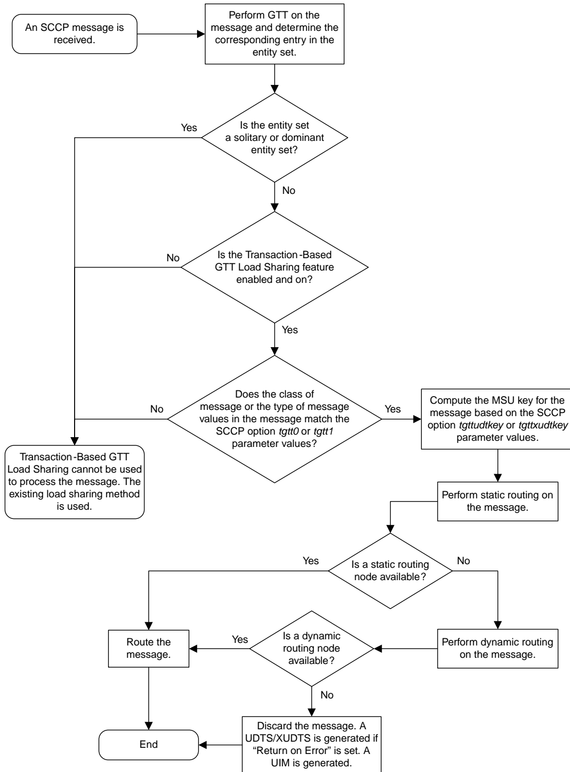
Figure 5: Message Routing using Transaction-Based GTT Load Sharing
