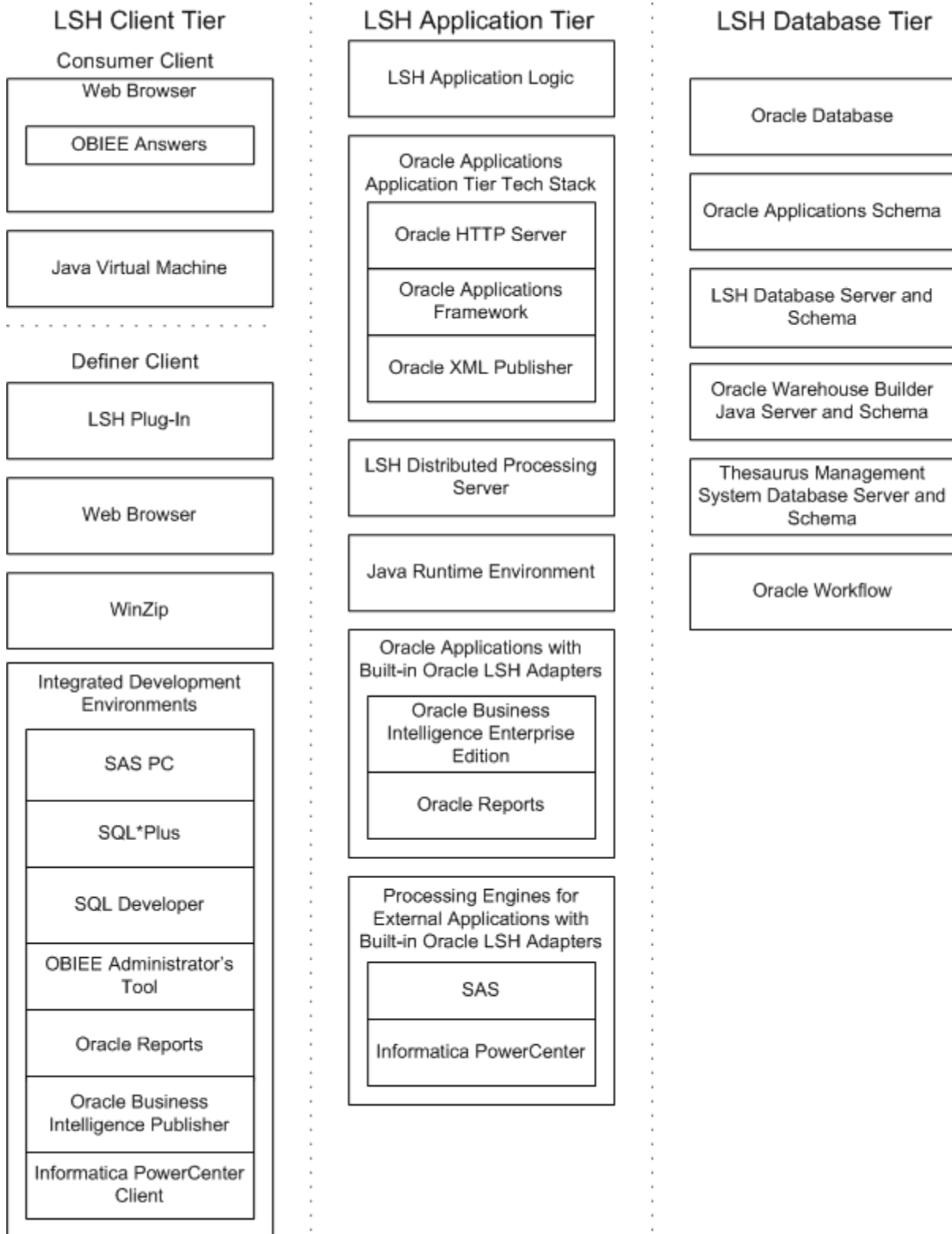
Figure A-1 Oracle LSH Architecture
