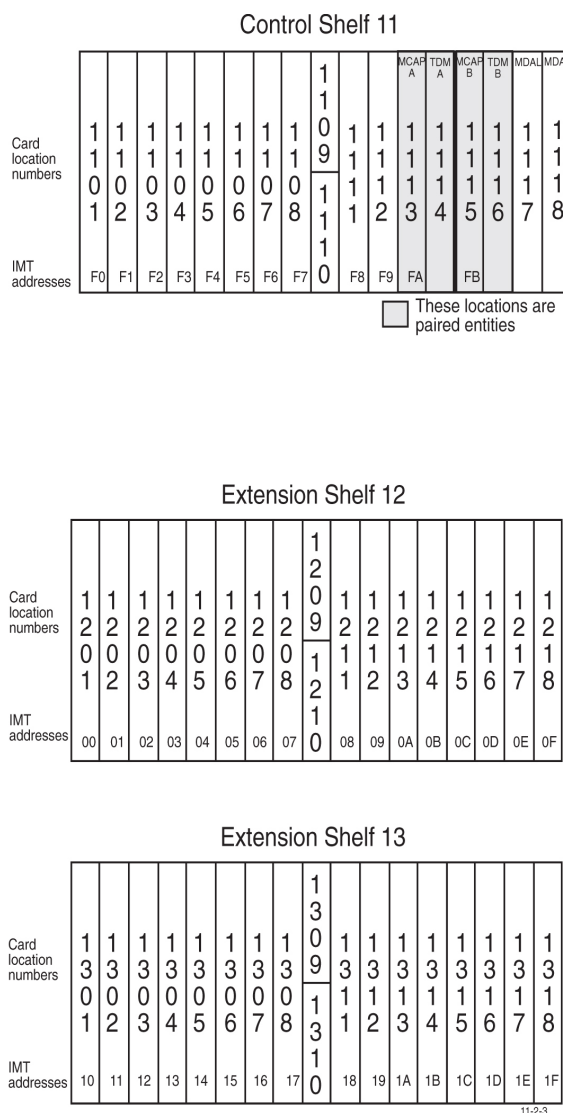
Figure 13: Control Frame CF-00 Numbering Plan
