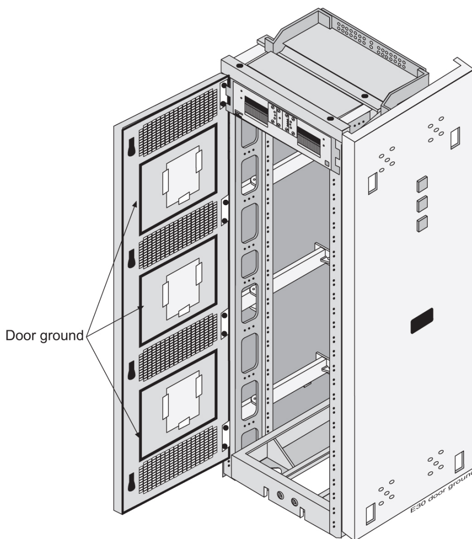
Figure 85: Door Grounding
