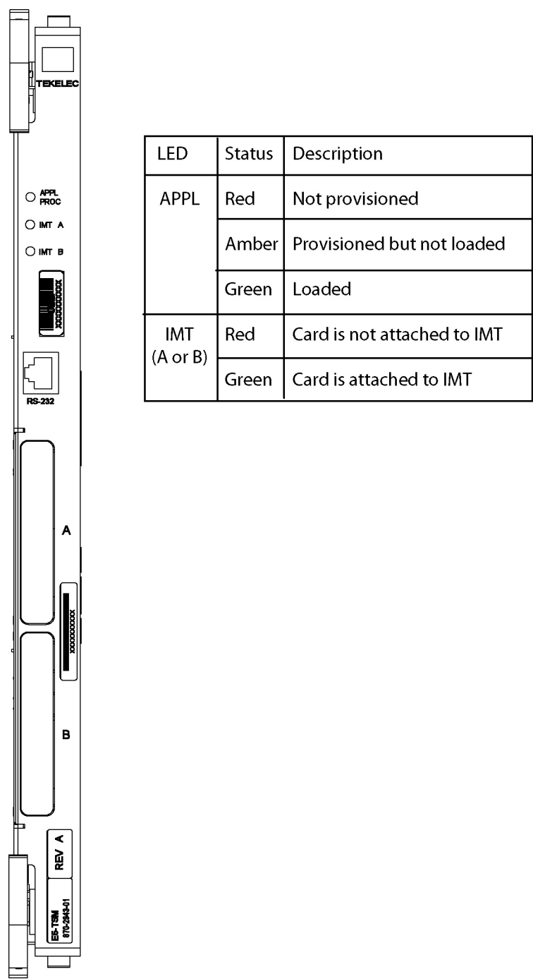
Figure 59: E5-TSM LEDs
