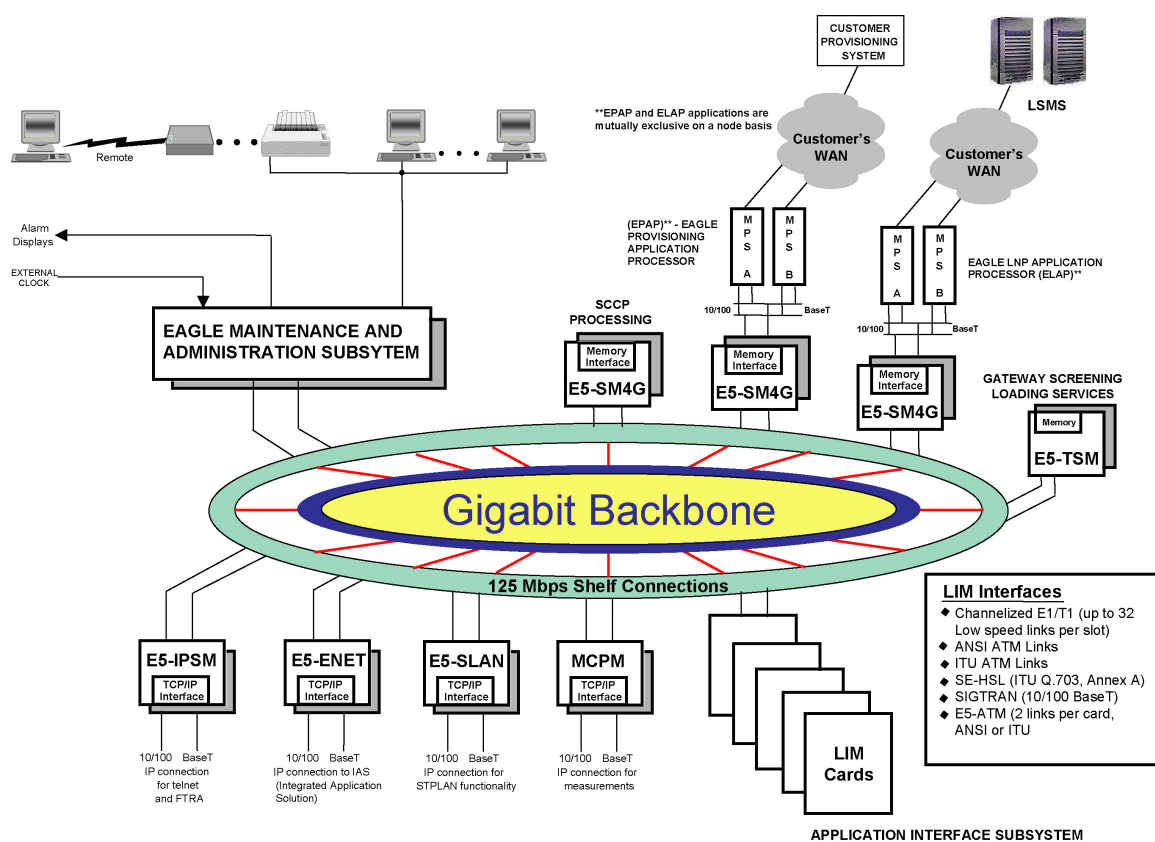
Figure 4: EAGLE 5 ISS Functional Diagram
