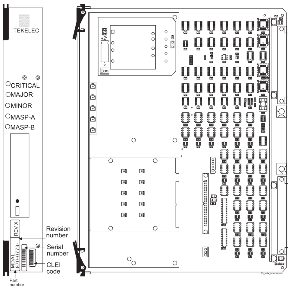
Figure 37: Maintenance Disk and Alarm Card
