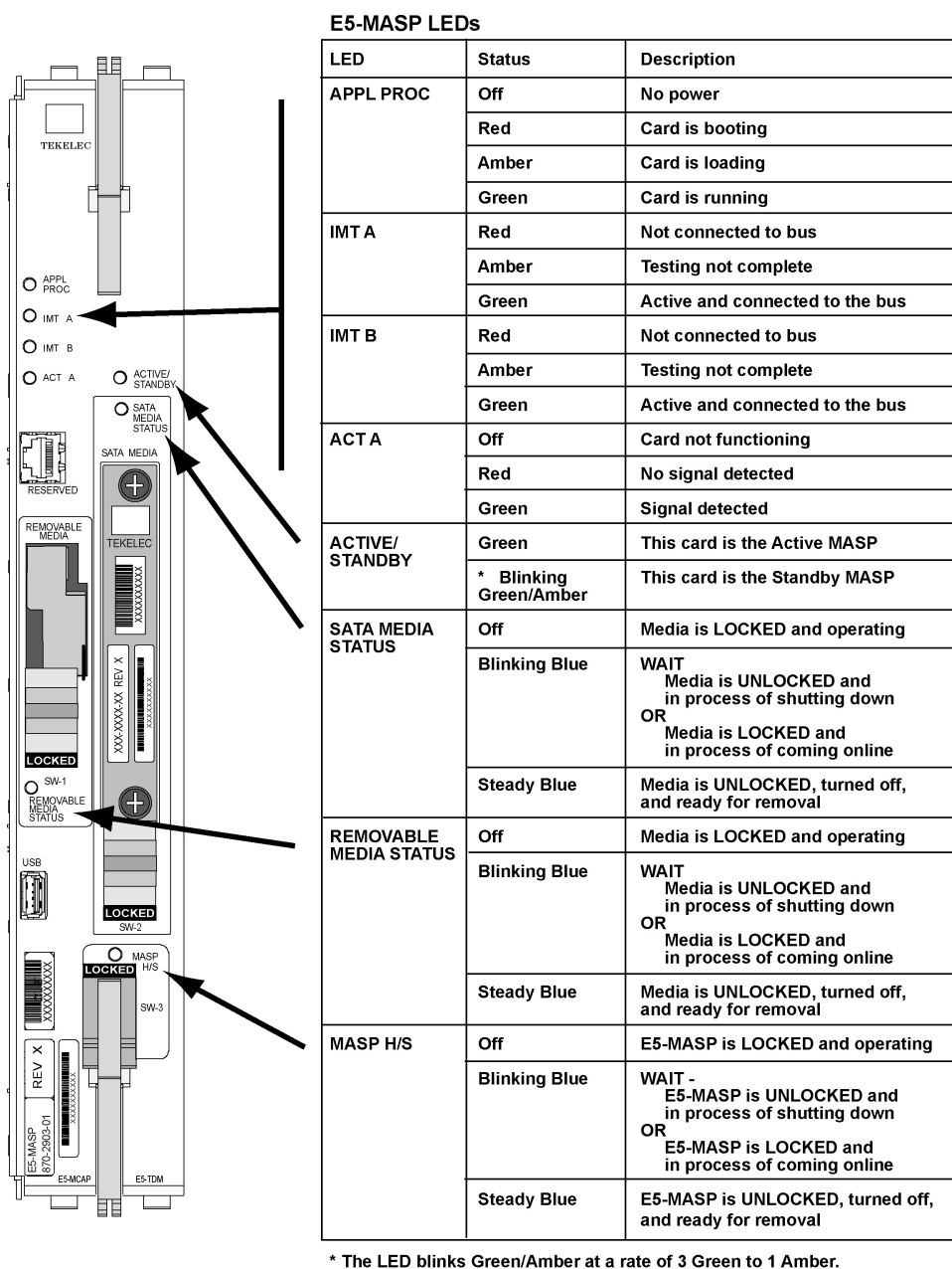
Figure 35: E5-MASP LEDs
