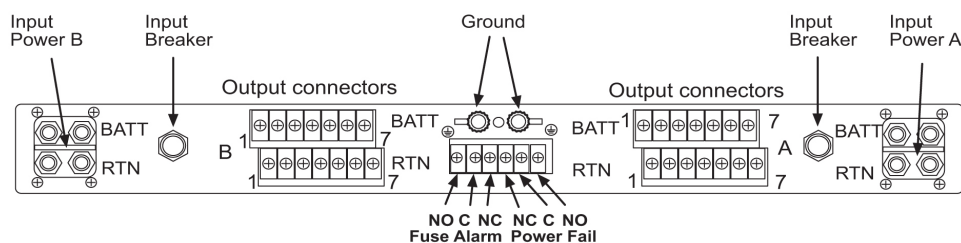
Figure 80: Telect Breaker Panel Rear View
