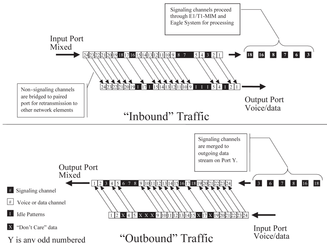
Figure 54: Channel Bridging Schematic
