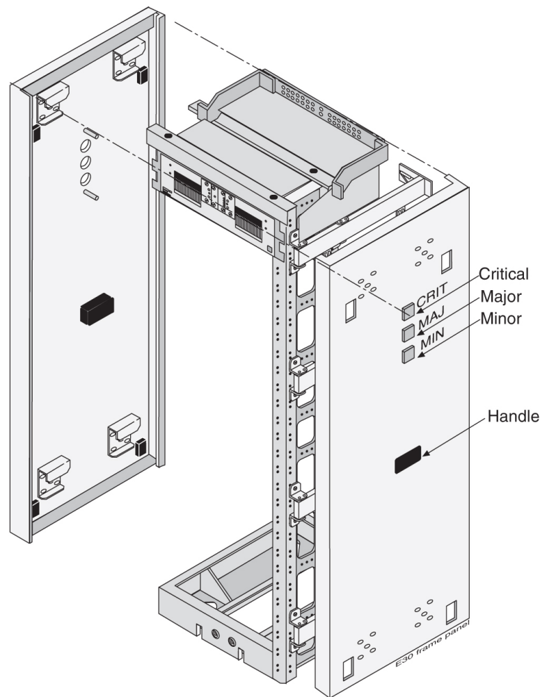
Figure 12: Frame End Panel with Lamp Indicators
