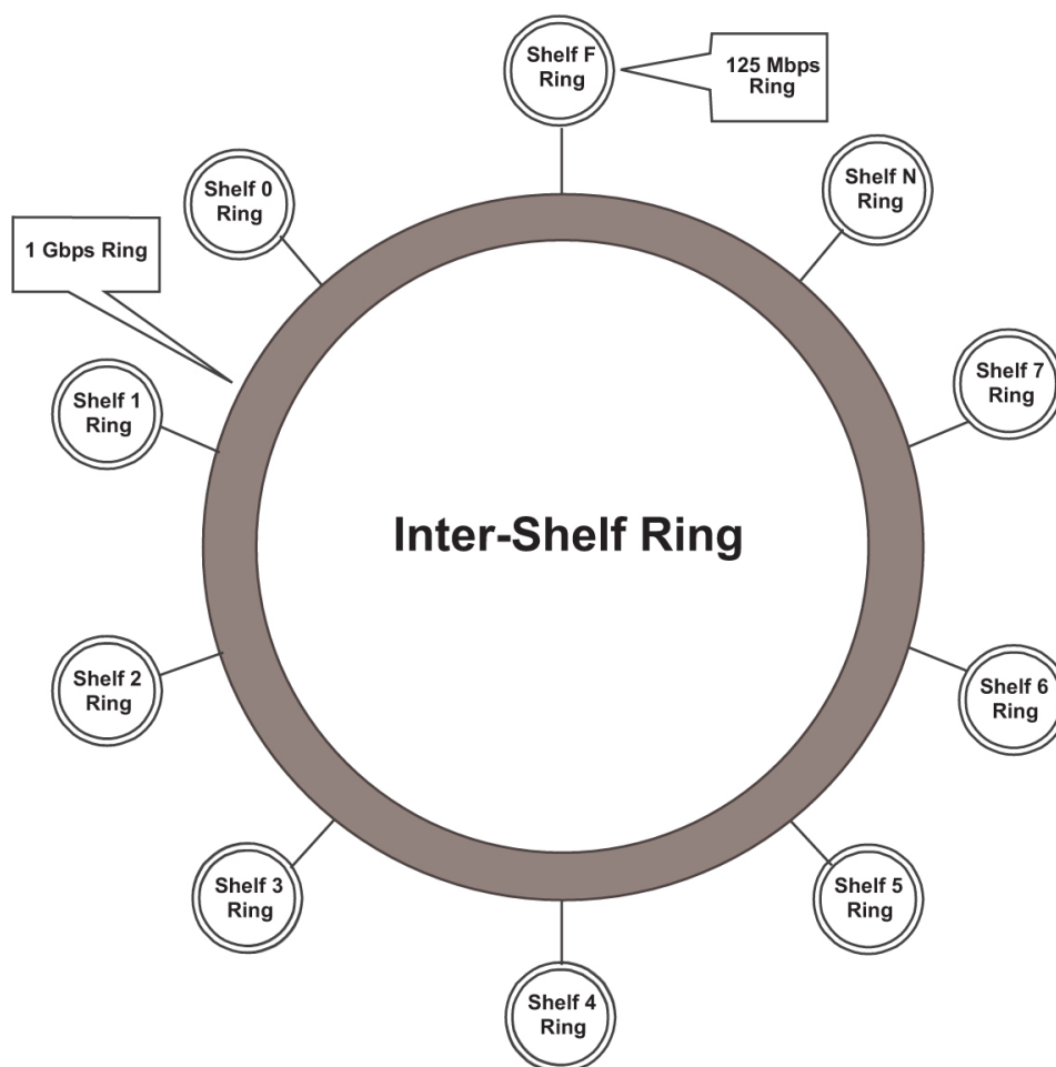
Figure 32: HMUX Ring Topology
