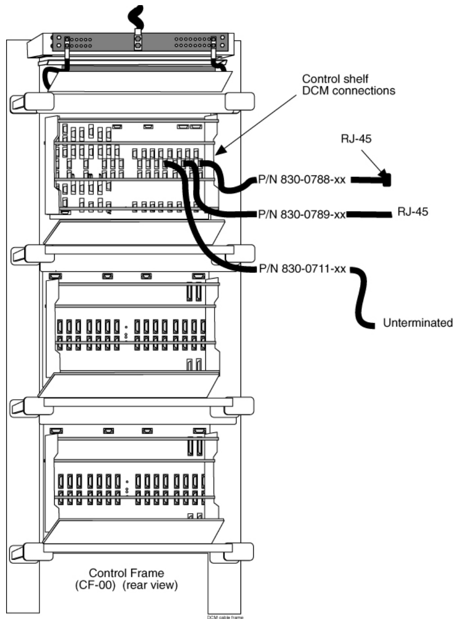
Figure 86: Database Communications Cabling in System
