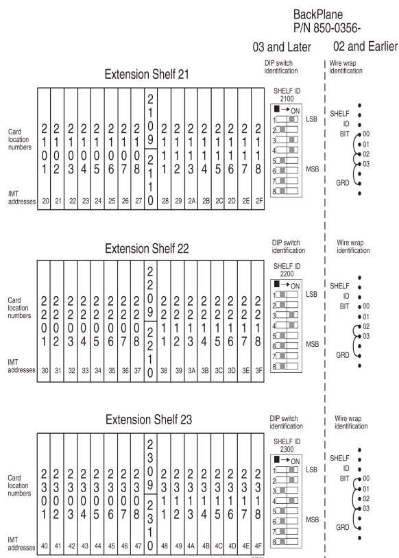
Figure 14: Extension Frame EF-00 Numbering Plan
