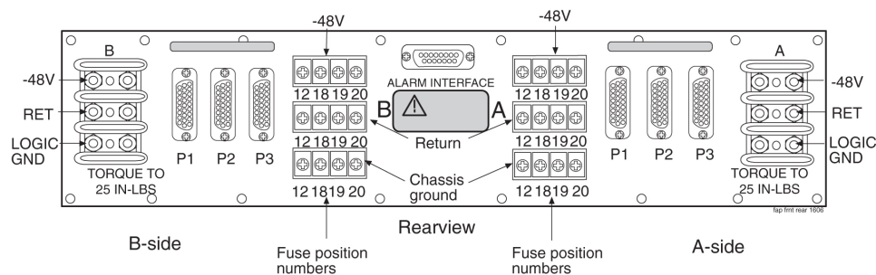
Figure 84: Logic Grounding with FAP (P/N 870-1606-xx/870-2320-xx)
