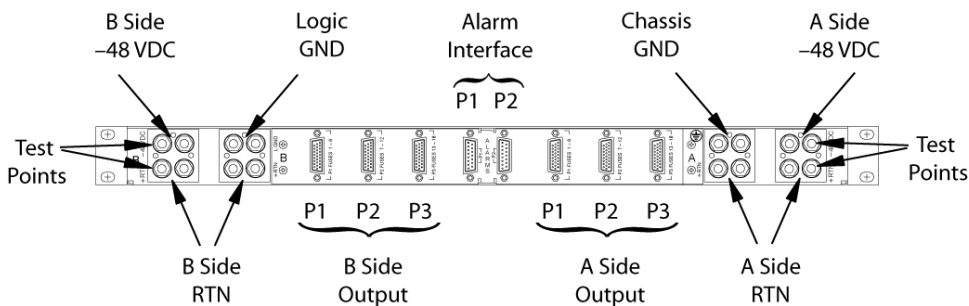
Figure 64: Fuse and Alarm Panel Rear (P/N870-2804-01).
