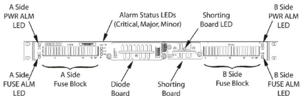
Figure 63: Fuse and Alarm Panel - Front View (P/N 870-2804-xx)
