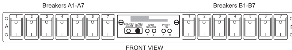
Figure 79: Telect Breaker Panel Front View
