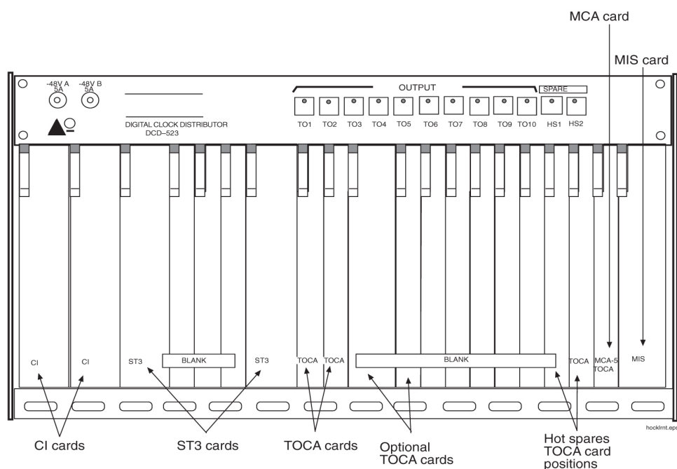
Figure 67: Holdover Clock, Card Location
