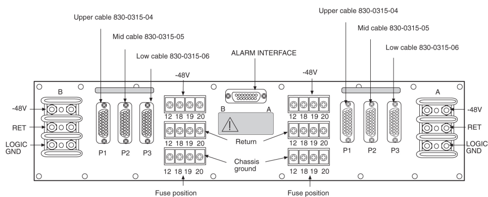
Figure 66: Fuse and Alarm Panel (P/N 870-1606-xx/870-2320-xx) Rear
