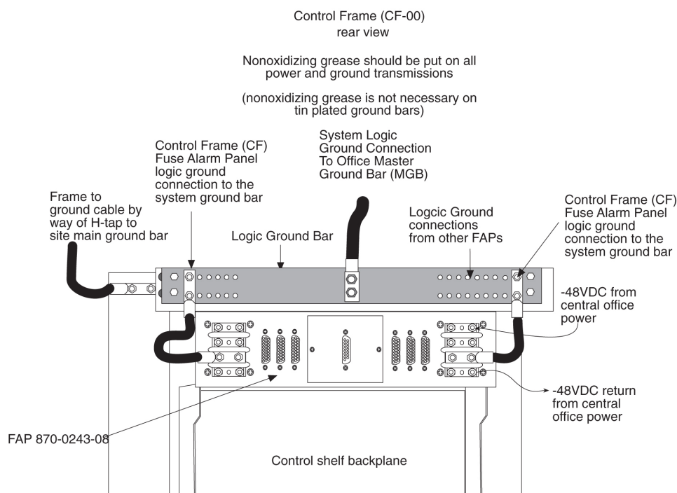
Figure 83: Logic Grounding with FAP (P/N 870-0243-08)
