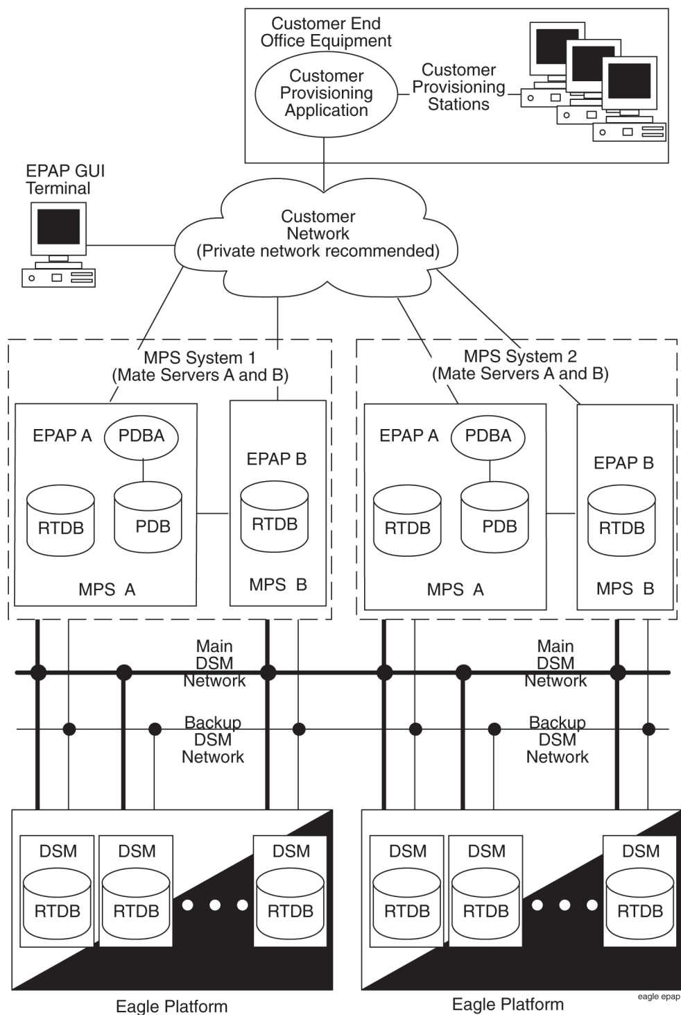
Figure 8: MPS on T1000 AS/EAGLE 5 ISS Overview
