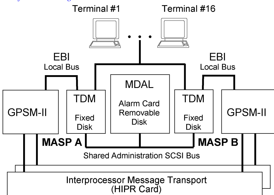
Figure 6: Legacy Maintenance and Administration Subsystem Block Diagram
