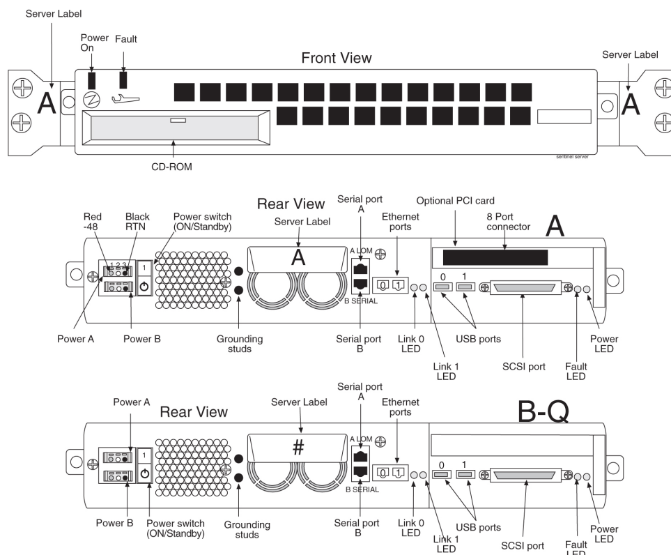
Figure 71: ESP Server Front and Rear Views
