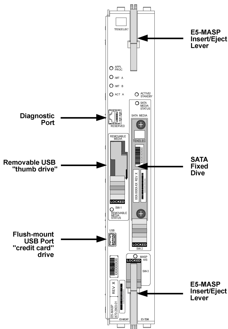
Figure 34: E5-MASP Card
