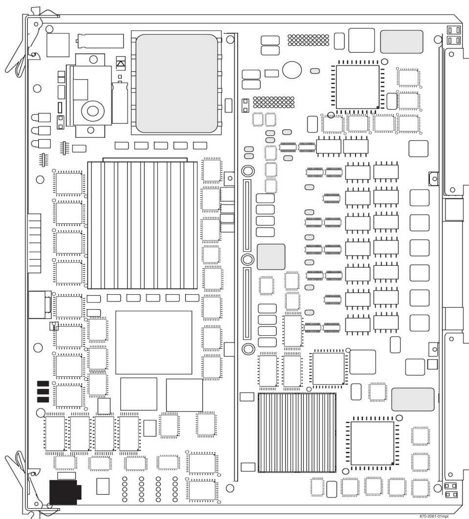
Figure 43: Multi-Port Link Interface Module (MPL) (P/N 870-2061-01)
