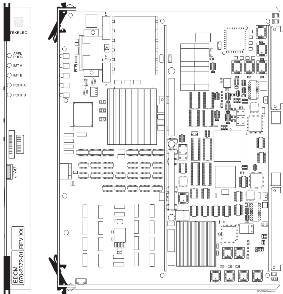
Figure 46: Single-Slot Enhanced Database Communications Module
