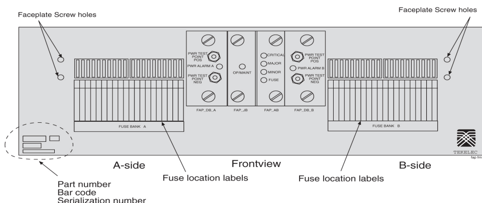
Figure 65: Fuse and Alarm Panel (P/N 870-1606-xx/870-2320-xx) Front
