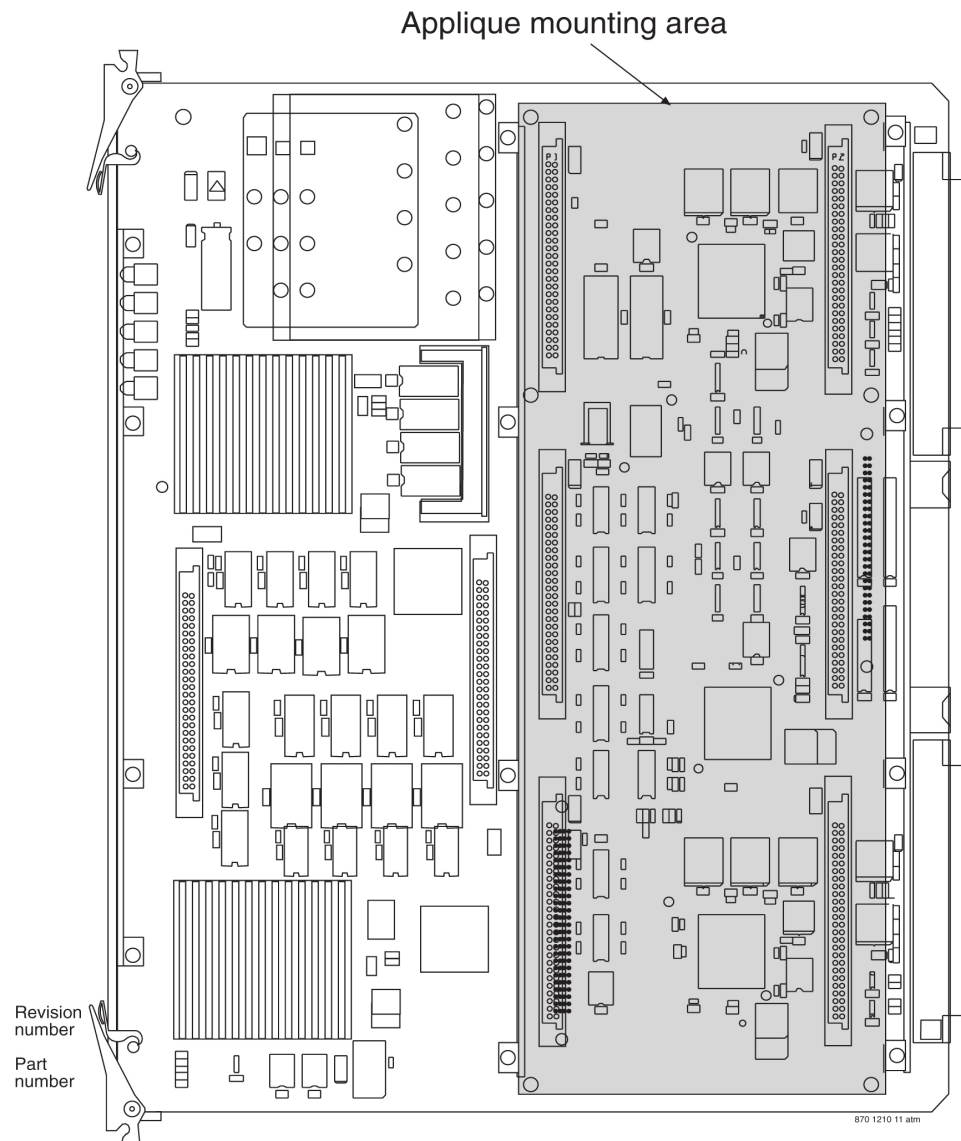
Figure 42: HCAP Main Assembly (P/N 850-0419-xx)
