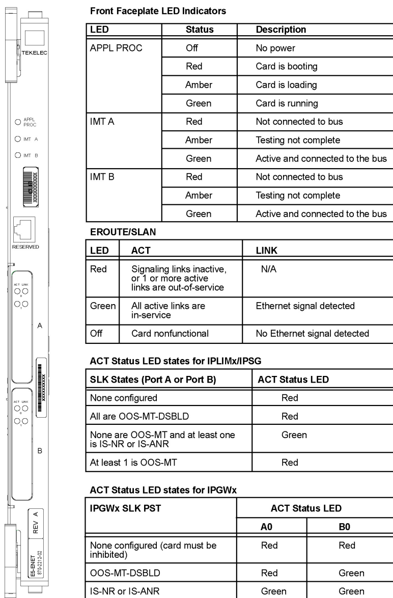
Figure 56: E5-ENET
