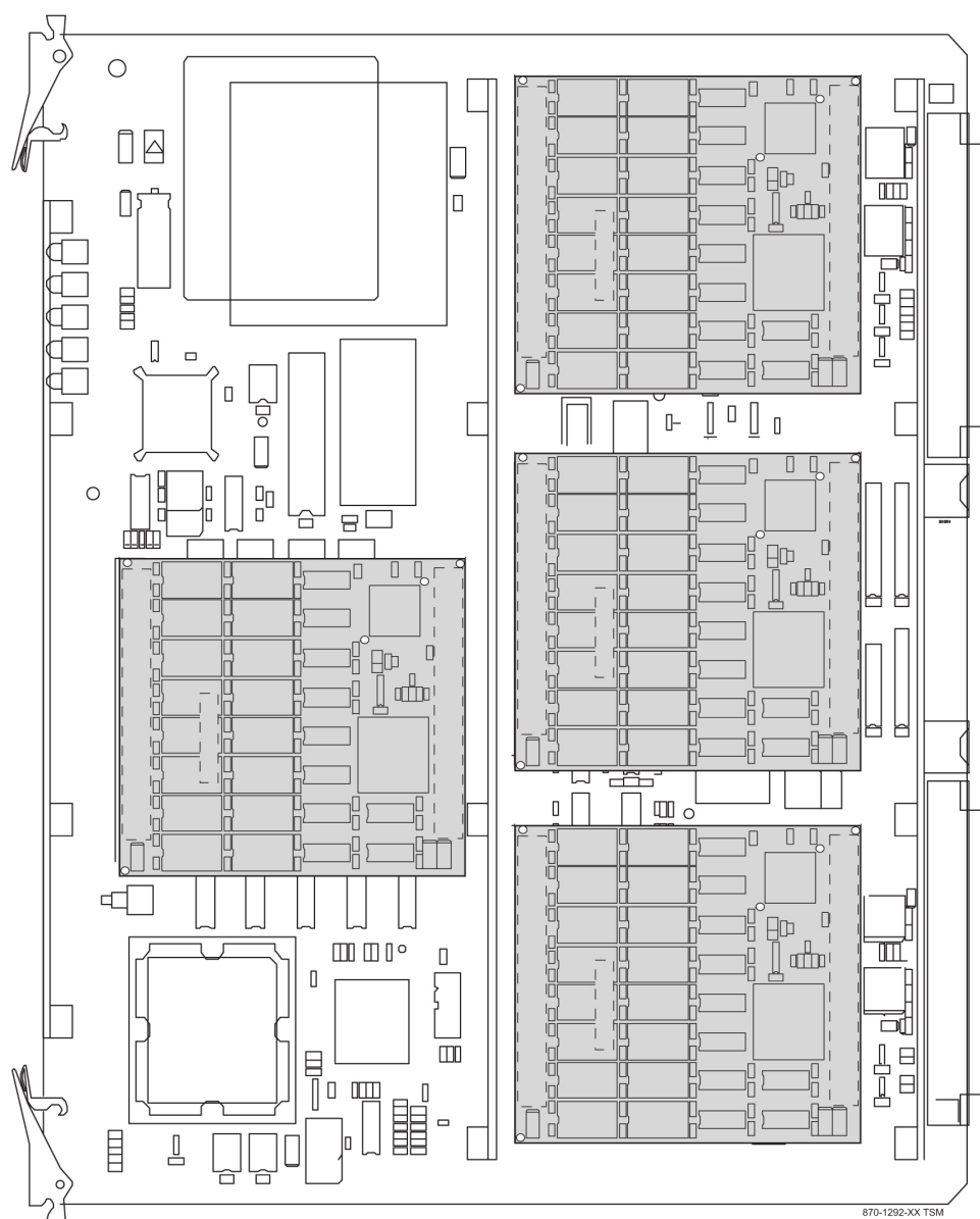
Figure 48: Translation Service Module (P/N 870-1292-xx)
