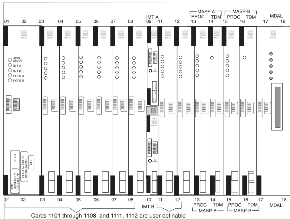
Figure 21: Control Shelf Front, with DCM Card
