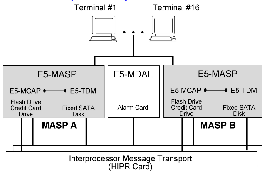
Figure 5: E5-based Maintenance and Administration Subsystem Block Diagram
