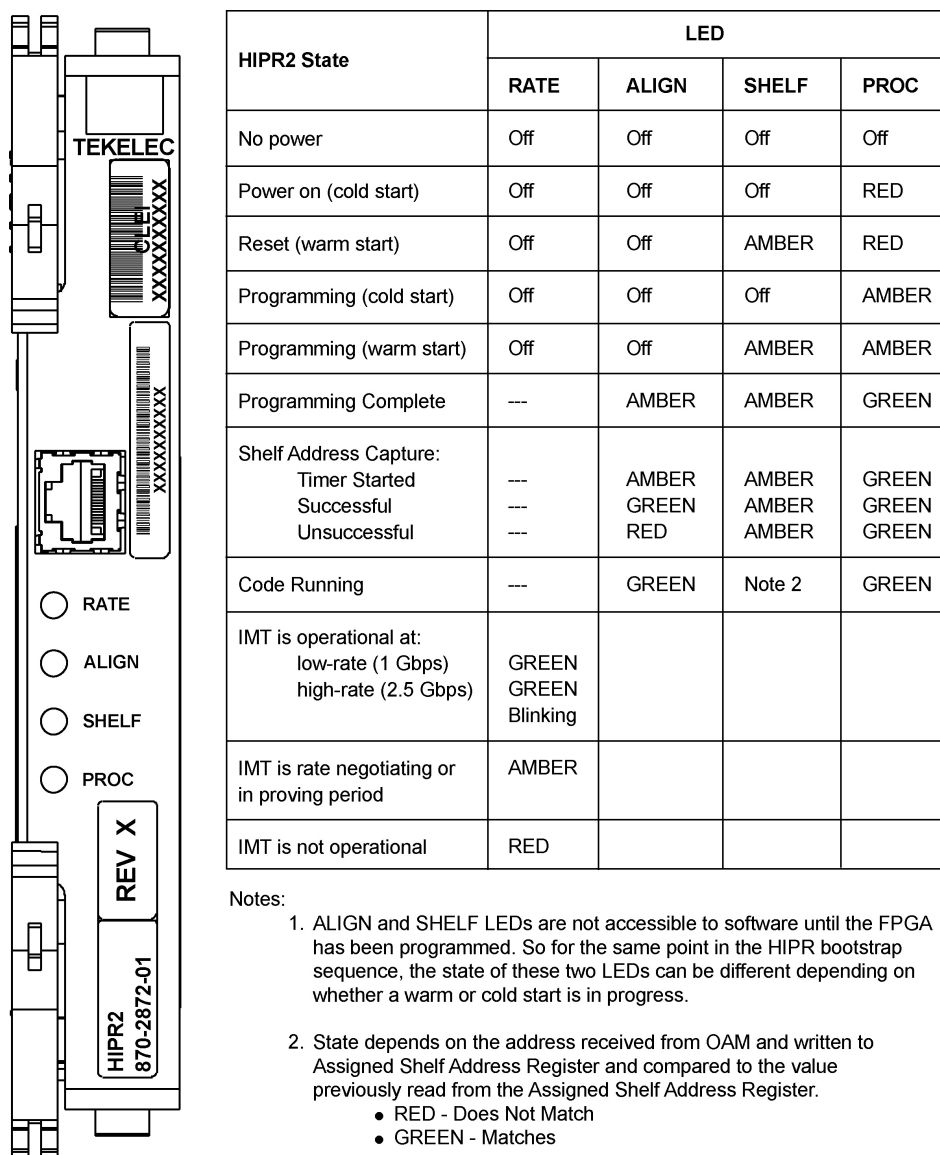
Figure 29: HIPR2 LEDs
