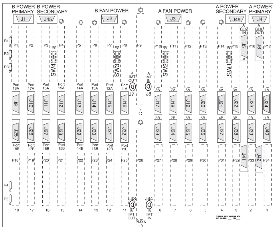
Figure 19: Extension Shelf Backplane ID (P/N 850-0356-04/06)
