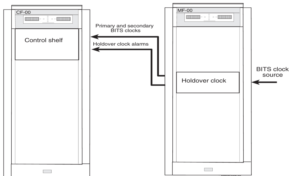
Figure 68: Holdover Clock, Frame Connections
