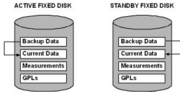
Figure 5-2. The chg-db:action=restore:src=fixed Command
