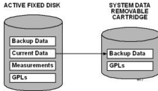
Figure 5-3. The chg-db:action=backup:dest=remove Command
