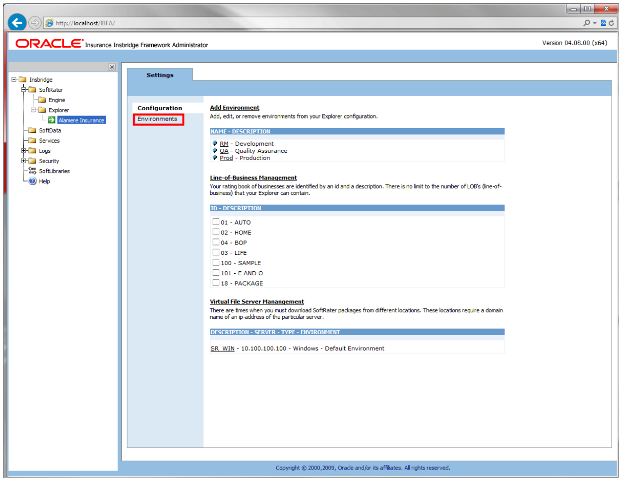
Figure 47 Create a Rating Environment
