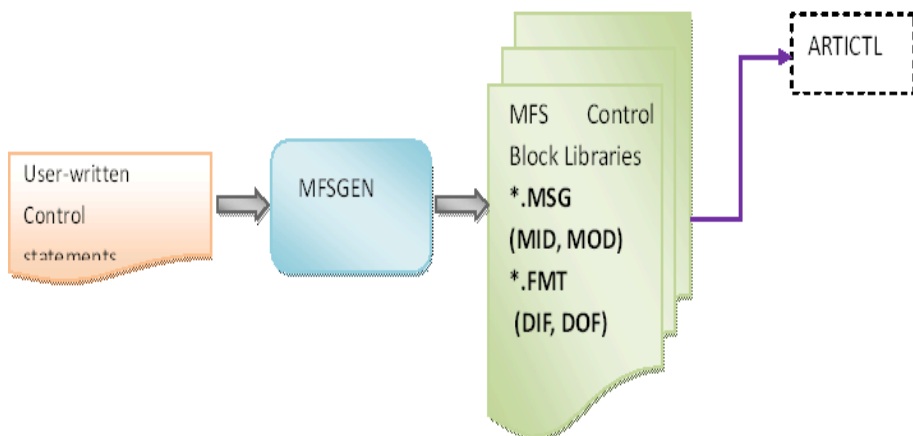
Figure 1 Mfsgen Workflow
