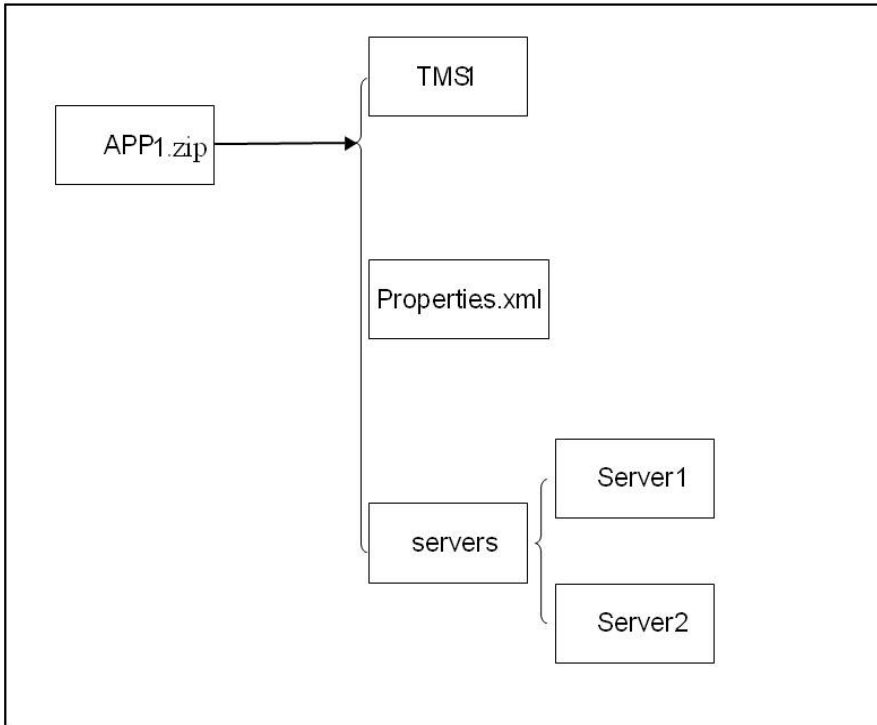
Figure 4-6 Application Package Structure
