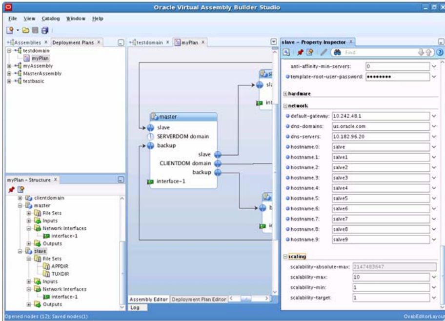
Figure 4-15 Set Scaling Parameters
