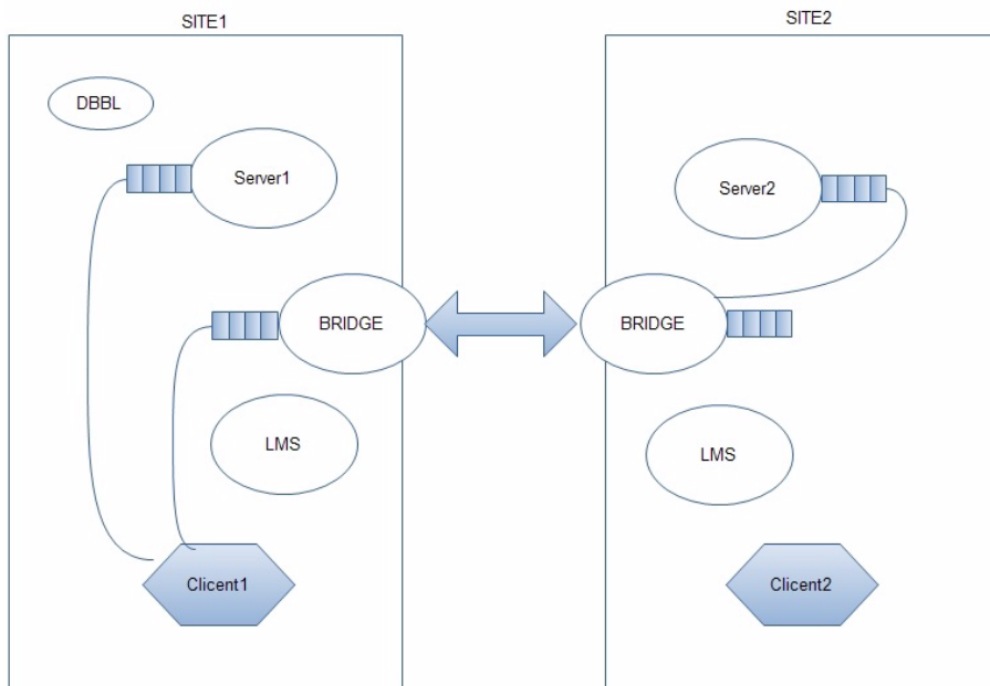
Figure 4-13 Dynamic Request Broker in MP Domain
