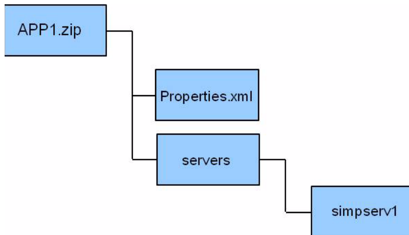
Figure 4-8 APP1.zip Content Structure
