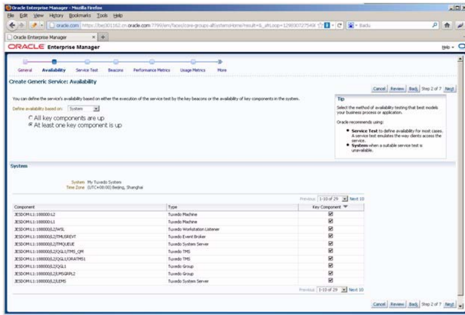
Figure 4-5 Creating Enterprise Manager services SLA (Continued)
