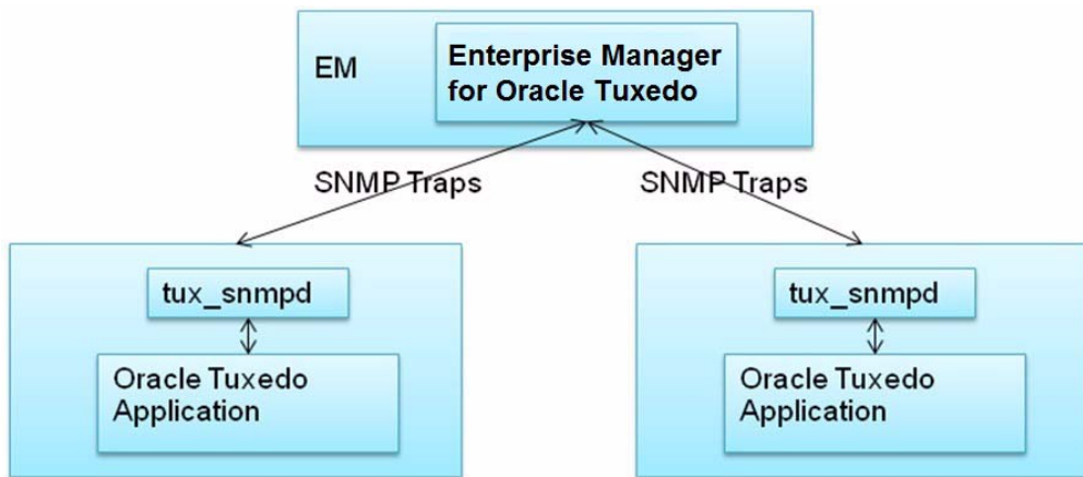
Figure 4-1 Tuxedo Event Monitoring Structure
