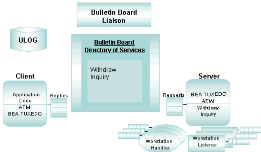
Figure 3-2 Bulletin Board and Bulletin Board Liaison
