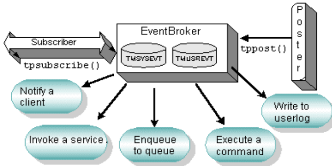
Figure 3-7 Handling Events Using TMUSREVT and TMSYSEVT
