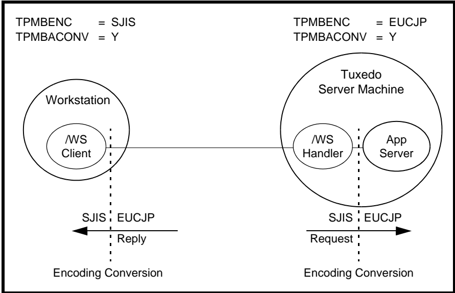
Figure 2-1 Encoding Conversion Using MBSTRING Buffers—Example
