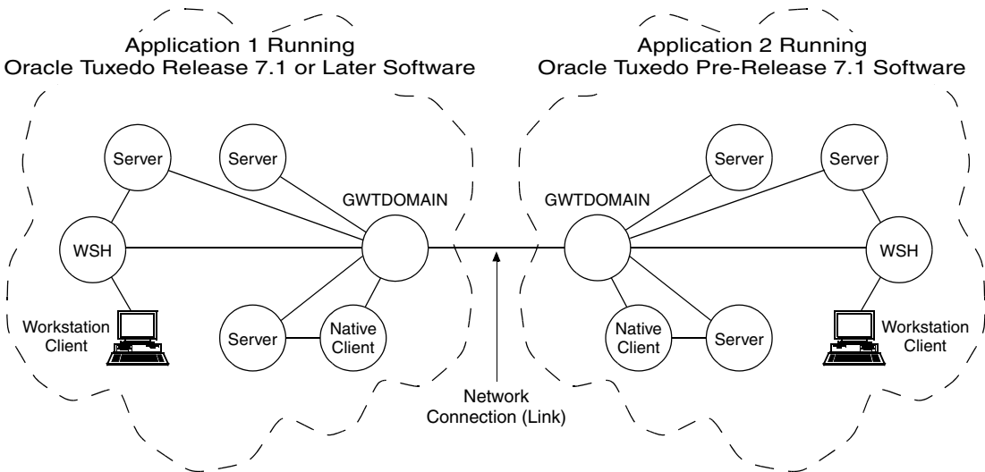
Figure 1-12 Inter-Domain Interoperability
