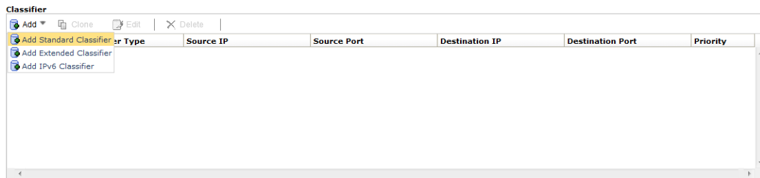
Figure 19: Classifier Table with Drop-down Menu
