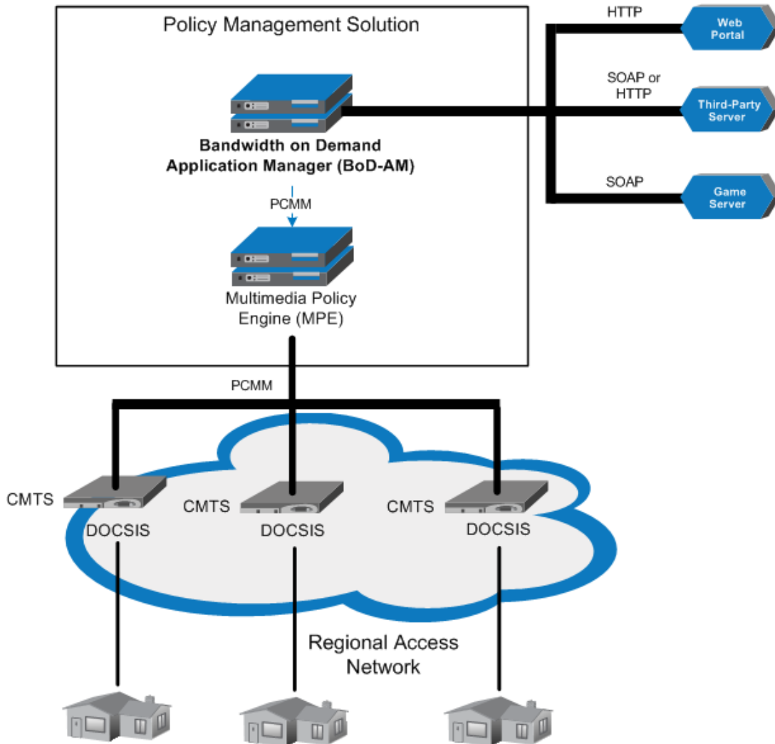
Figure 2: SOAP and HTTP Interface
