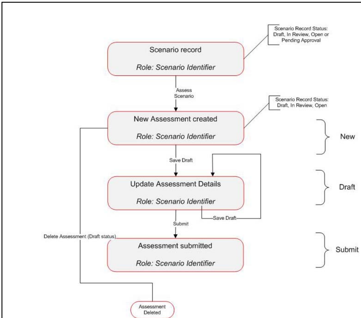
Figure 195. Scenarios Assessment Workflow
