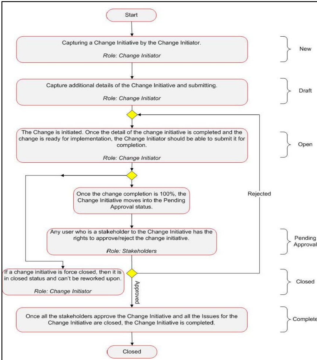
Figure 167. Change Management Workflow
