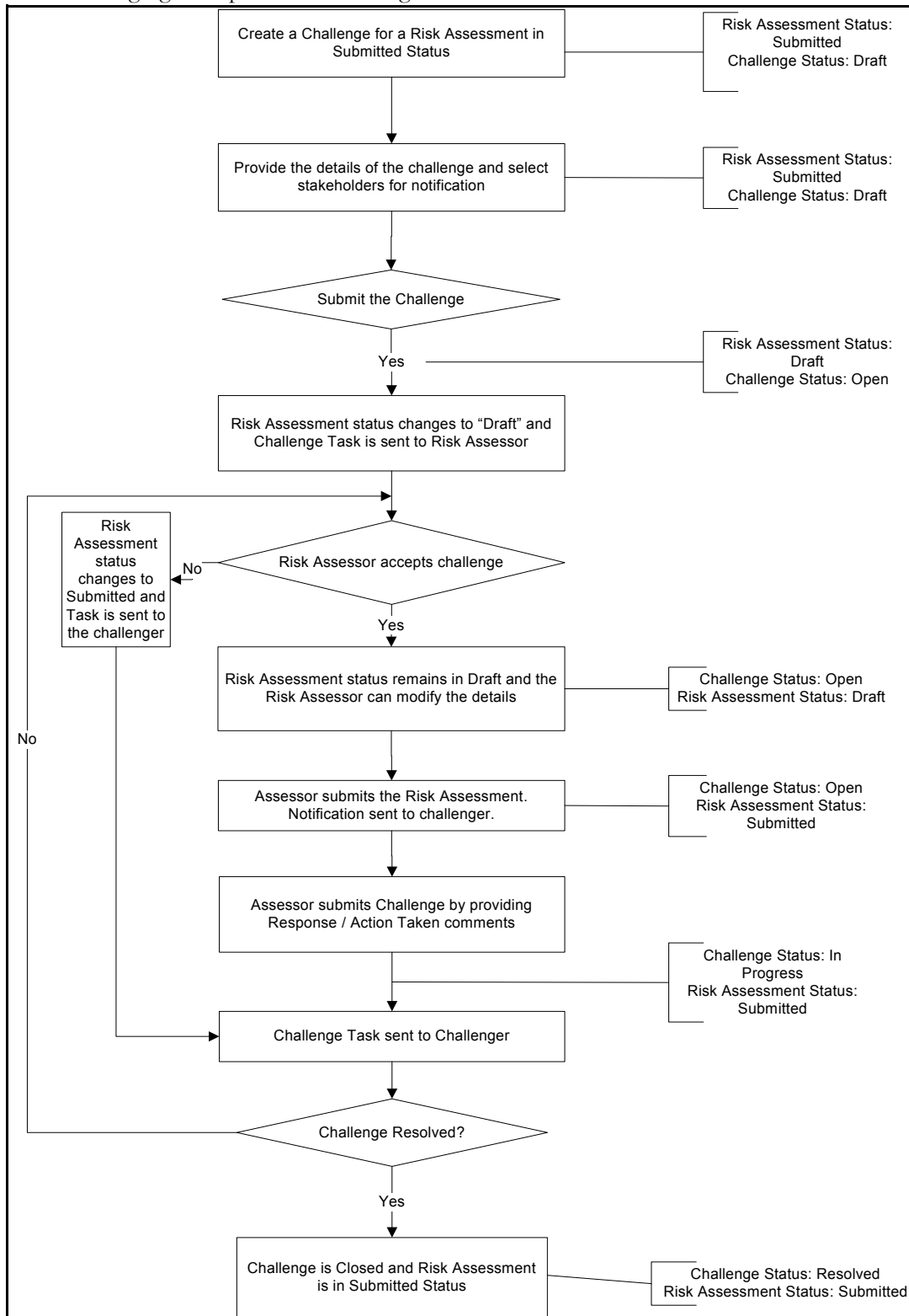
Figure 63. Assessment Challenge Workflow
