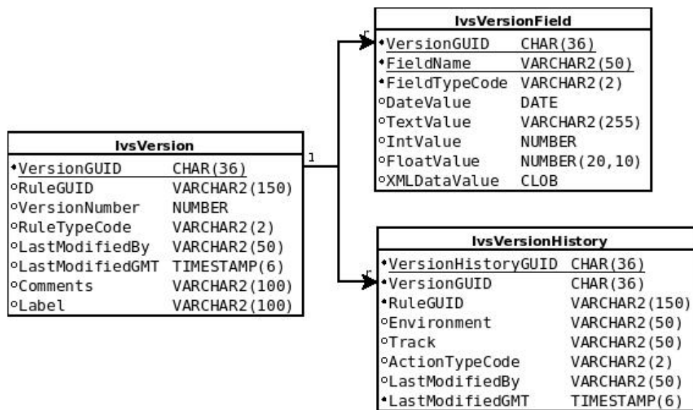
Figure 1: Version Table Structure
