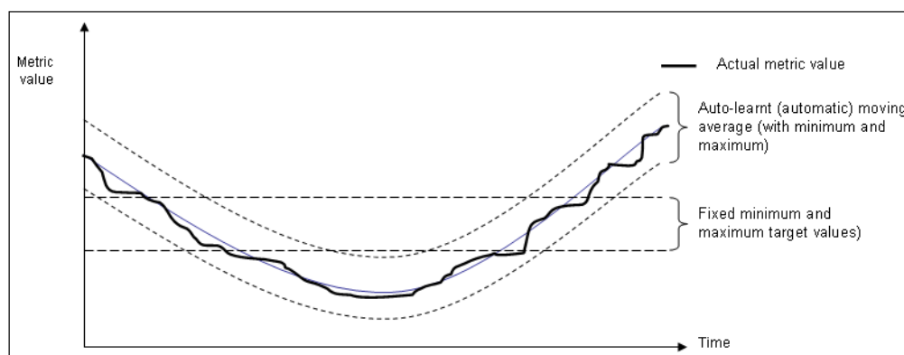
Figure 7-3 Automatic and Fixed KPI Targets Contrasted
