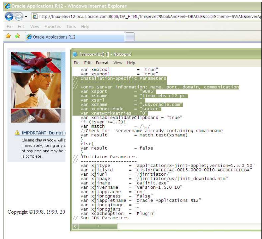
Figure N-7 Example Launch Page Details
