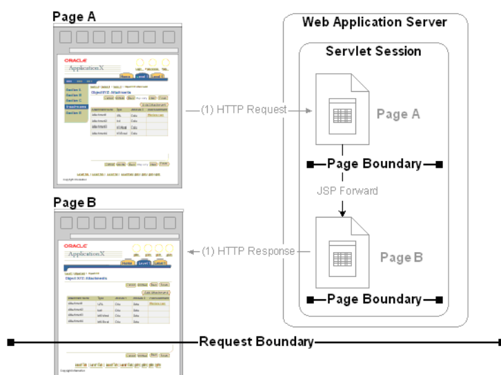
Figure N-9 Different Request and Page Boundaries in the JSP Forward Case
