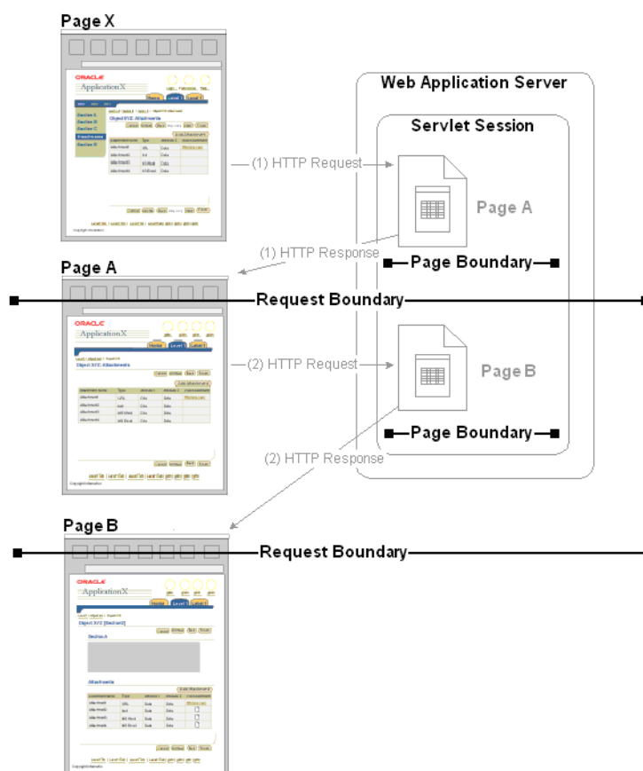
Figure N-8 Request and Page Boundaries the Same
