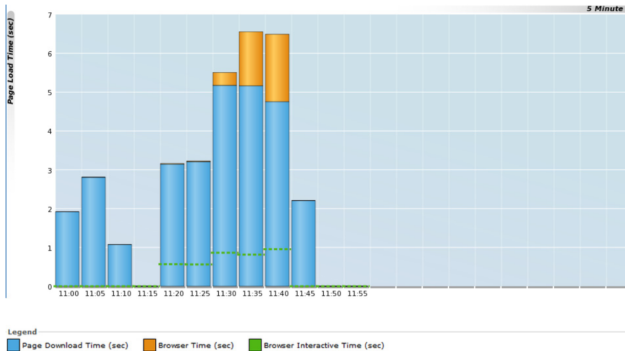
Figure 12–34 Page Loading Time Breakdown View
