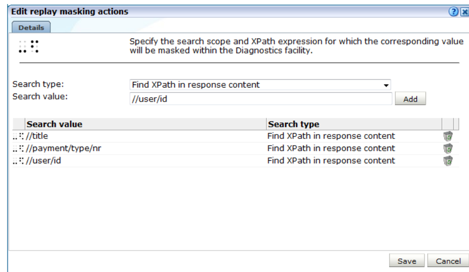
Figure 13–26 Edit Replay Masking Actions Dialog
