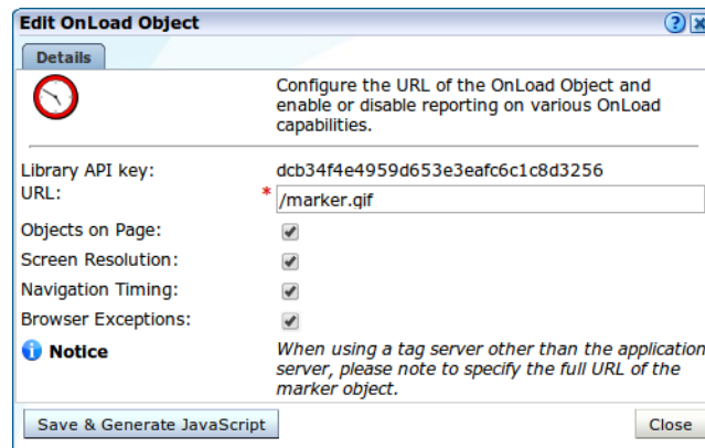
Figure 8-6 Edit OnLoad Object Dialog
