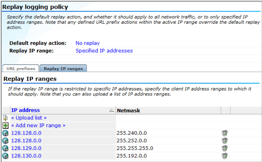
Figure 13–32 Replay Logging Policy Window
