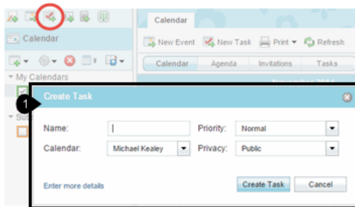
Figure 3–31 Convergence Calendar Create Task Dialog Widget
