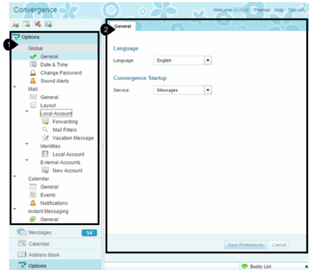
Figure 3–55 Common Convergence Option Widgets
