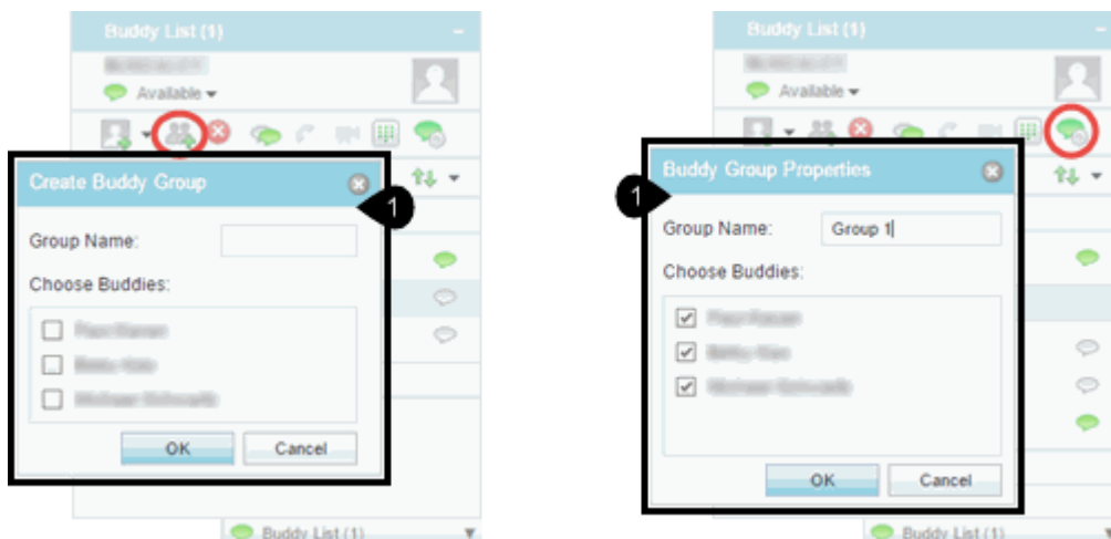
Figure 3–48 Convergence Instant Messaging Group Properties Dialog Widget
