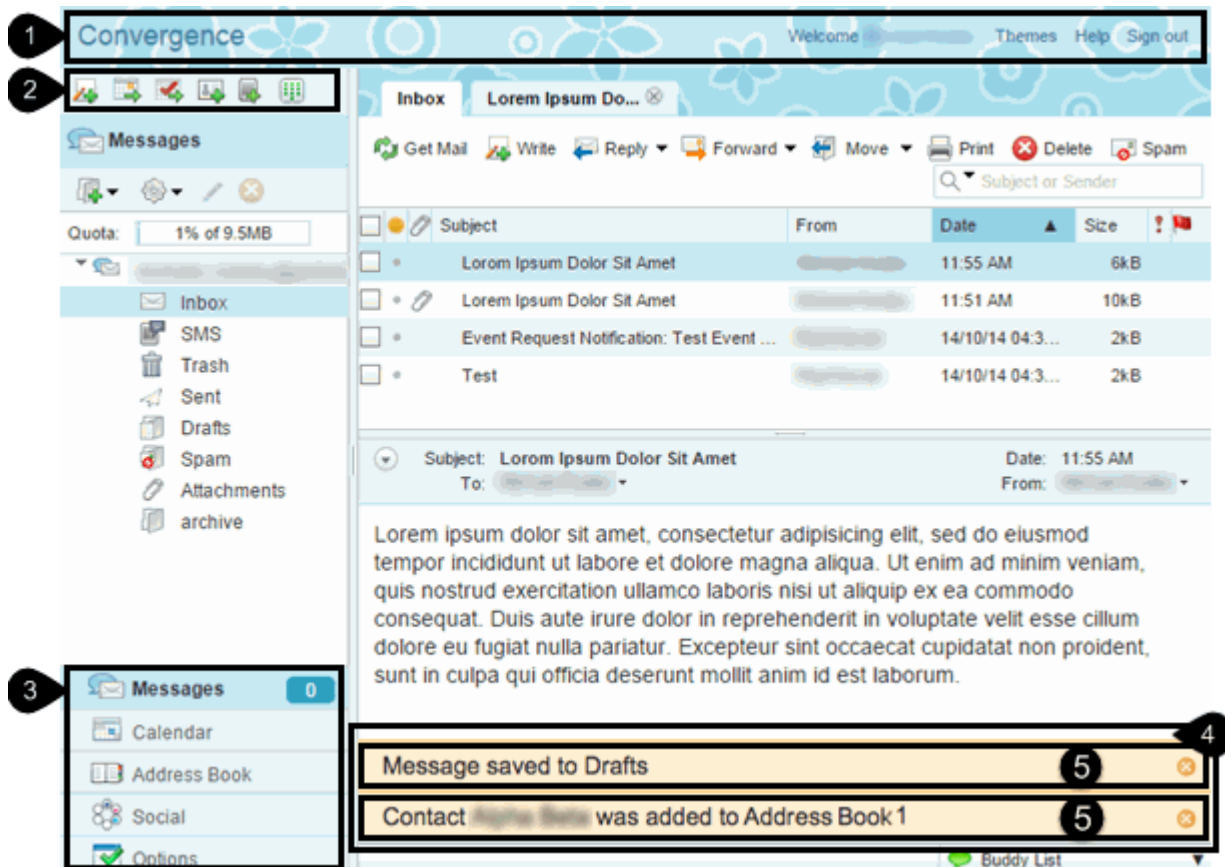
Figure 3–1 Common Widgets in Convergence UI
