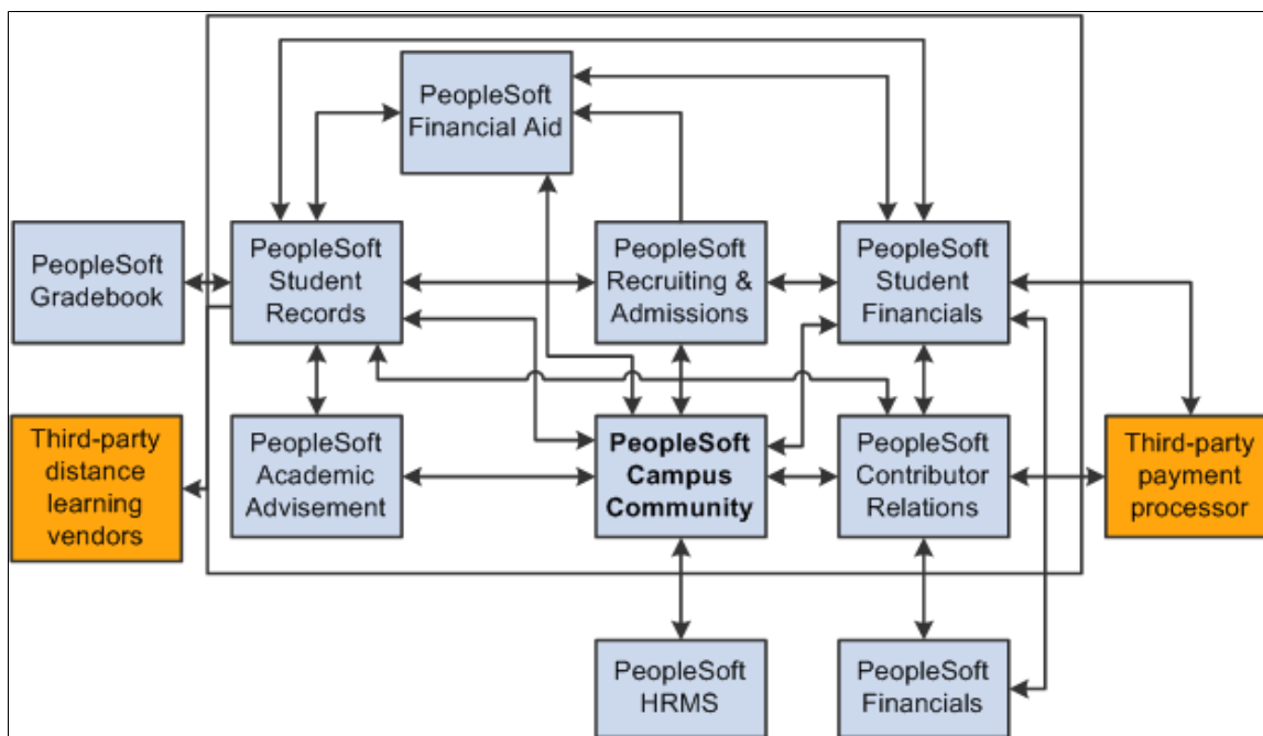
PeopleSoft Campus Community integrations
