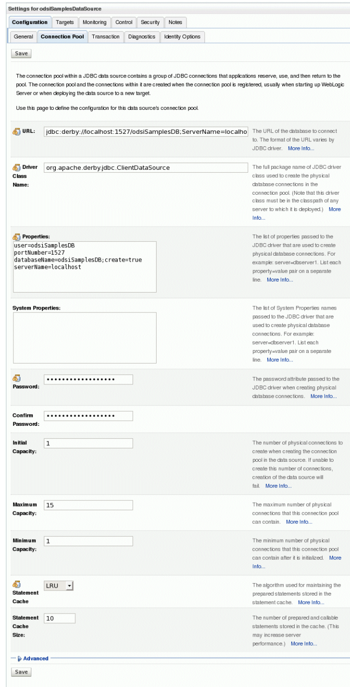
Figure 4–13 WebLogic Server Administration Console Connections Tab
