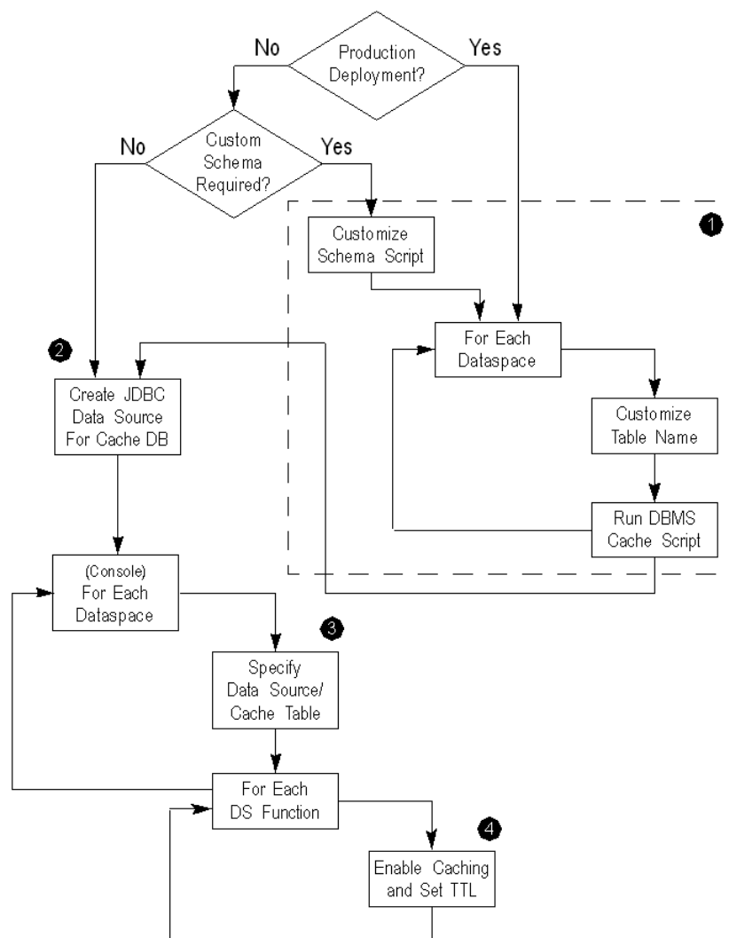
Figure 8–1 Cache Setup Steps
