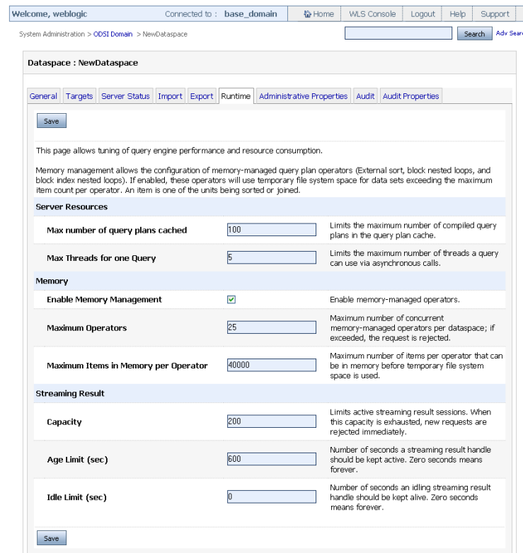
Figure 4–9 Oracle Data Service Integrator Administration Console: Runtime Tab
