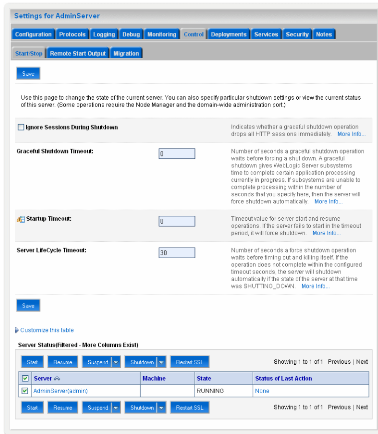
Figure 2–2 Graceful Shutdown of a Server
