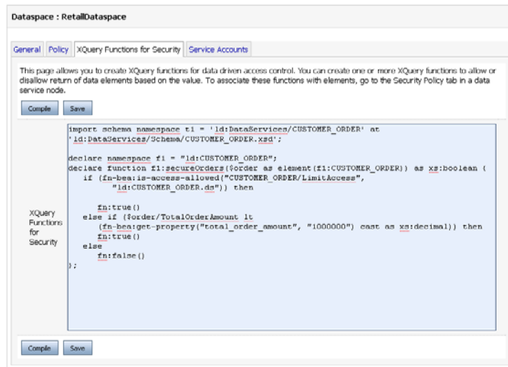
Figure 5–7 Security XQuery Functions
