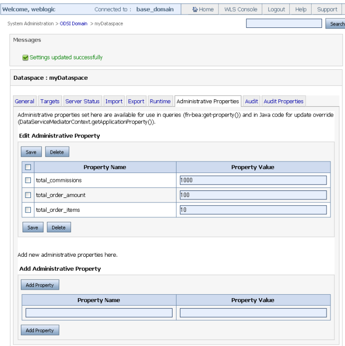
Figure 4–10 Administrative Properties Tab
