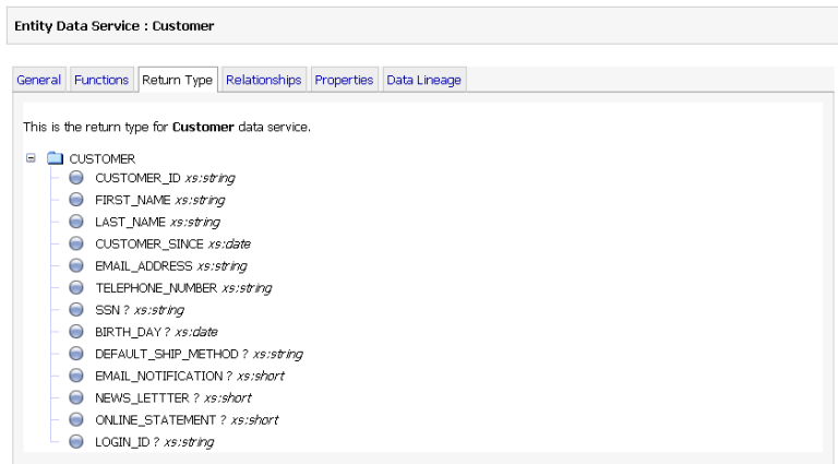
Figure 7-3 Return Type for a Logical Data Service
