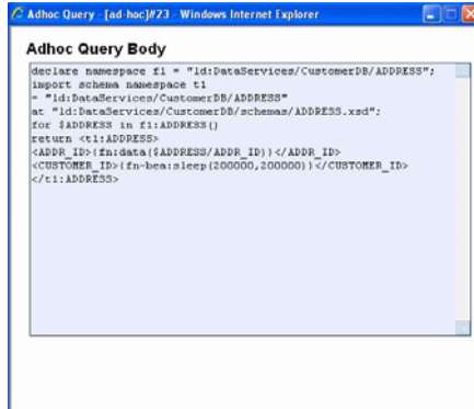
Figure 4–12 Ad Hoc Query Displayed on Oracle Data Service Integrator Administration Console
