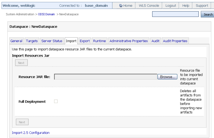
Figure 3-9 System Administration Category: Import Tab
