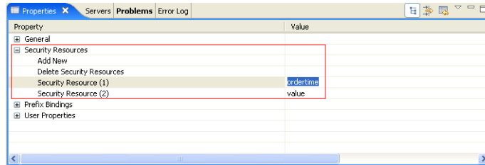
Figure 5–20 Oracle Data Service Integrator IDE Property Editor: User-Defined Security Resources
