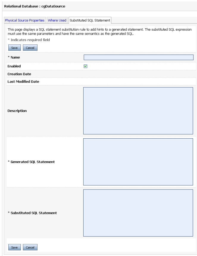
Figure 4–4 Substituted SQL Statement Dialog Box
