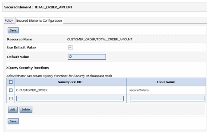
Figure 5–8 Applying XQuery Functions for Security
