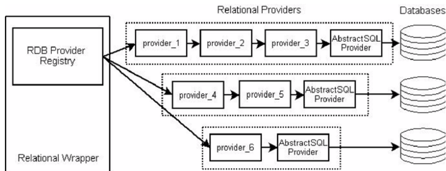
Figure 10–1 Database Extension Framework Architecture
