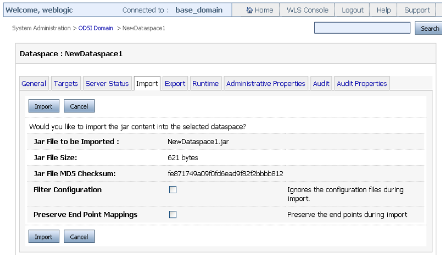
Figure 3–10 Resource File Details
