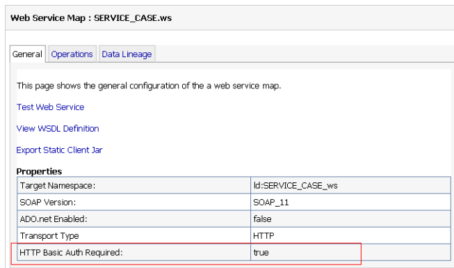
Figure 5–19 Basic Auth Required Property Information in Service Explorer
