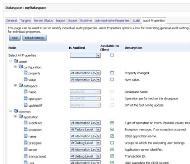
Figure 4–6 Setting the basesql Property to Always be Returned
