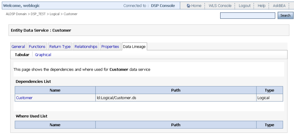
Figure 7-2 Logical Data Service Dependencies and Where Used
