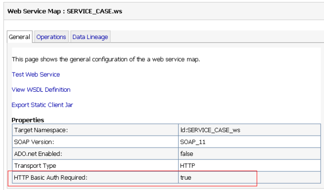
Figure 6–1 Native Web Service: General Tab
