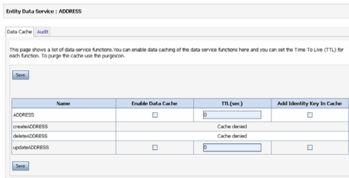
Figure 8–3 Enabling Caching by Function
