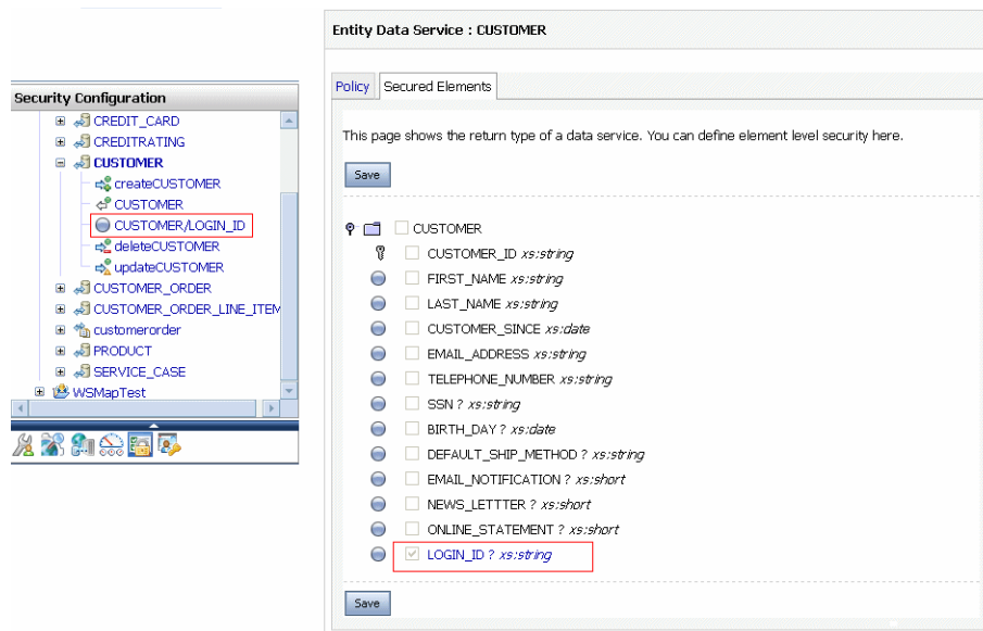
Figure 5–16 Secured Data Element in the Navigation Tree
