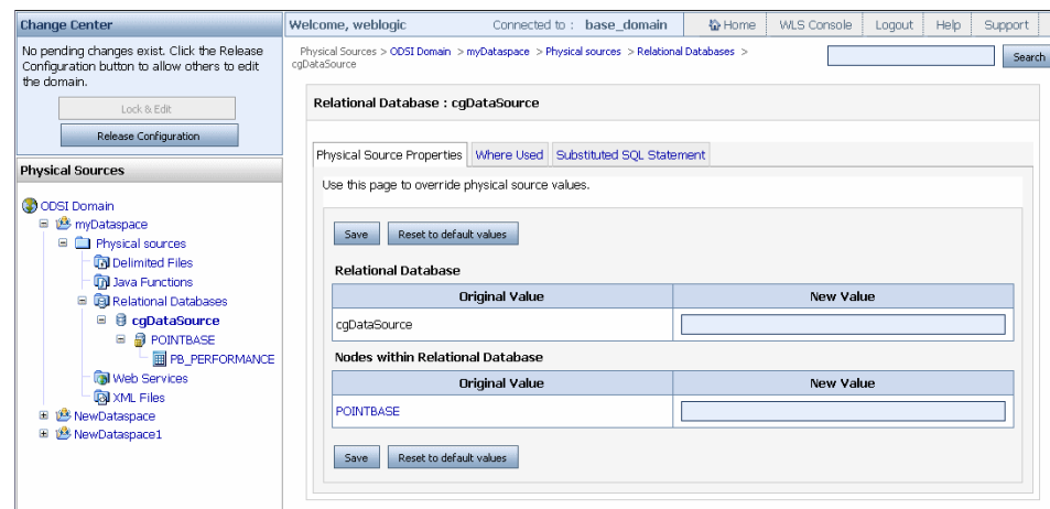
Figure 4–3 Setting End Points for Relational Sources
