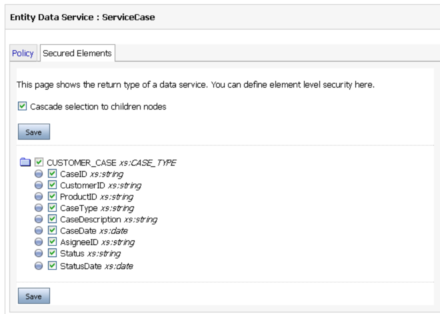
Figure 5–17 Securing Data Elements at the Data Service Level
