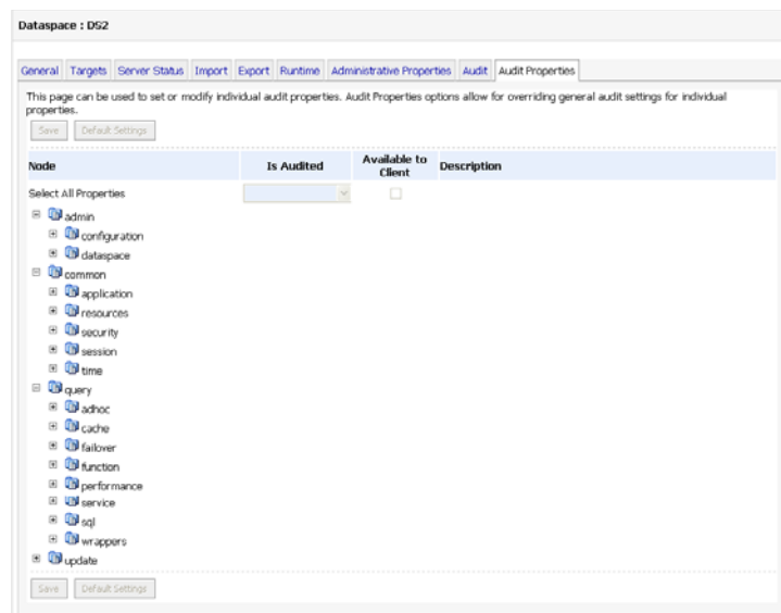
Figure 9–2 Audit Properties Tab
