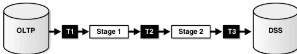
Figure 13–1 Typical Data Processing with Non-Parallel, Non-Pipelined Table Functions
