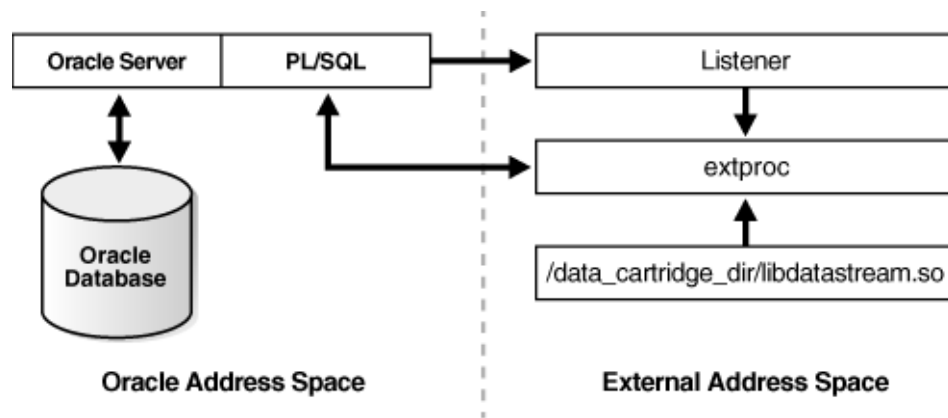
Figure 5-1 Calling an External Procedure
