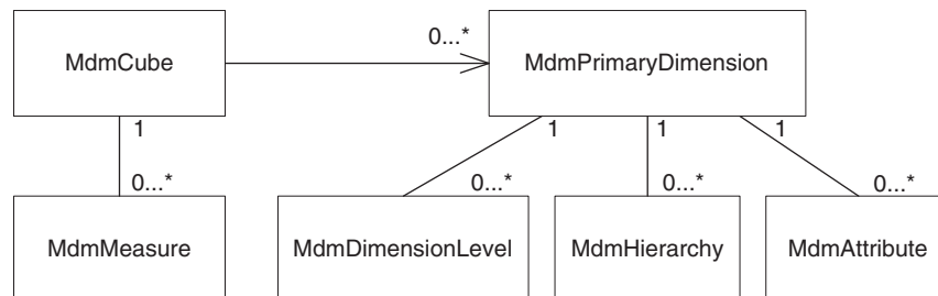
Figure 2–5 Associations of Dimensional Data Model Classes
