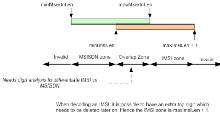
Figure 13: IMSI/MSISDN Overlap Range Scenario
