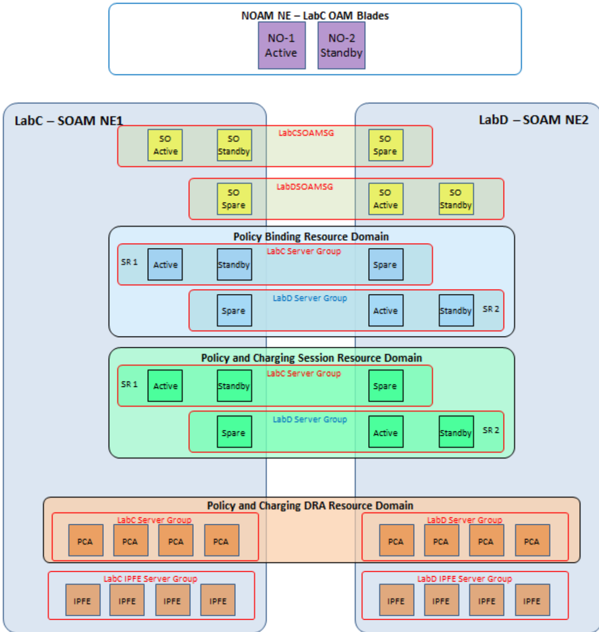
Figure 2. Example - PCA / Policy and Charging SBR Topology
