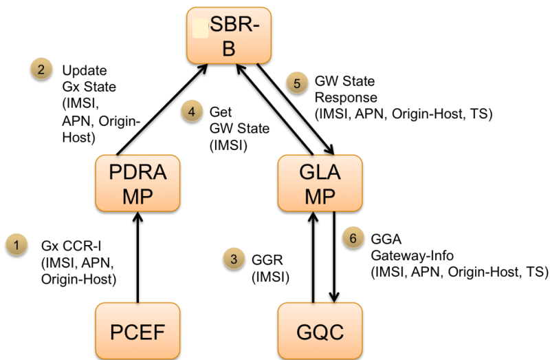
Figure 34 - IMSI Query with Single Matching Gx Session Use Case
