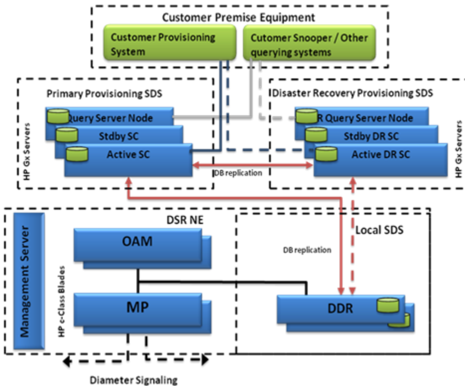
Figure 38 - Subscriber Data Server Architecture
