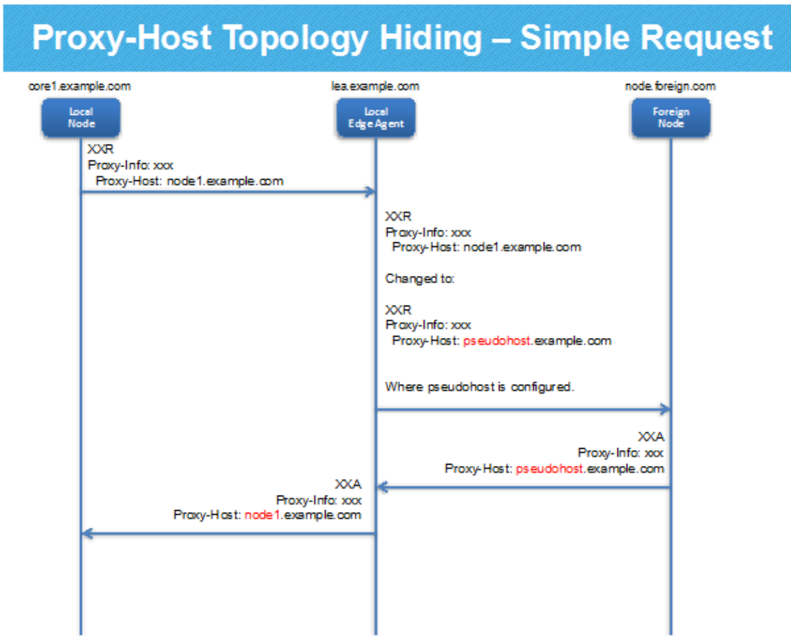
Figure 20 - Proxy-Host Topology Hiding Message Flow
