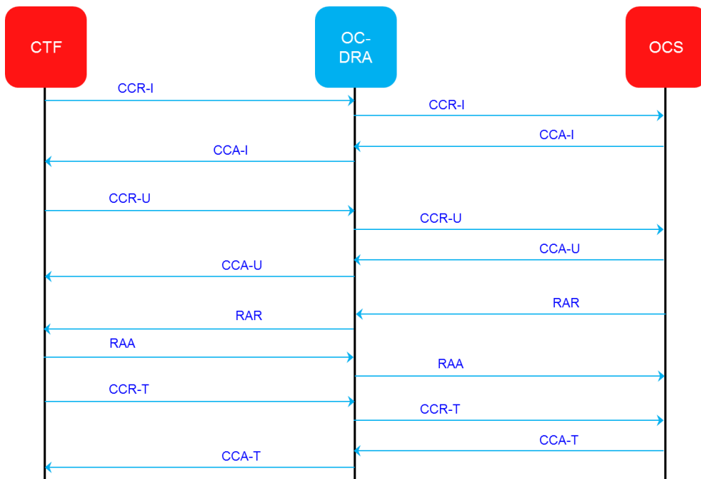
Figure 27: A typical Online Charging Session
