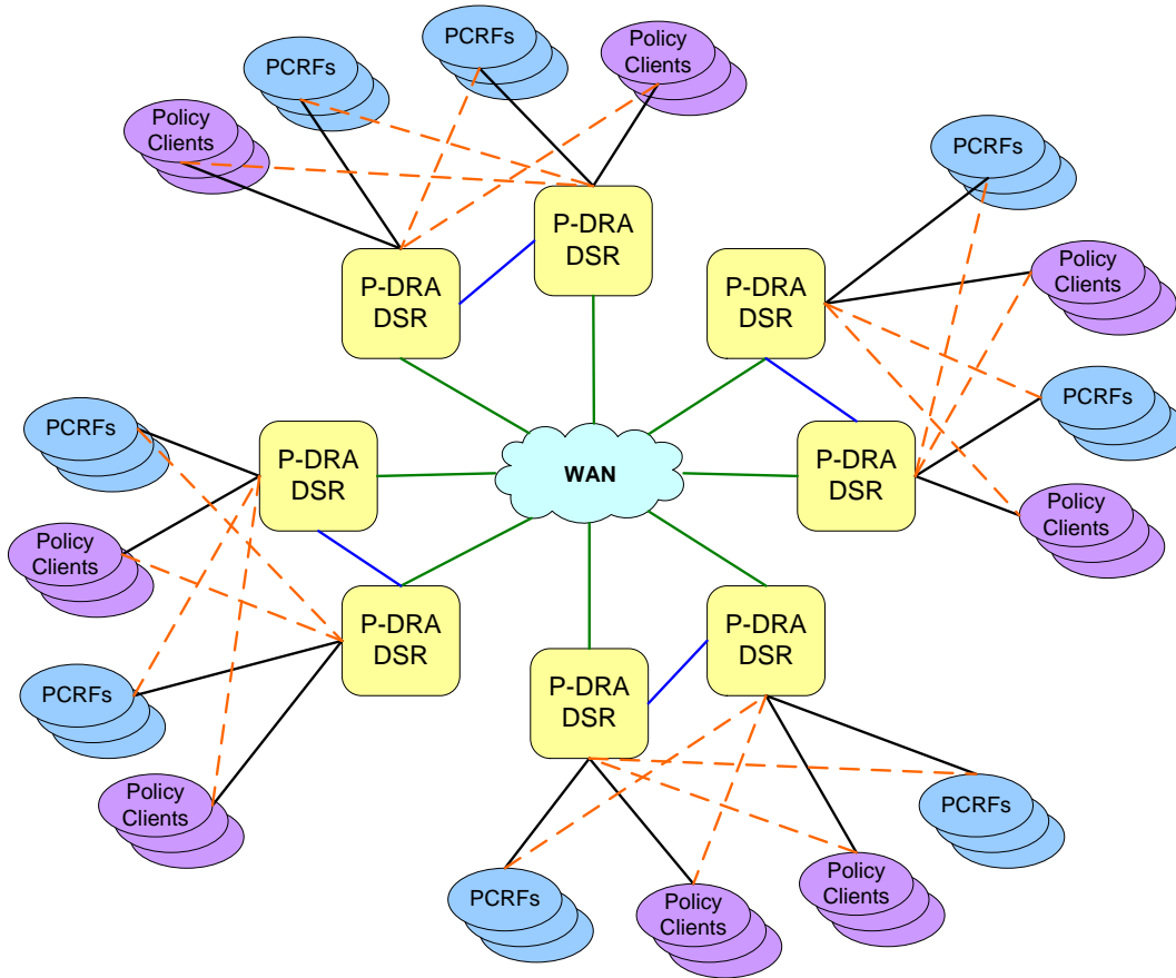
Figure 28 – Network View of P-DRA Mated Pairs
