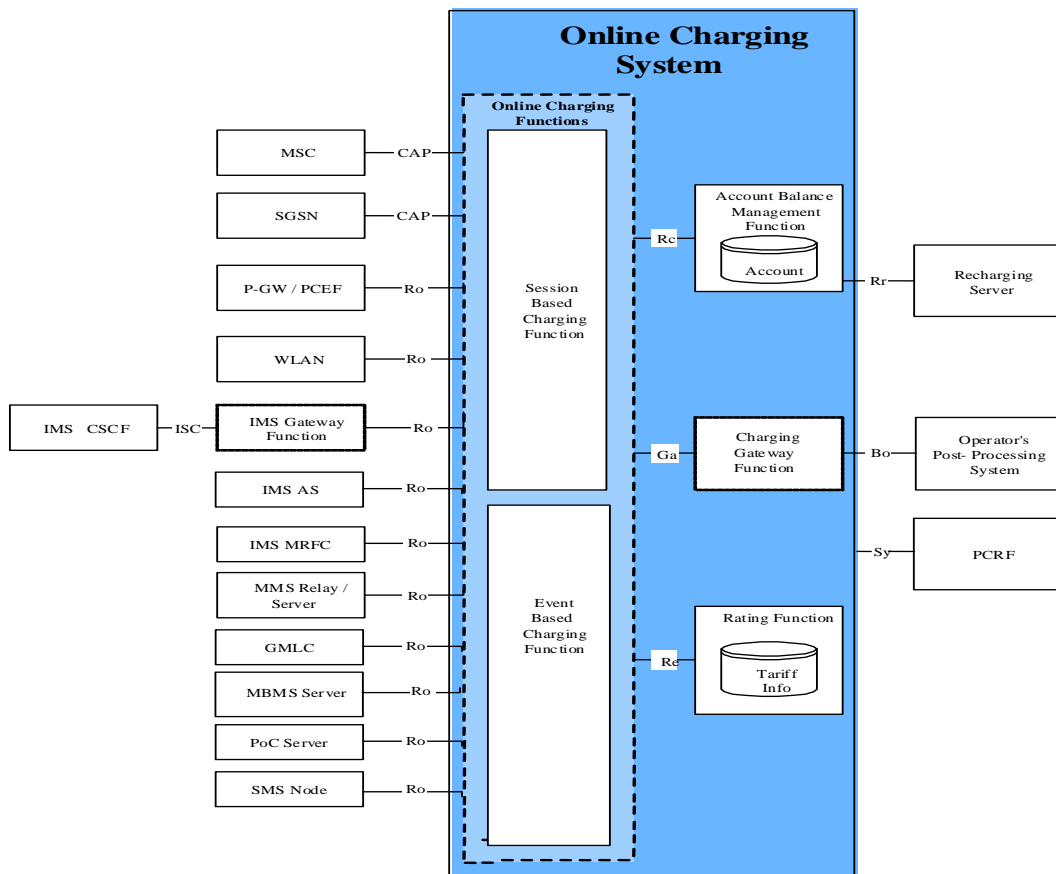
Figure 26 - Online Charging System and Architecture
