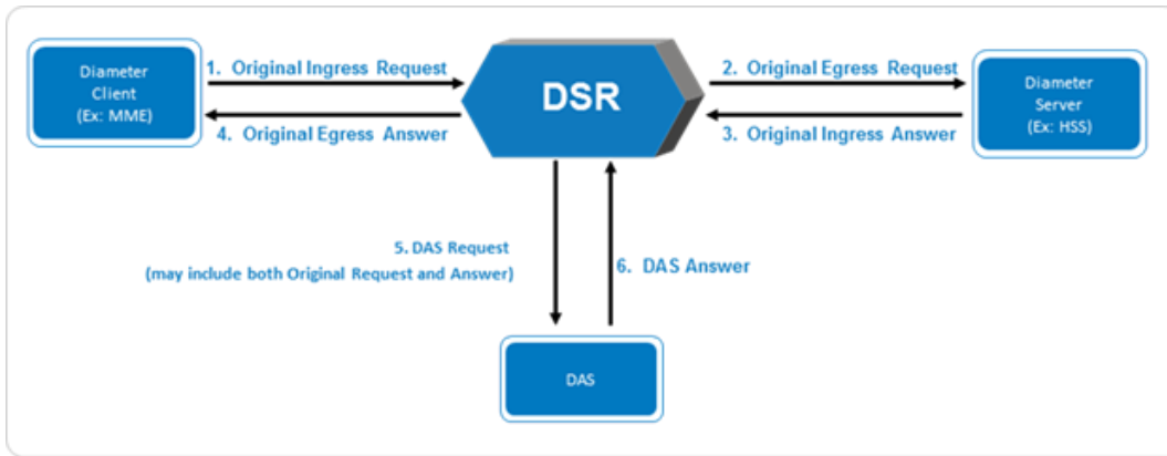
Figure 36 - Message Copy Overview
