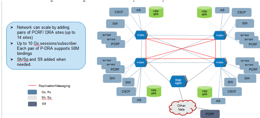
Figure 33 - PCA Example Deployment
