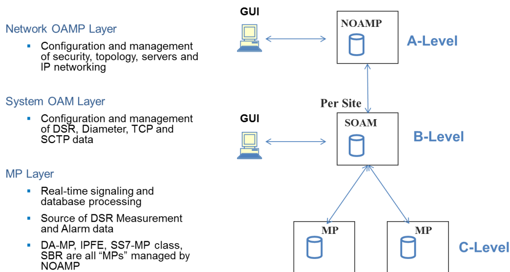
Figure 39 - DSR 3-tiered Topology Architecture
