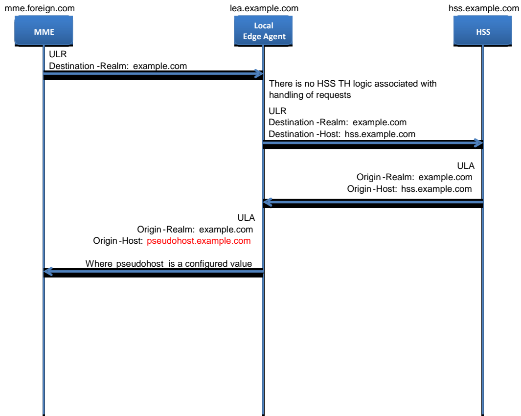
Figure 22 - S6a/S6d HSS Topology Hiding - ULR Message Flow
