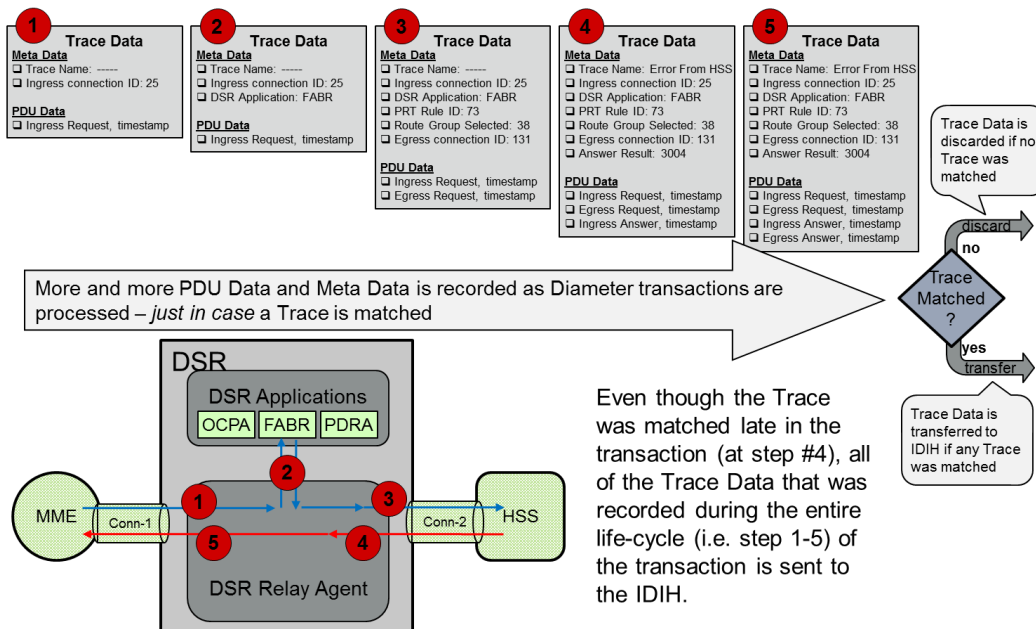
Figure 37 - IDIH Trace Data
