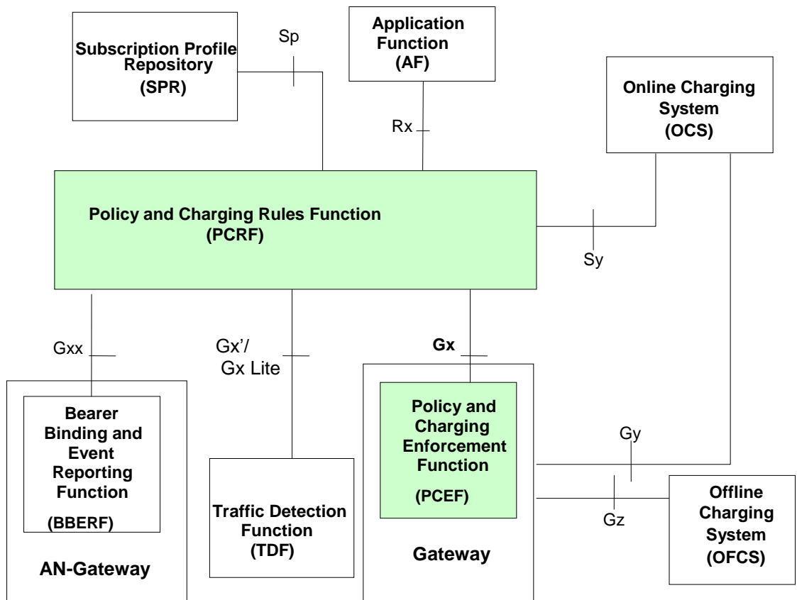
Figure 29 - Overall PCC logical architecture (non-roaming)
