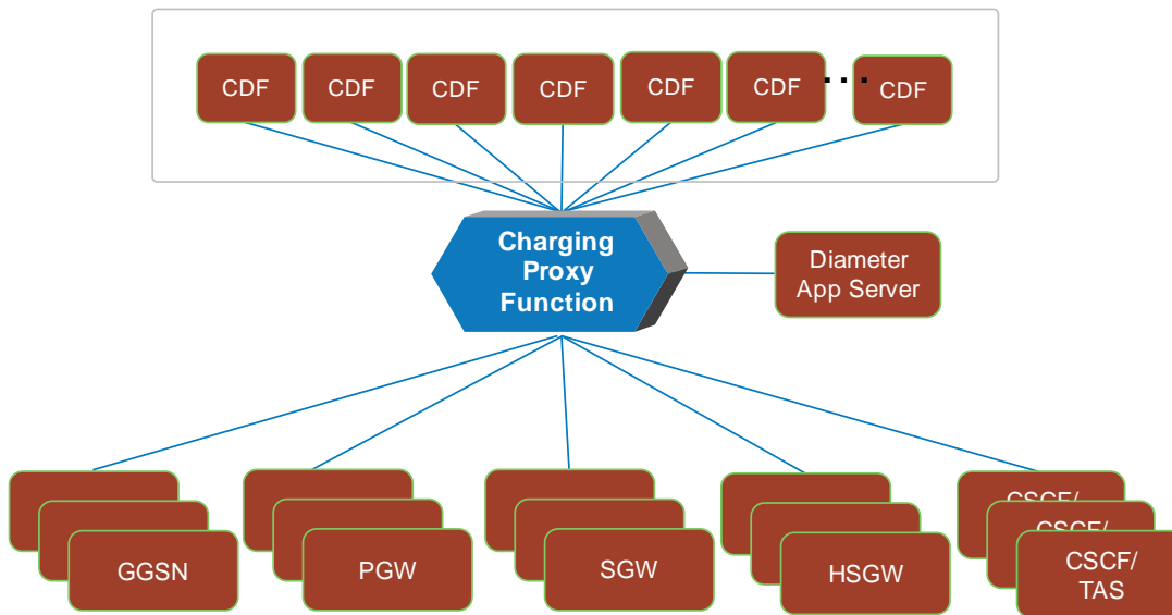
Figure 24 - Charging Proxy Network Architecture
