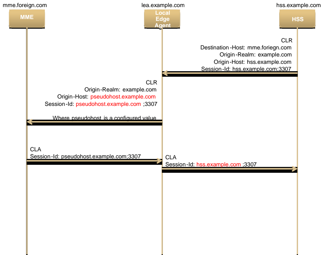
Figure 23 - S6a/S6d HSS Topology Hiding CLR Message Flow
