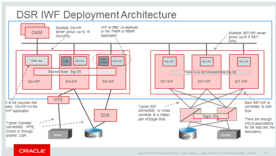
Figure 25 - DSR with MAP-Diameter IWF
