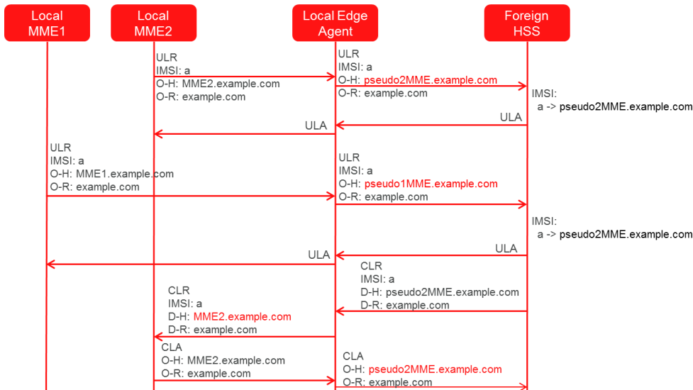
Figure 21 - MME/SGSN Topology Hiding
