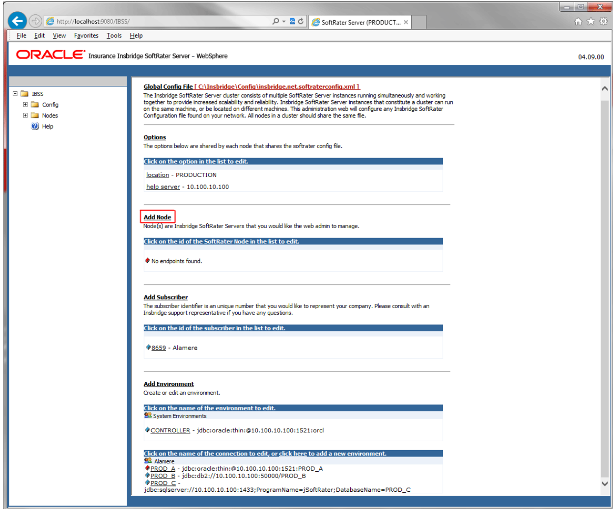
Figure 50 Adding a Controller Database Connection
