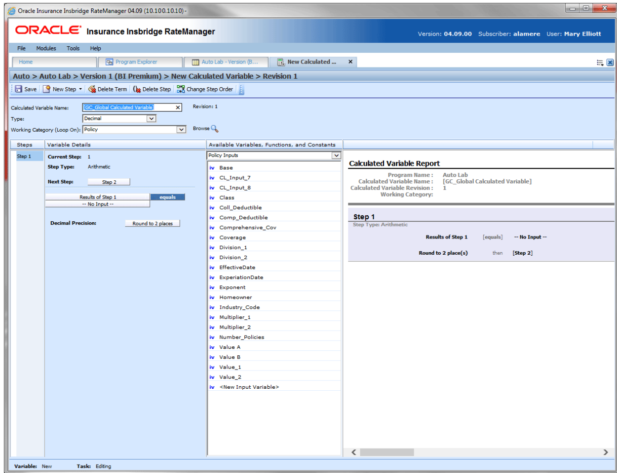
Figure 205 Creating a New Calculated Variable
