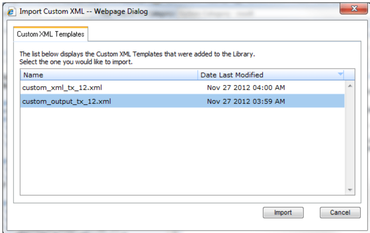
Figure 332 Uploading a Custom Output XML Template
