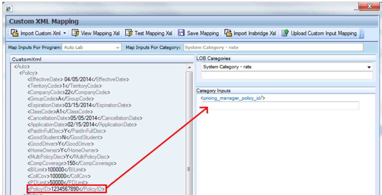
Figure 320 Mapping Custom XML
