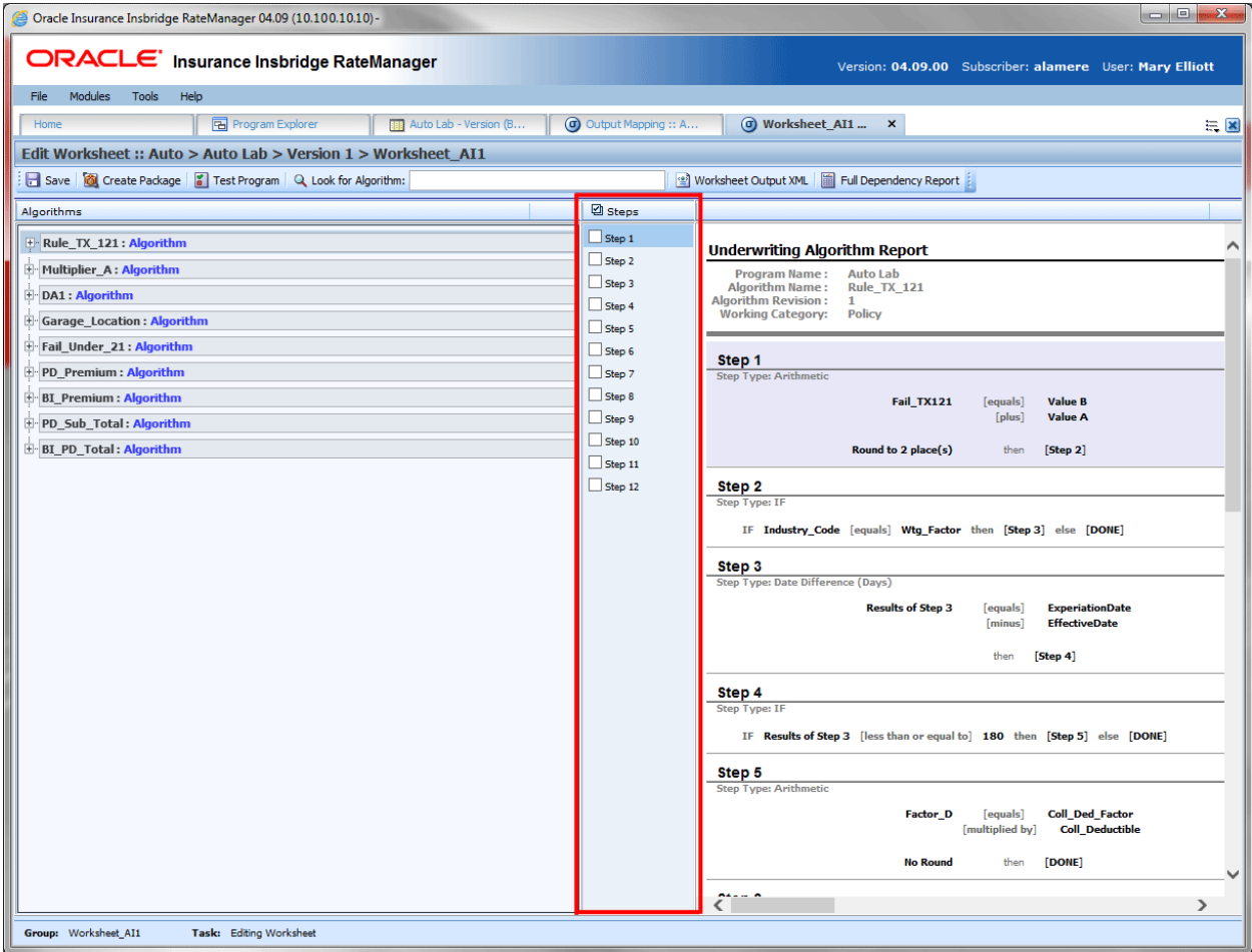
Figure 301 Edit Worksheet Steps
