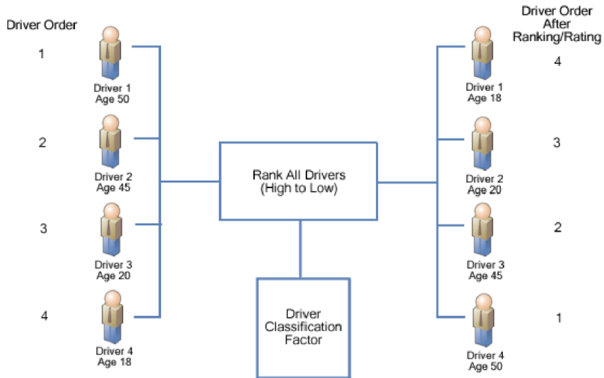
Figure 238 Ranking Functions
