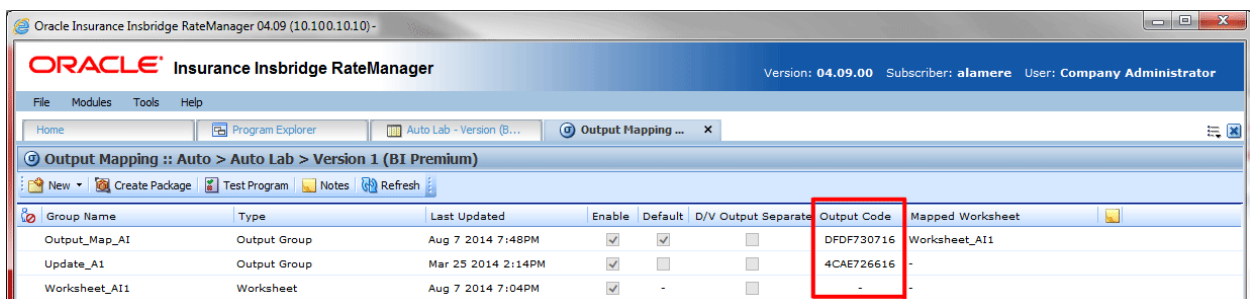
Figure 293 Output Codes
