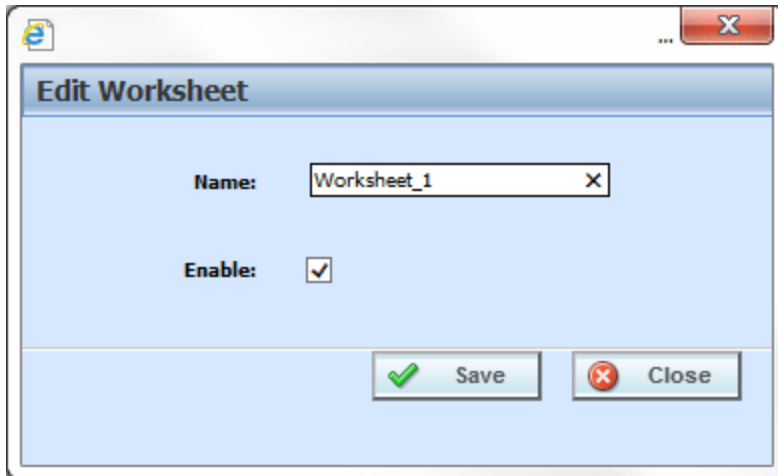
Figure 304 Worksheet Options
