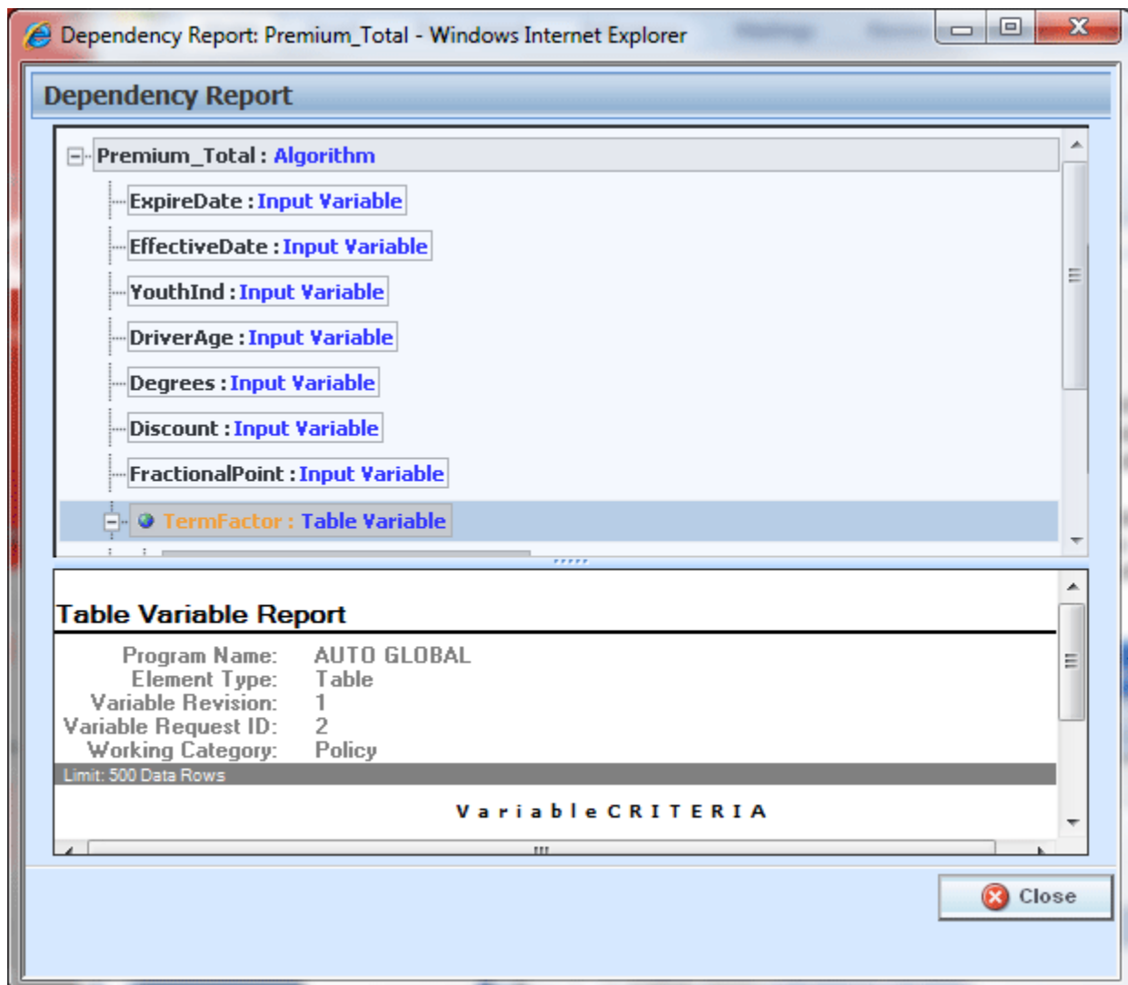
Figure 365 Dependency Report
