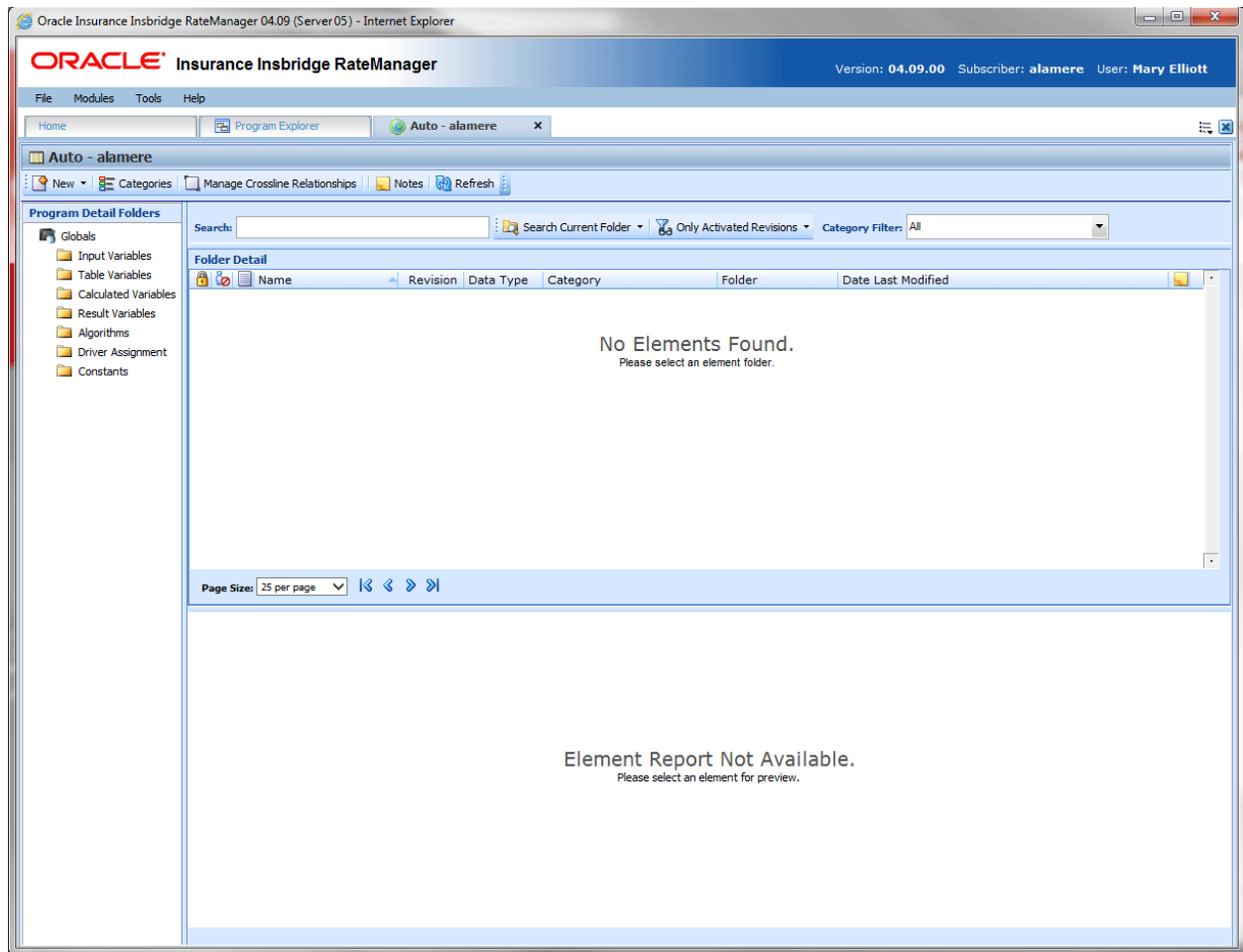
Figure 62 Global Tab
