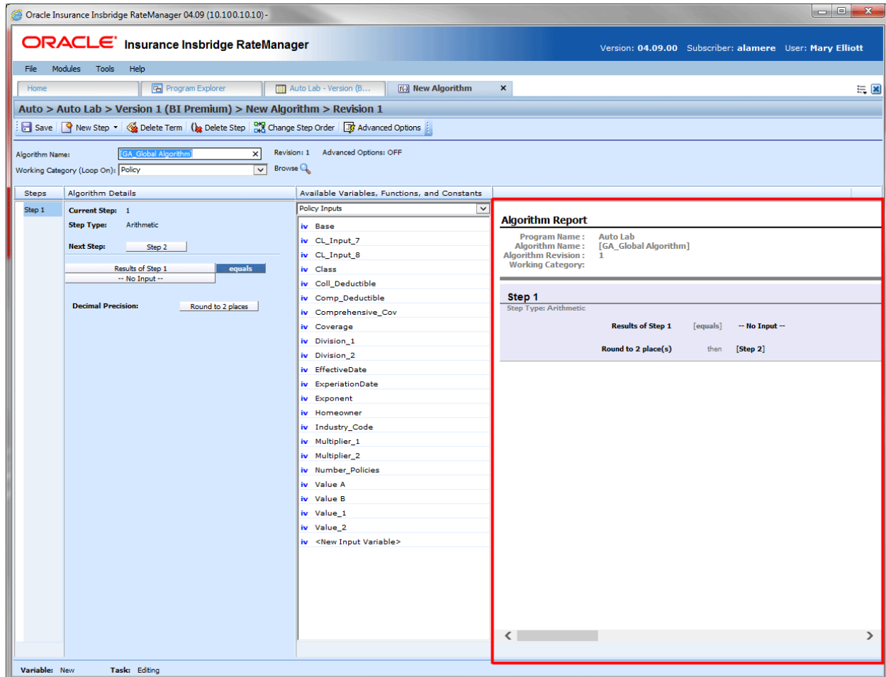
Figure 218 Algorithm Report
