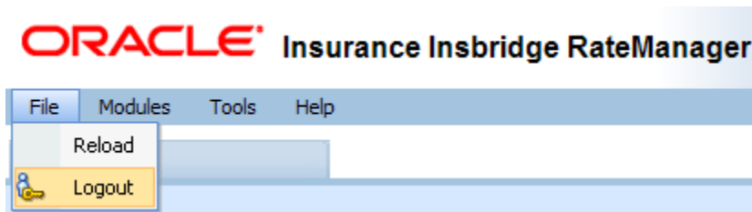
Figure 2 Logging Out
