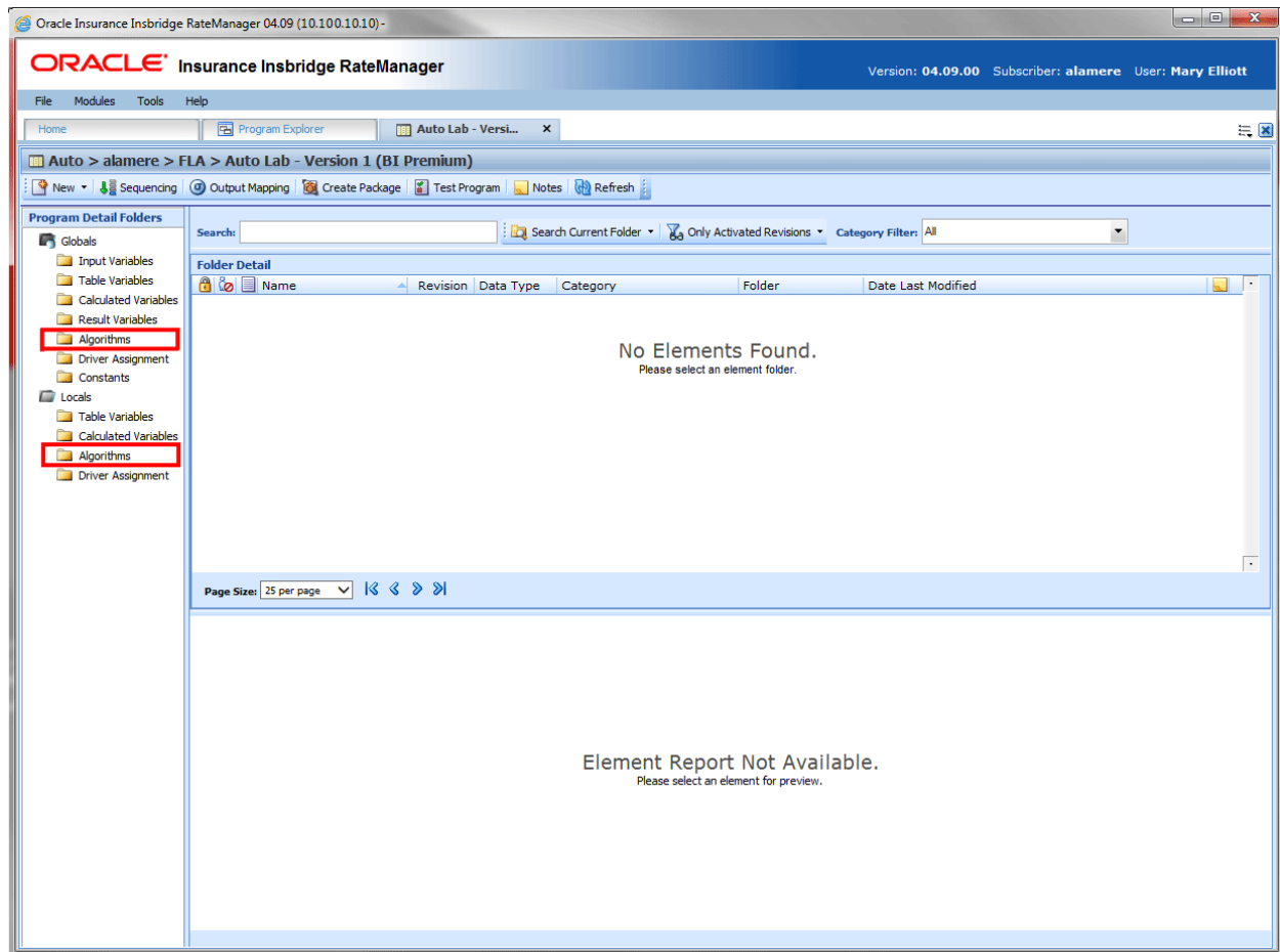
Figure 213 Algorithms Navigation
