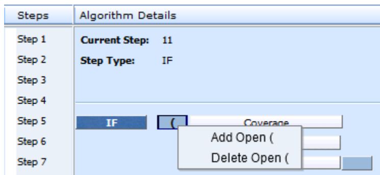
Figure 133 Adding an Open Parentheses
