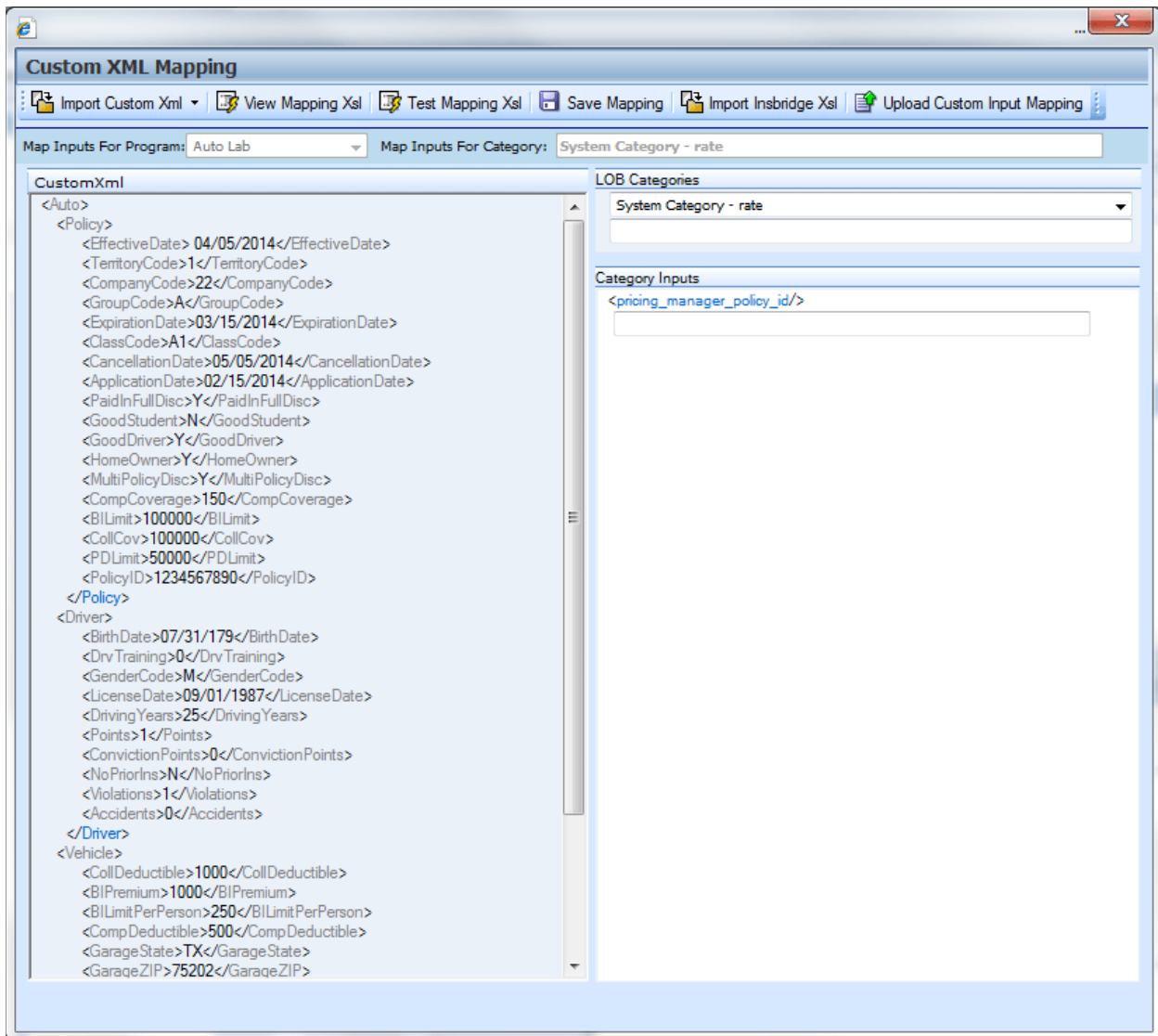
Figure 317 Imported Custom XML Template
