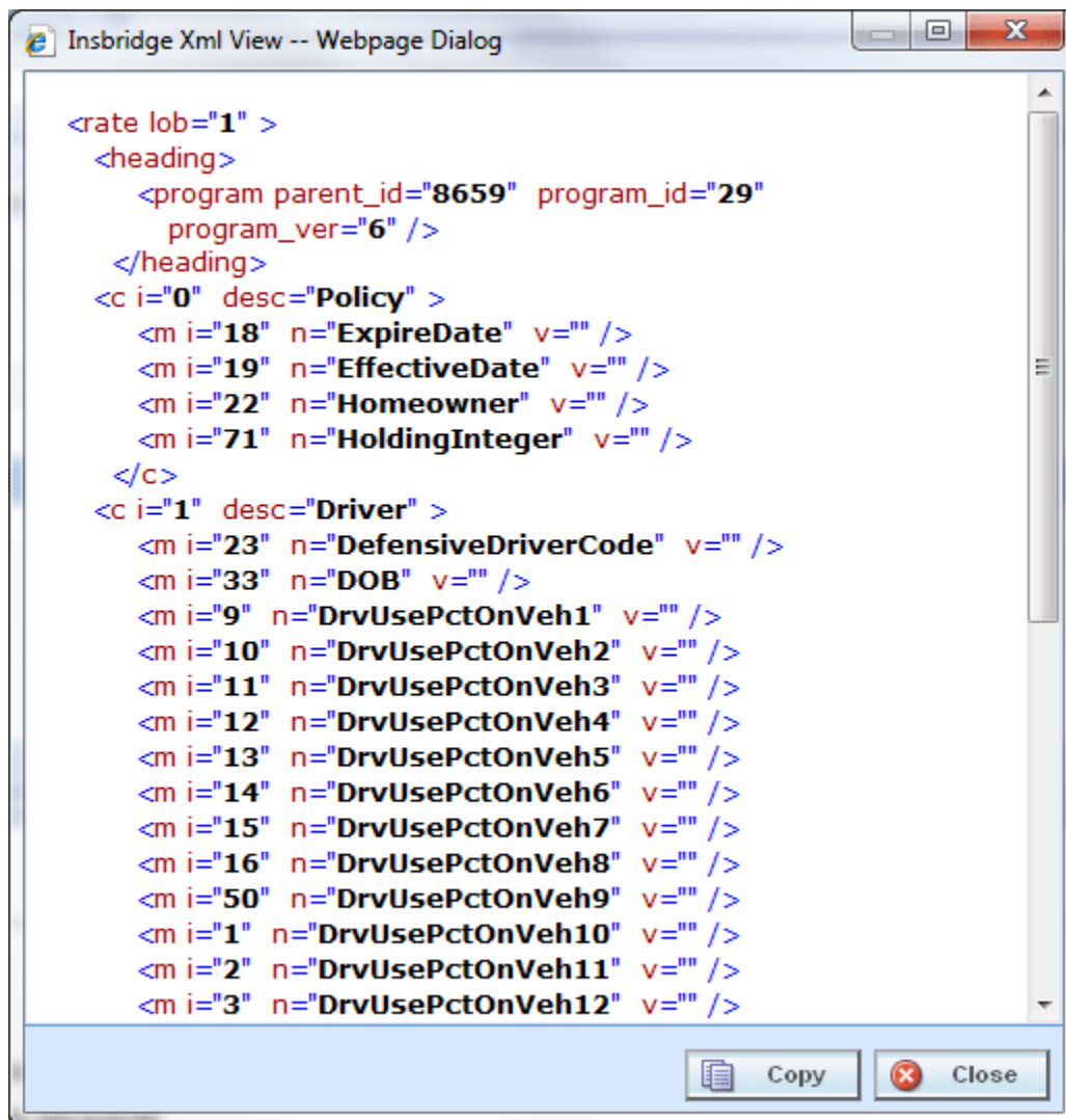
Figure 364 Program Inputs XML
