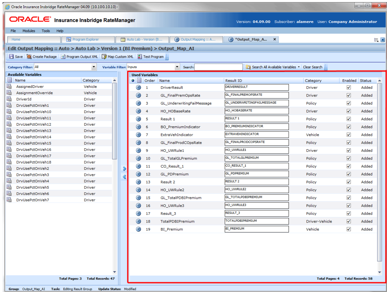
Figure 289 Available Variables for Output Mapping
