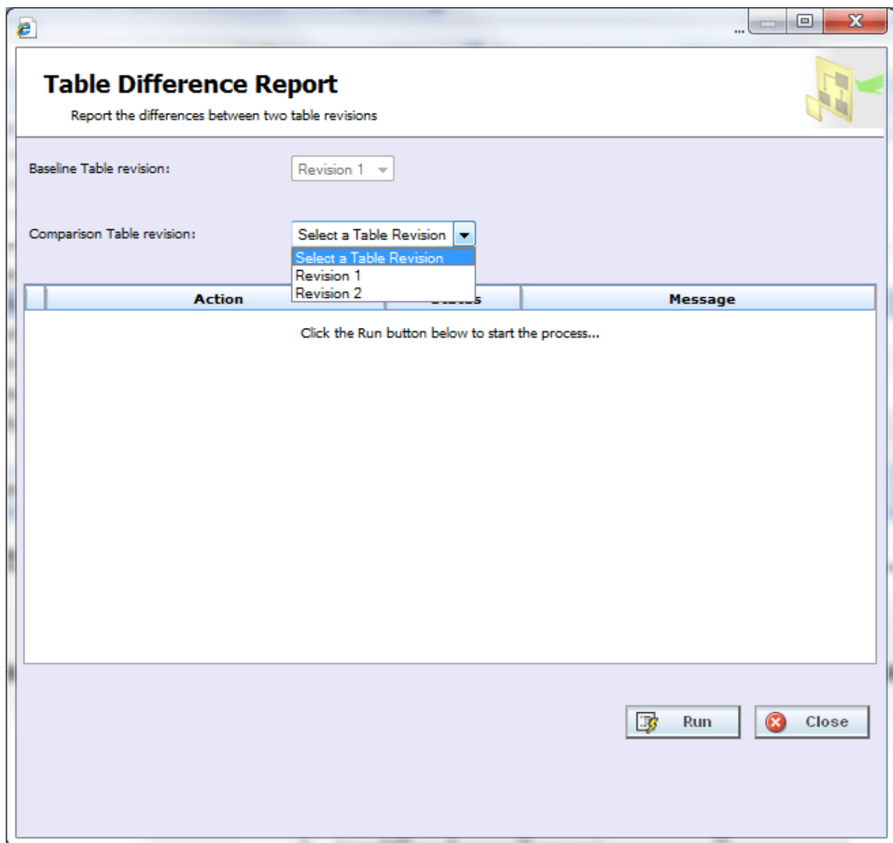
Figure 374 Selecting Revisions to Compare
