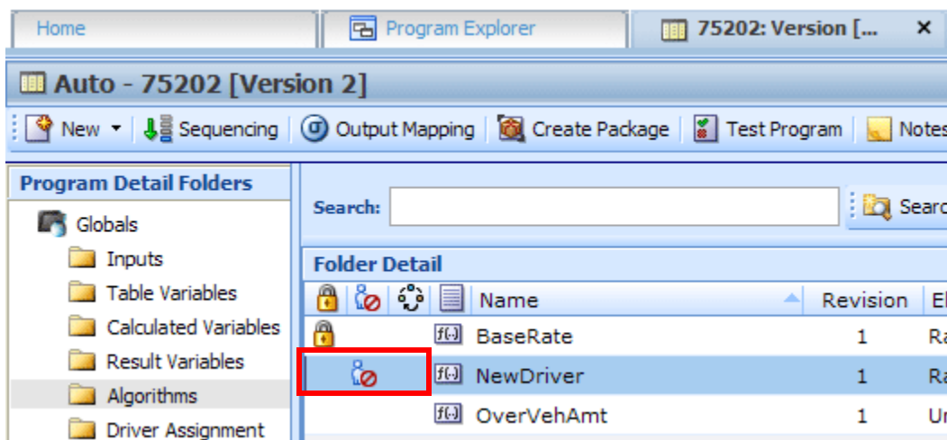
Figure 378 In-Use Locking on an Element
