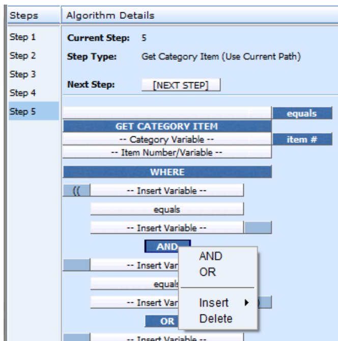
Figure 132 Editing a Where Clause
