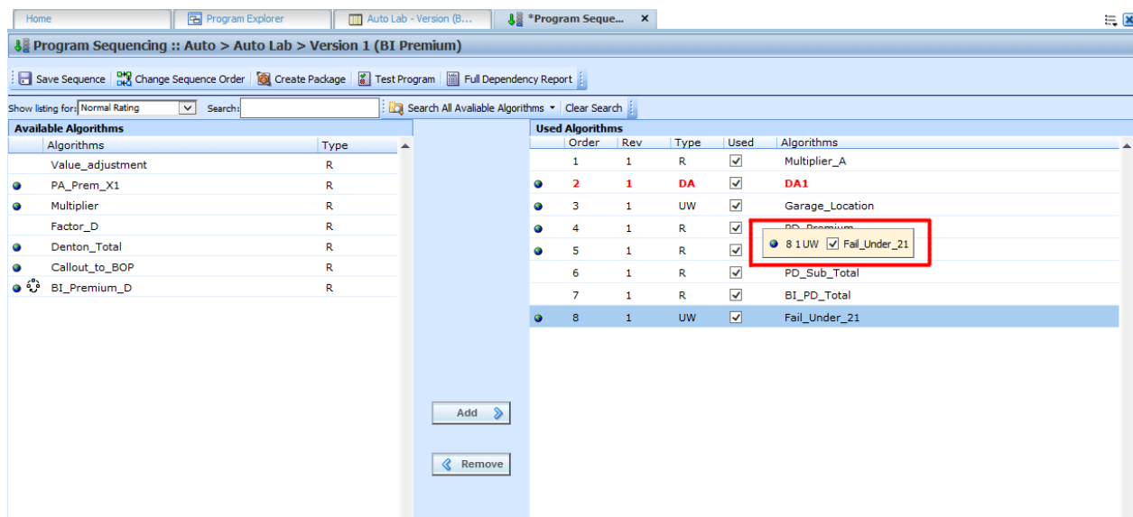
Figure 282 Changing Sequence Order Using Drop and Drag
