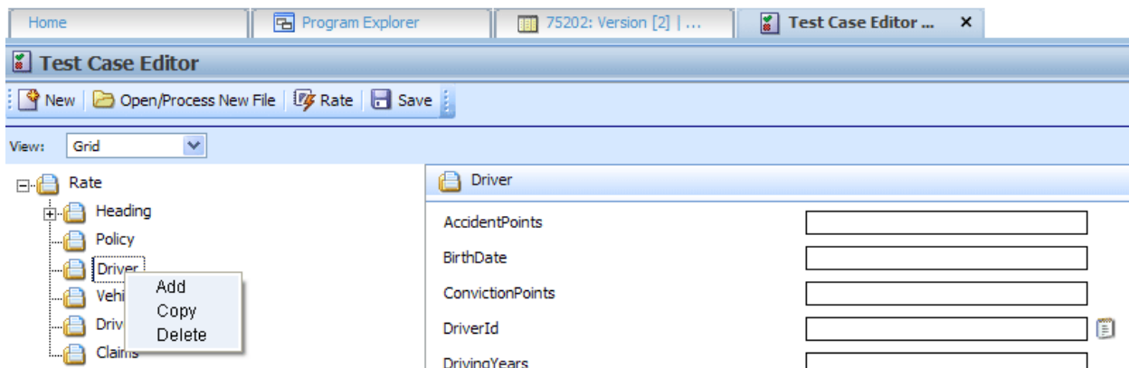
Figure 341 Right Click Menu for Test Case
