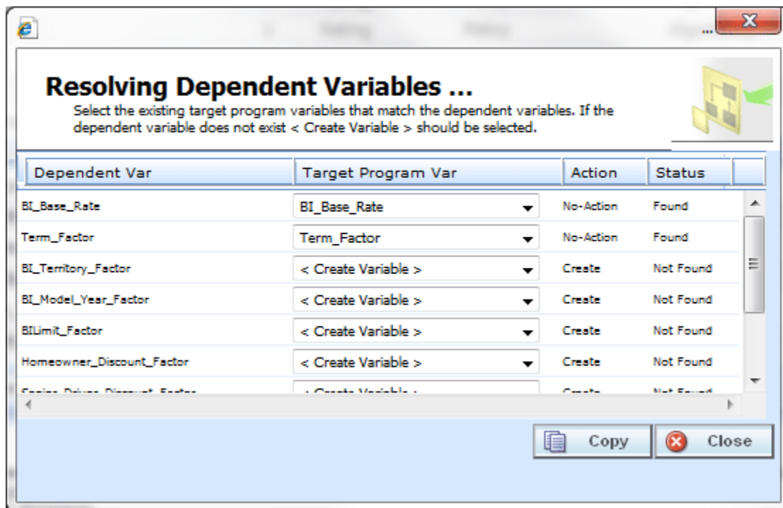
Figure 212 Resolving Dependent Variables
