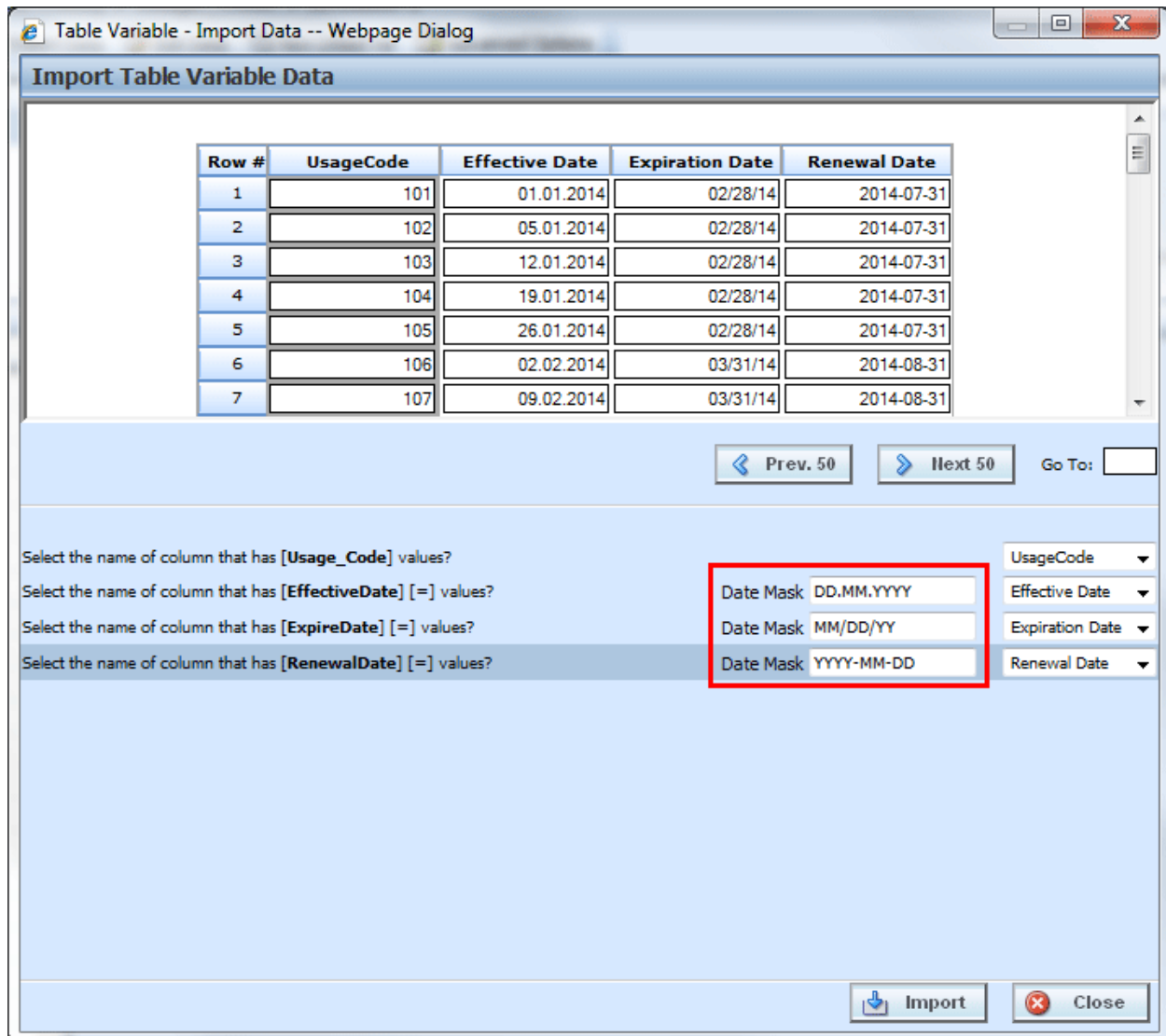
Figure 111 Previewing Data File with a Date Mask
