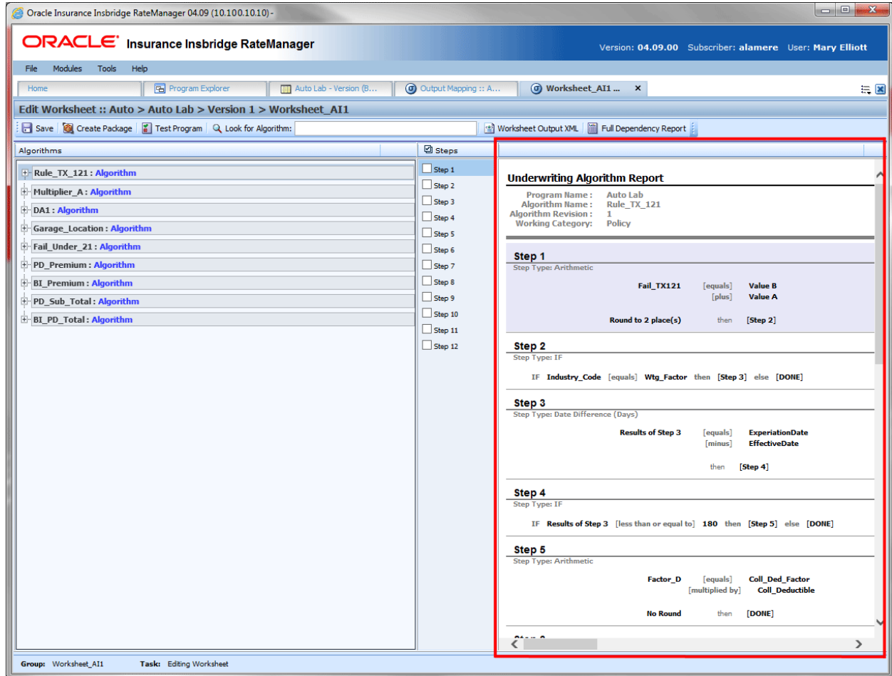
Figure 302 Edit Worksheet Report
