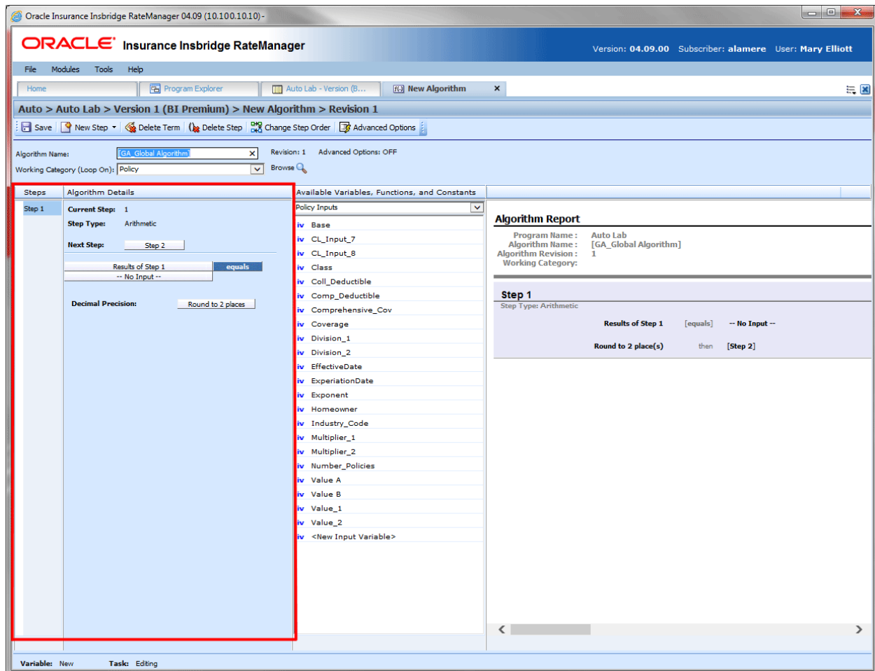
Figure 216 Algorithm Selection Criteria Field
