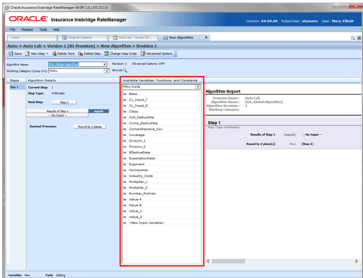
Figure 217 Available Variables, Function and Constants Field
