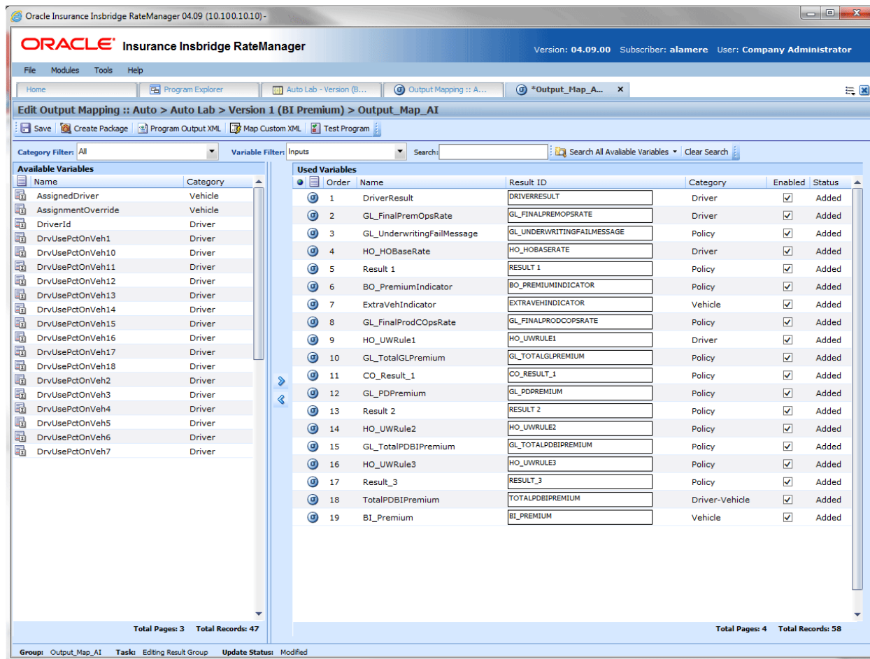
Figure 290 Editing an Output Group Mapping
