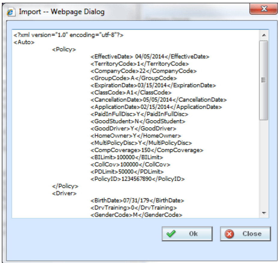
Figure 318 Import Custom XML Text Box
