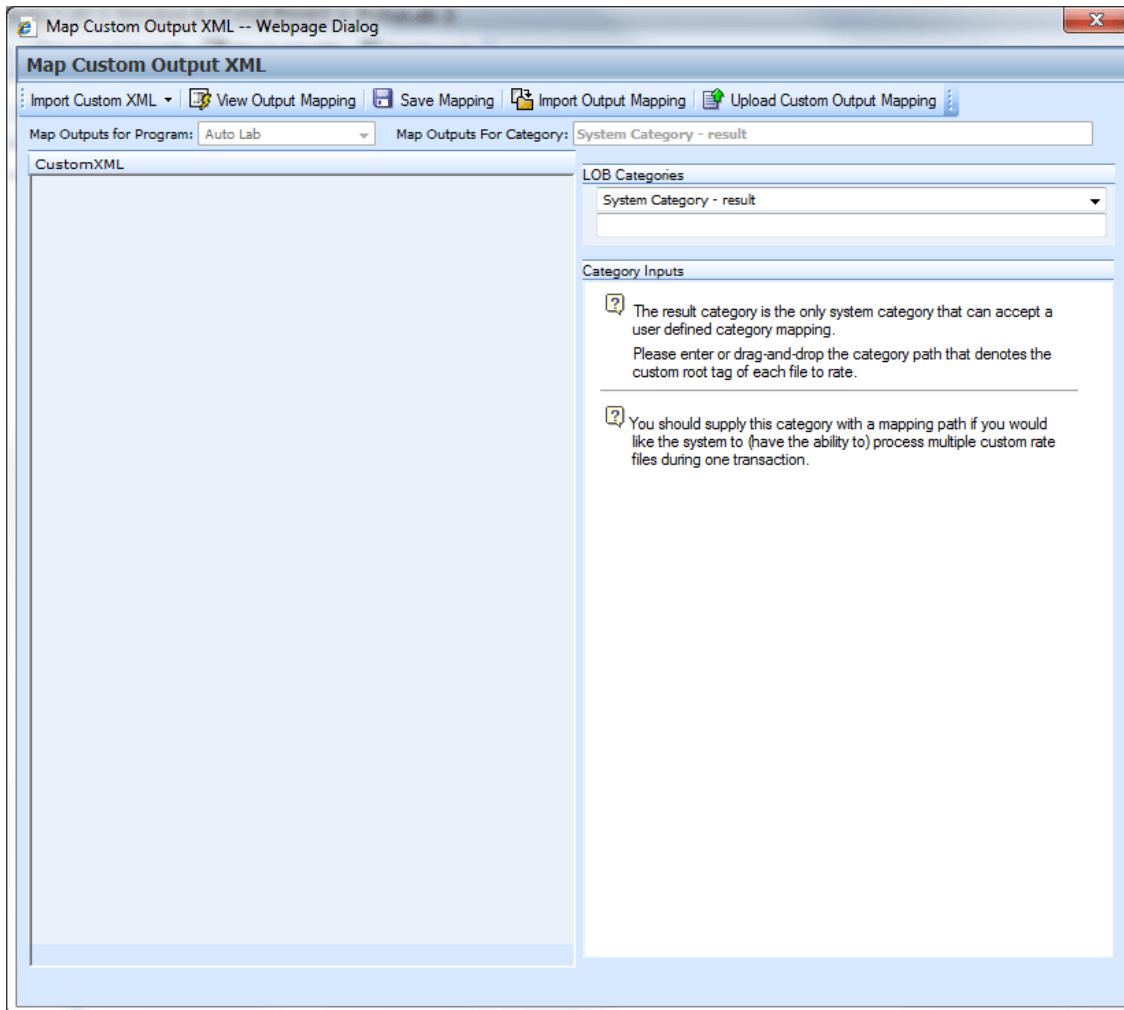
Figure 331 Mapping Custom Output XML
