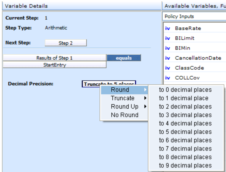
Figure 126 Setting the Rounding Option
