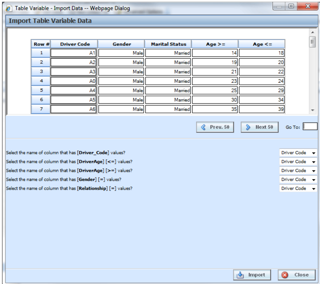
Figure 107 Previewing Data File
