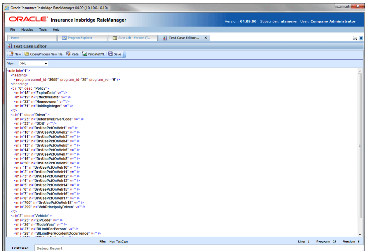
Figure 345 Test Case XML View
