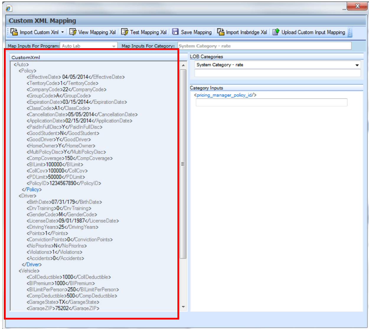
Figure 314 Custom XML Work Area
