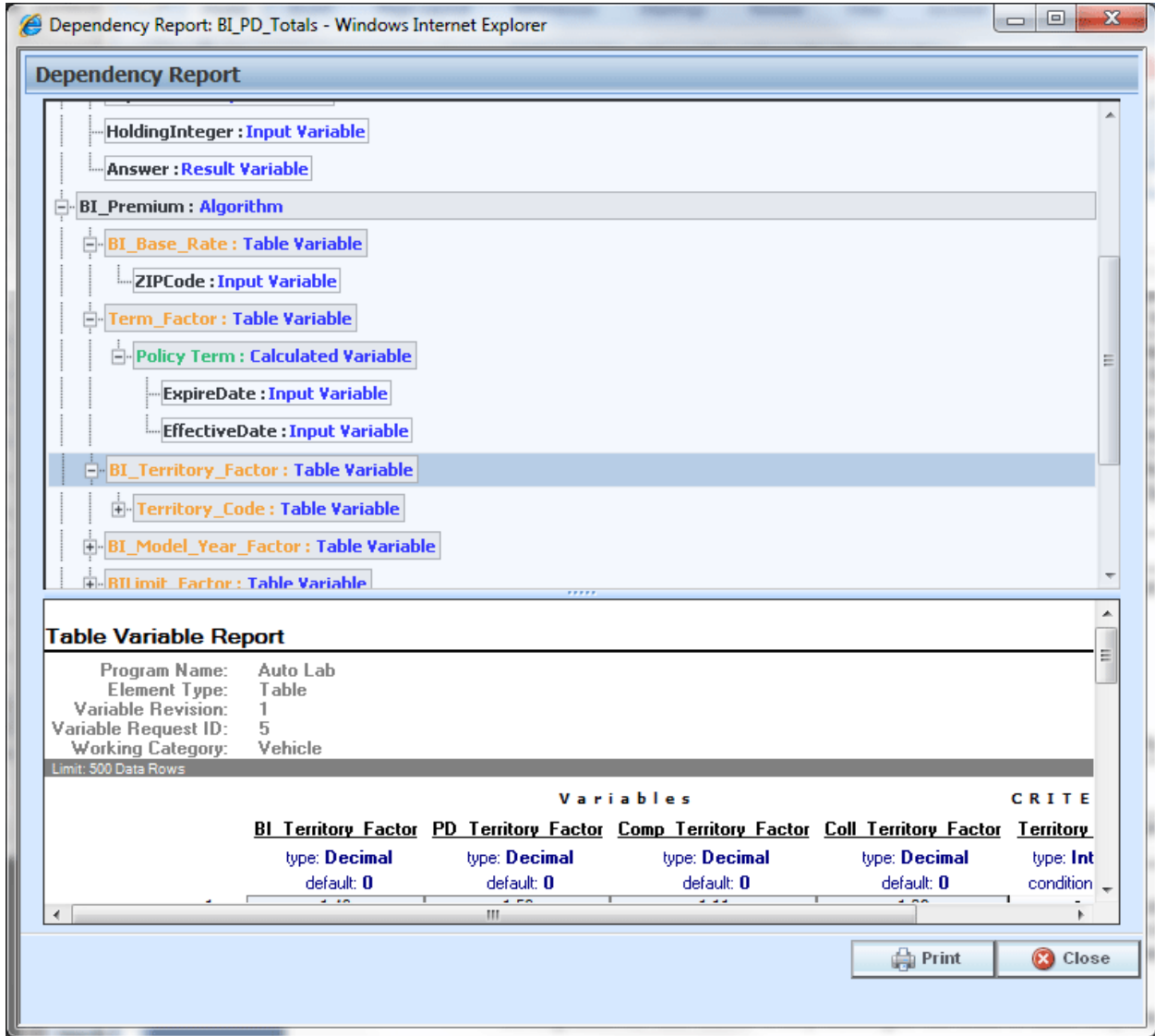
Figure 366 Full Dependency Report
