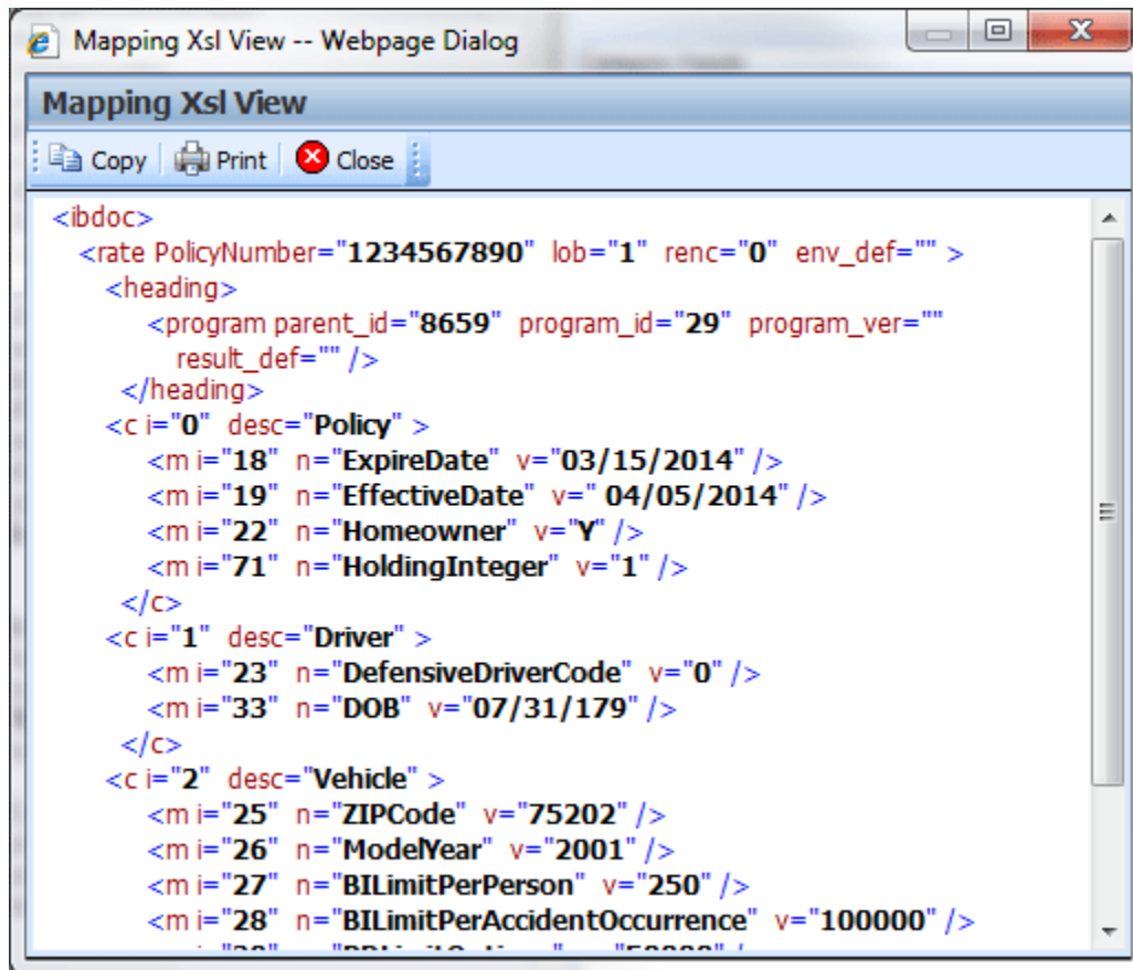
Figure 326 Test Mapping Xsl
