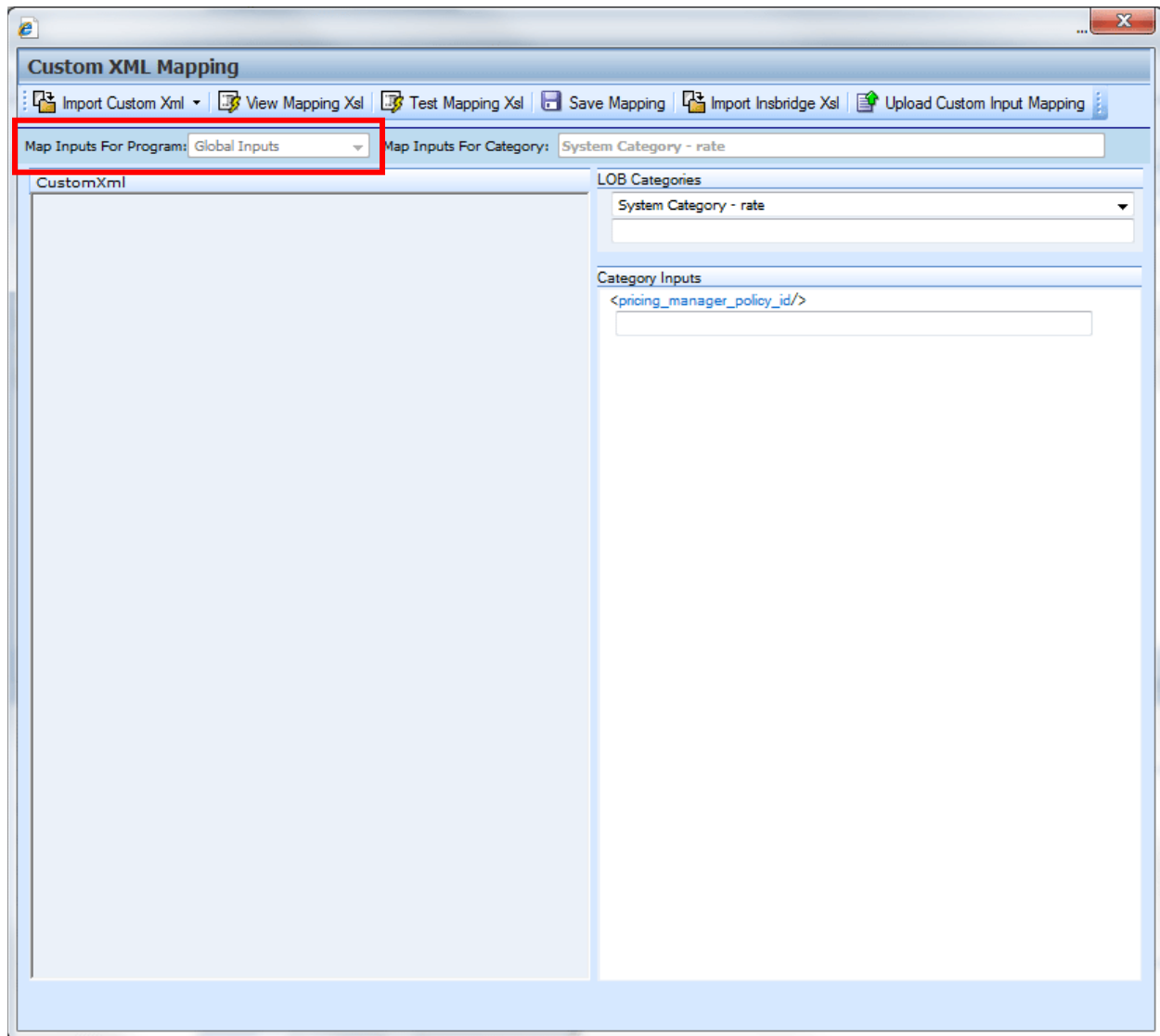
Figure 312 Custom XML Mapping at Global Level
