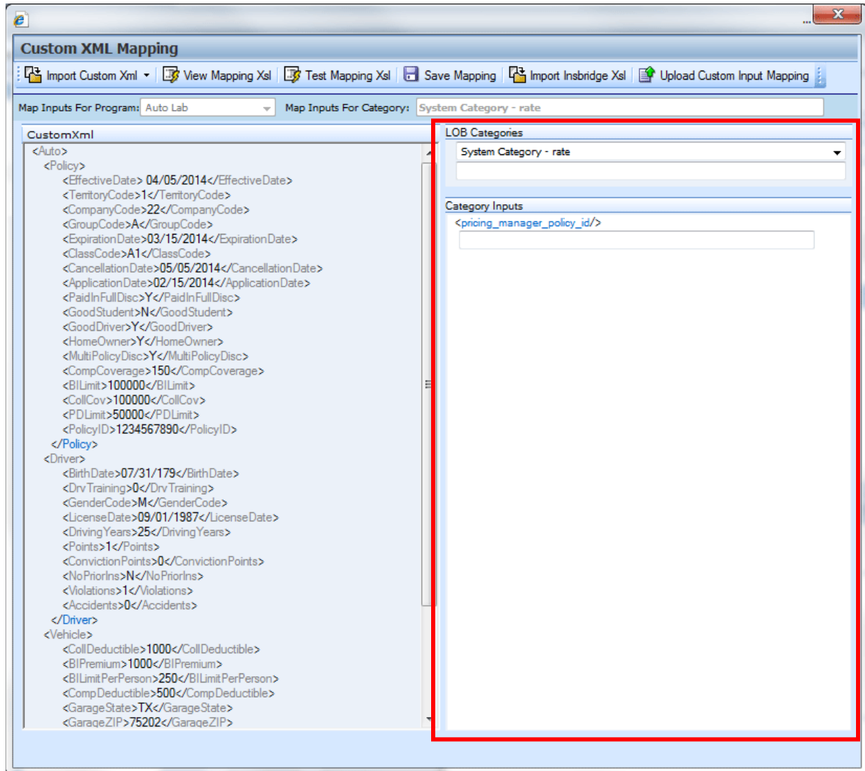
Figure 315 Category Inputs Work Area
