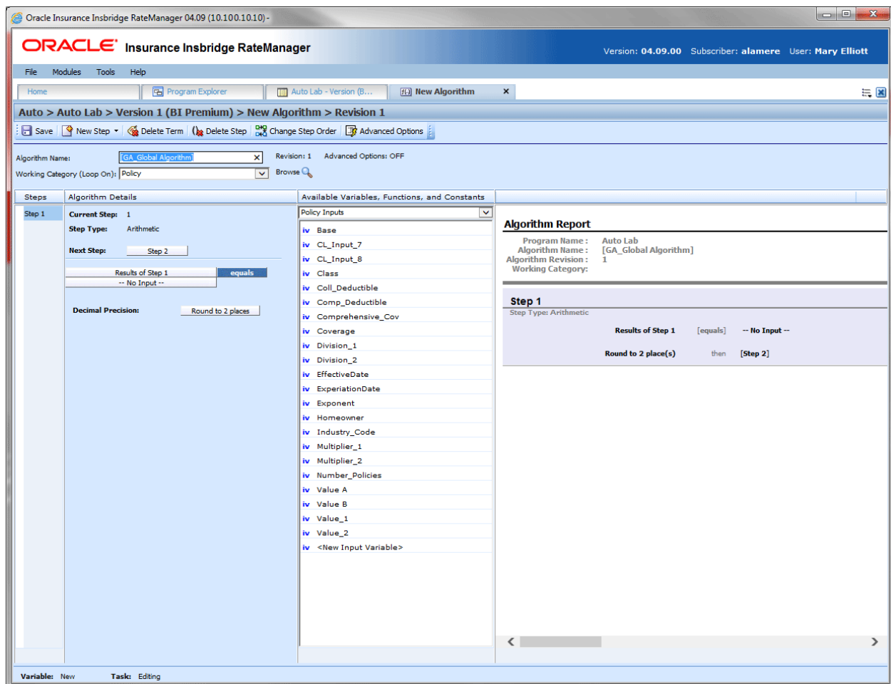
Figure 219 Creating a New Algorithm
