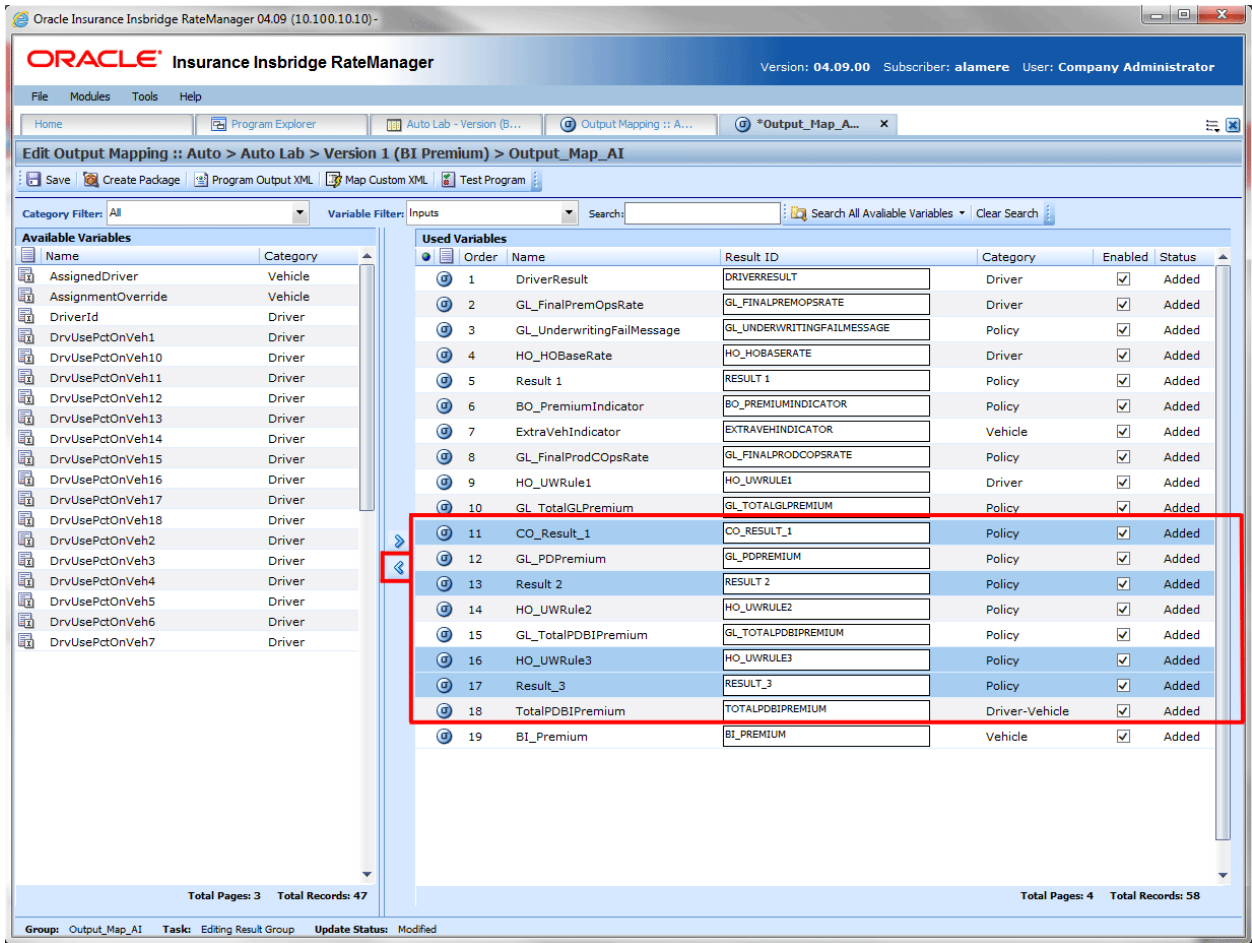
Figure 291 Multiple Selections to Create an Output Mapping
