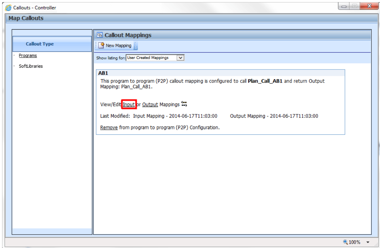
Figure 259 Edit Inputs
