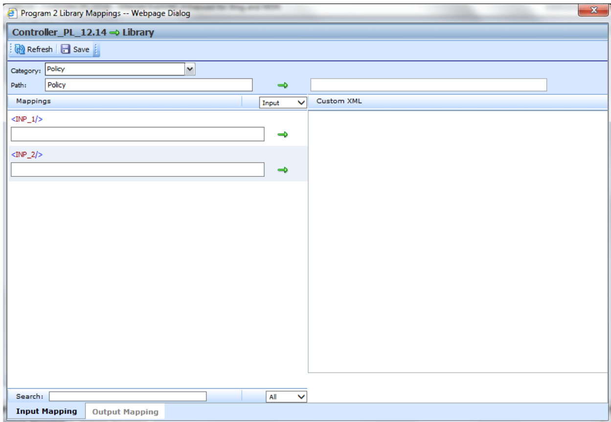
Figure 266 Adding Exceptions
