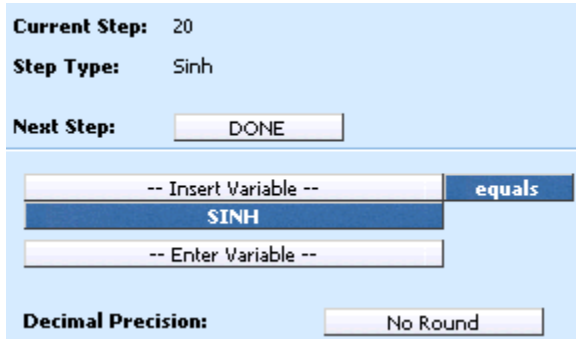
Figure 178 Sinh Step
