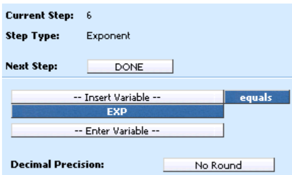
Figure 165 Exponent Step
