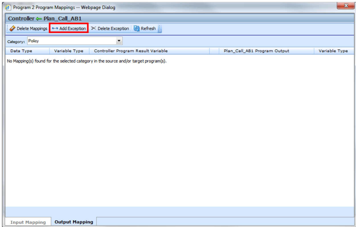
Figure 260 Adding Exceptions
