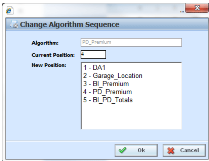
Figure 281 Change Sequence
