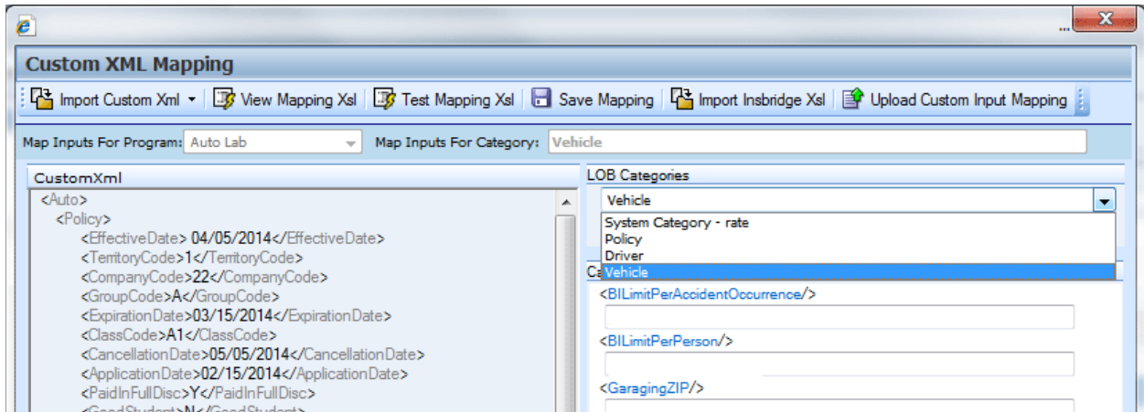
Figure 322 Selecting Categories
