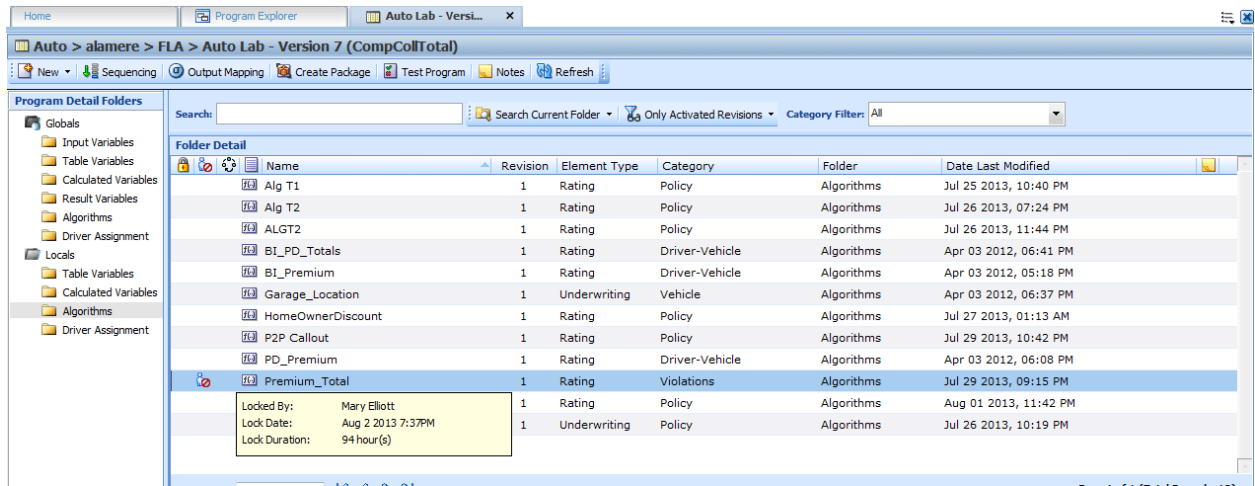
Figure 379 In-Use Message
