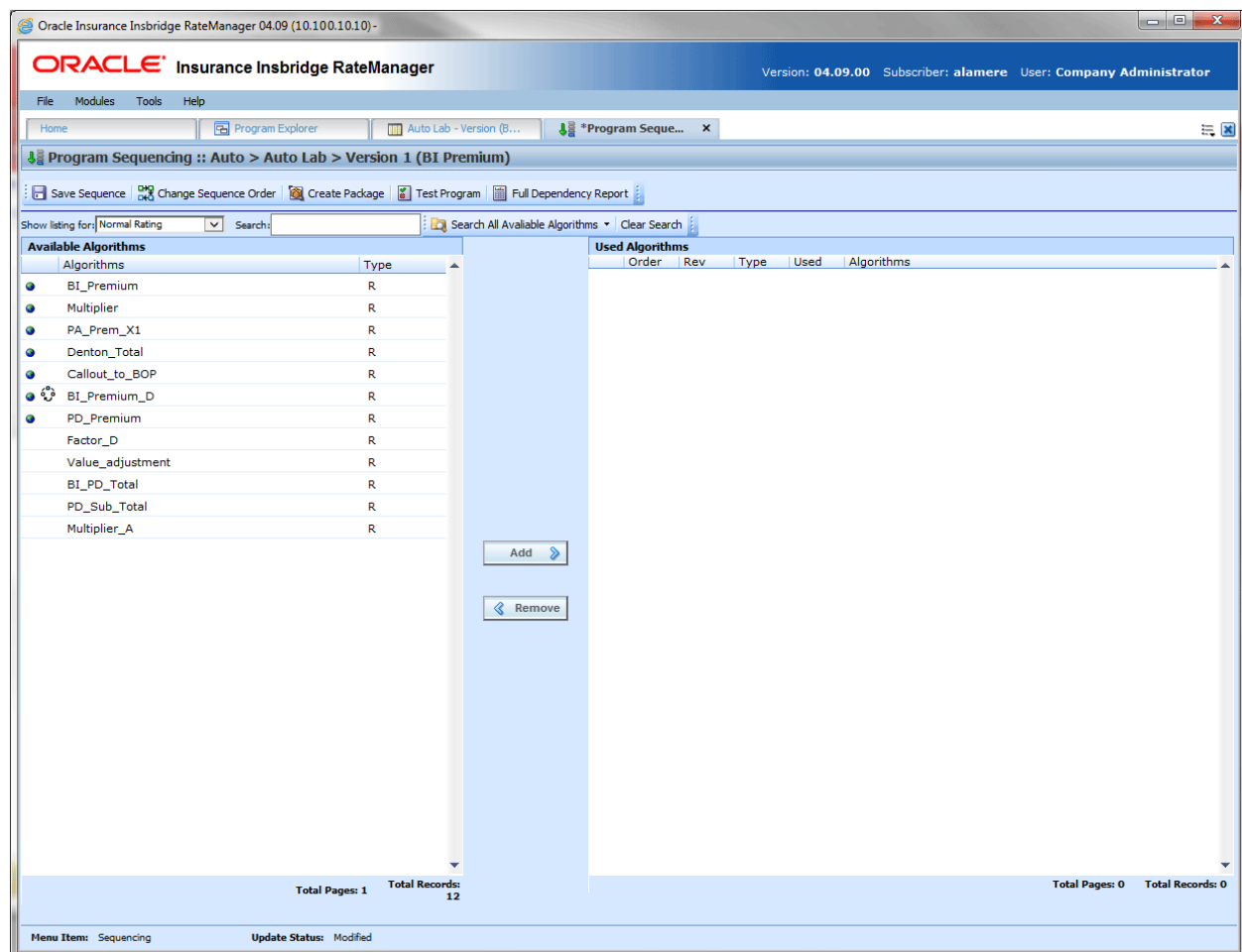
Figure 277 Sequencing Tab
