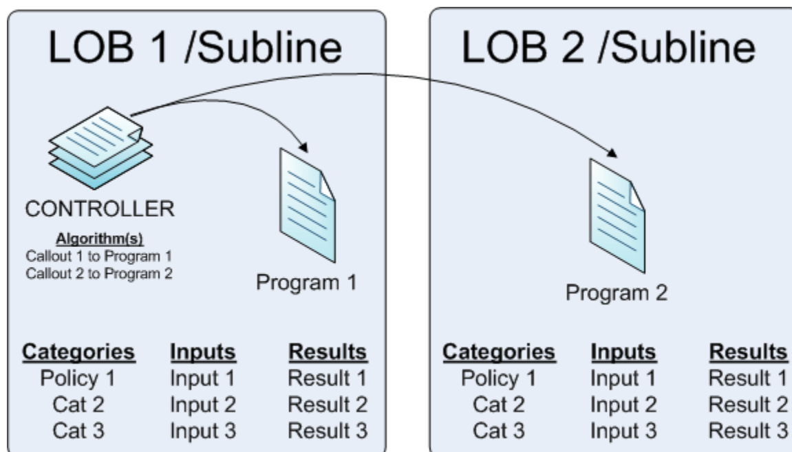
Figure 255 Crossline P2P
