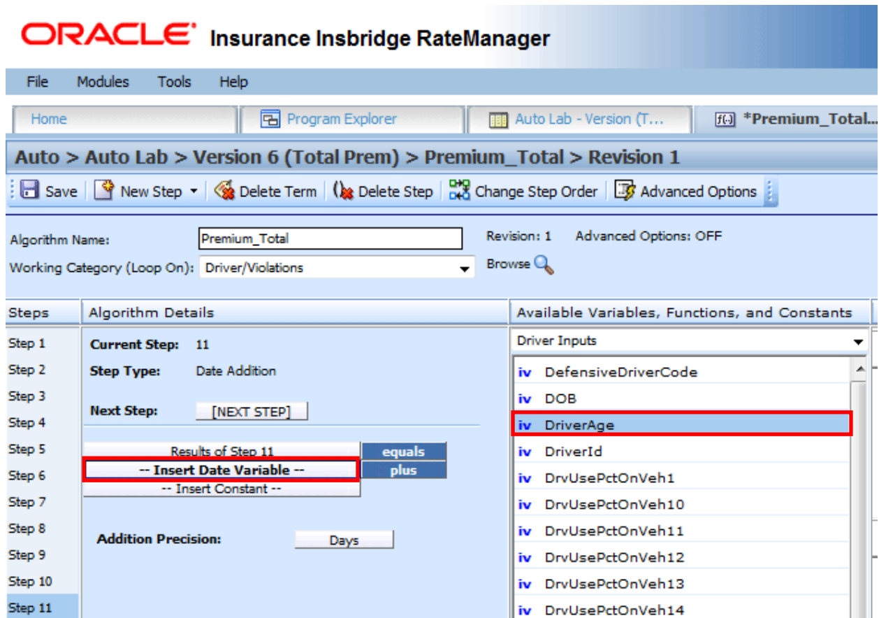
Figure 123 Editing Steps
