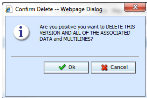
Figure 48 Confirming Delete
