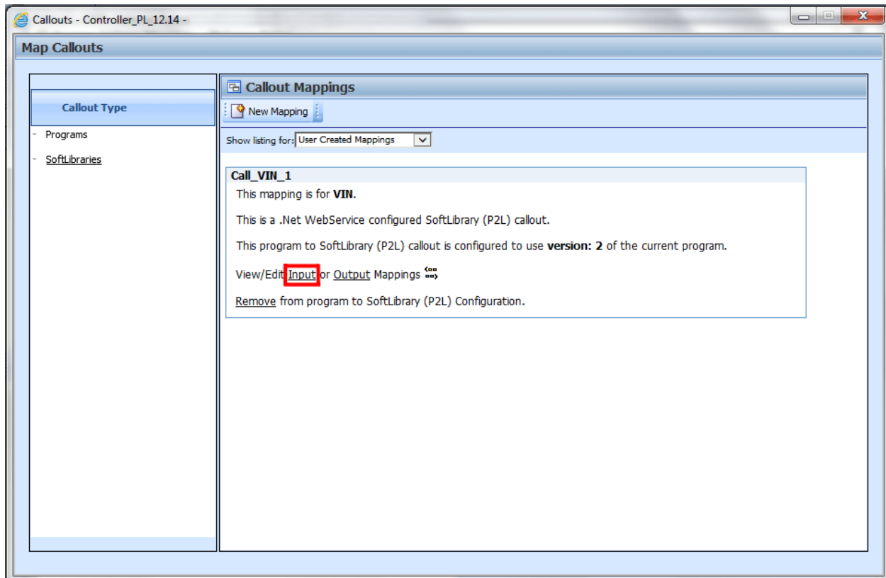
Figure 265 Edit Inputs
