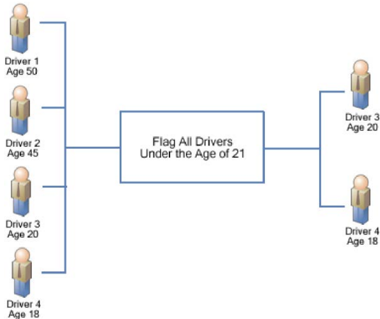
Figure 237 Flagging Functions
