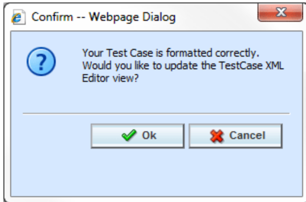
Figure 346 XML Validation
