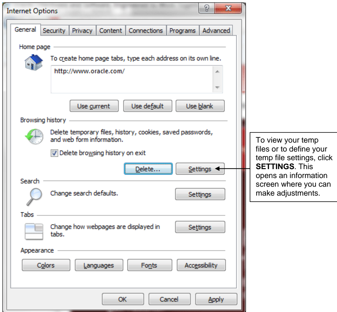
Figure 398 Delete Files
