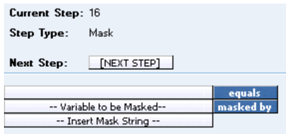
Figure 155 Mask Step
