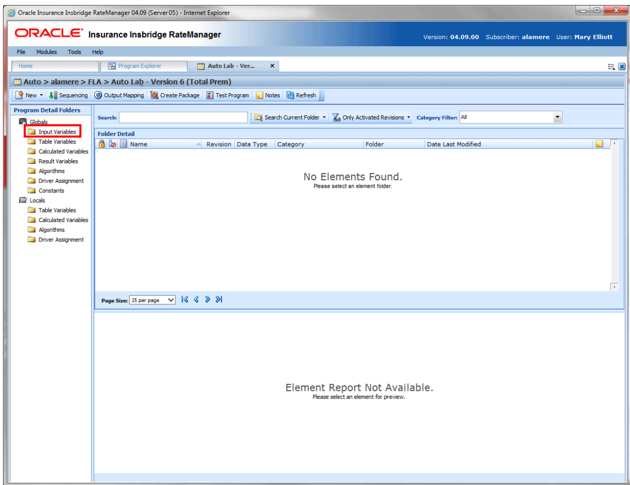
Figure 74 Selecting Inputs
