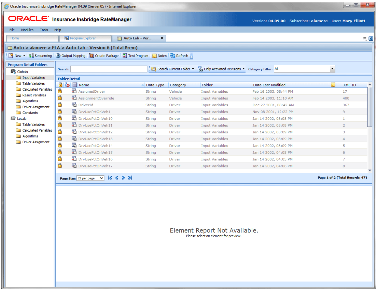
Figure 75 Input Listing
