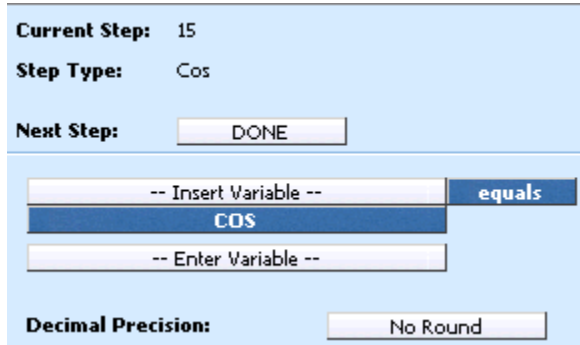
Figure 173 Cosine Step
