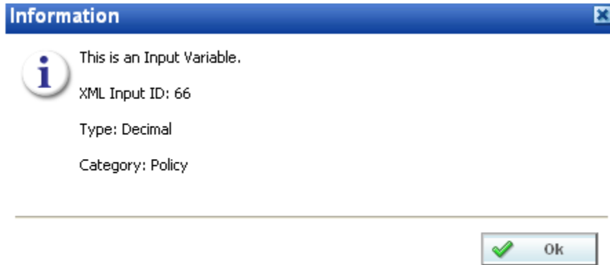
Figure 372 View Report
