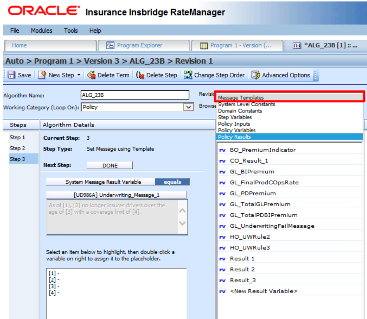
Figure 224 Message Templates
