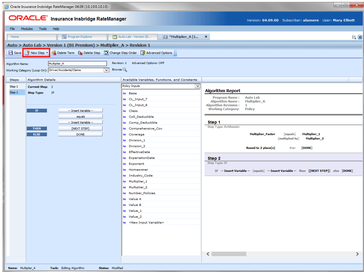
Figure 151 Creating a Simple IF Statement
