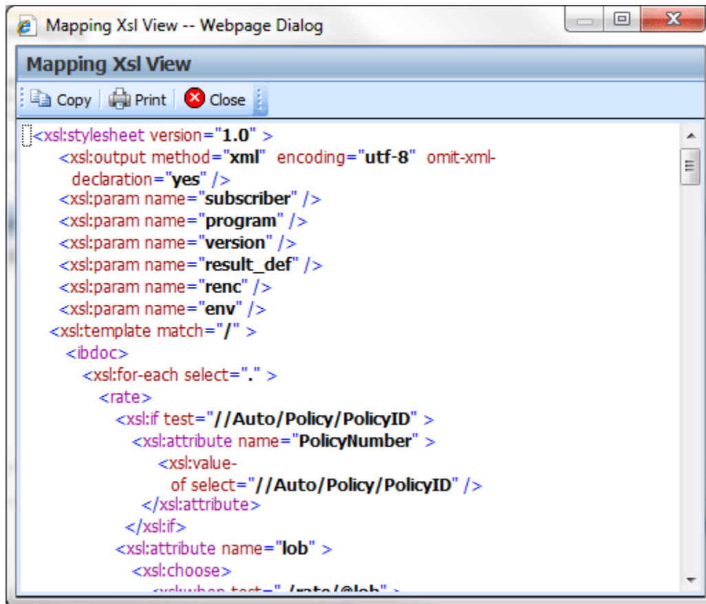
Figure 325 View Mappings Xsl
