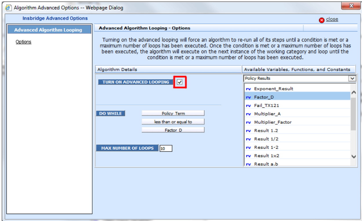
Figure 221 Algorithm Advanced Options
