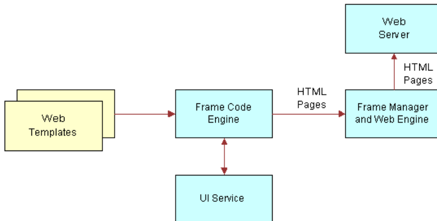
Figure 12. Web Template Processing
