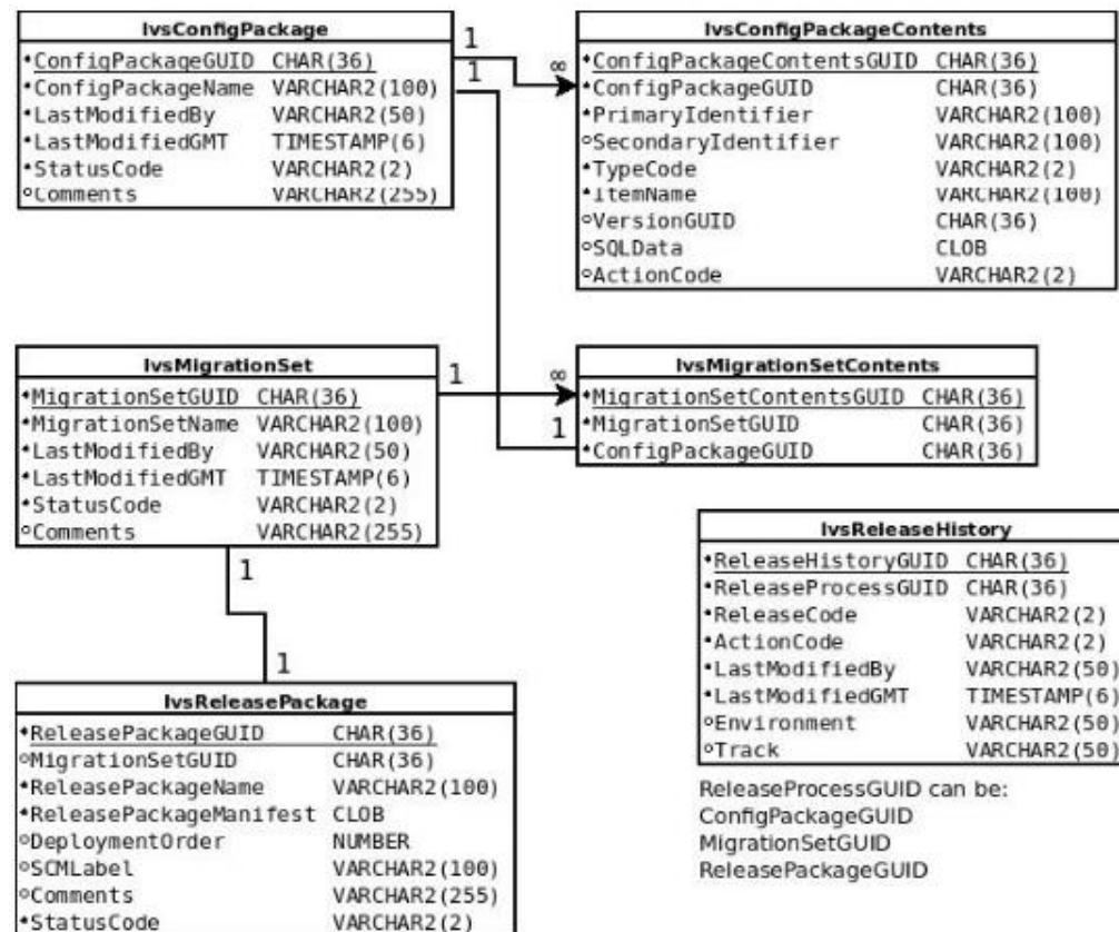
Figure 4: Release Management Table Structure
