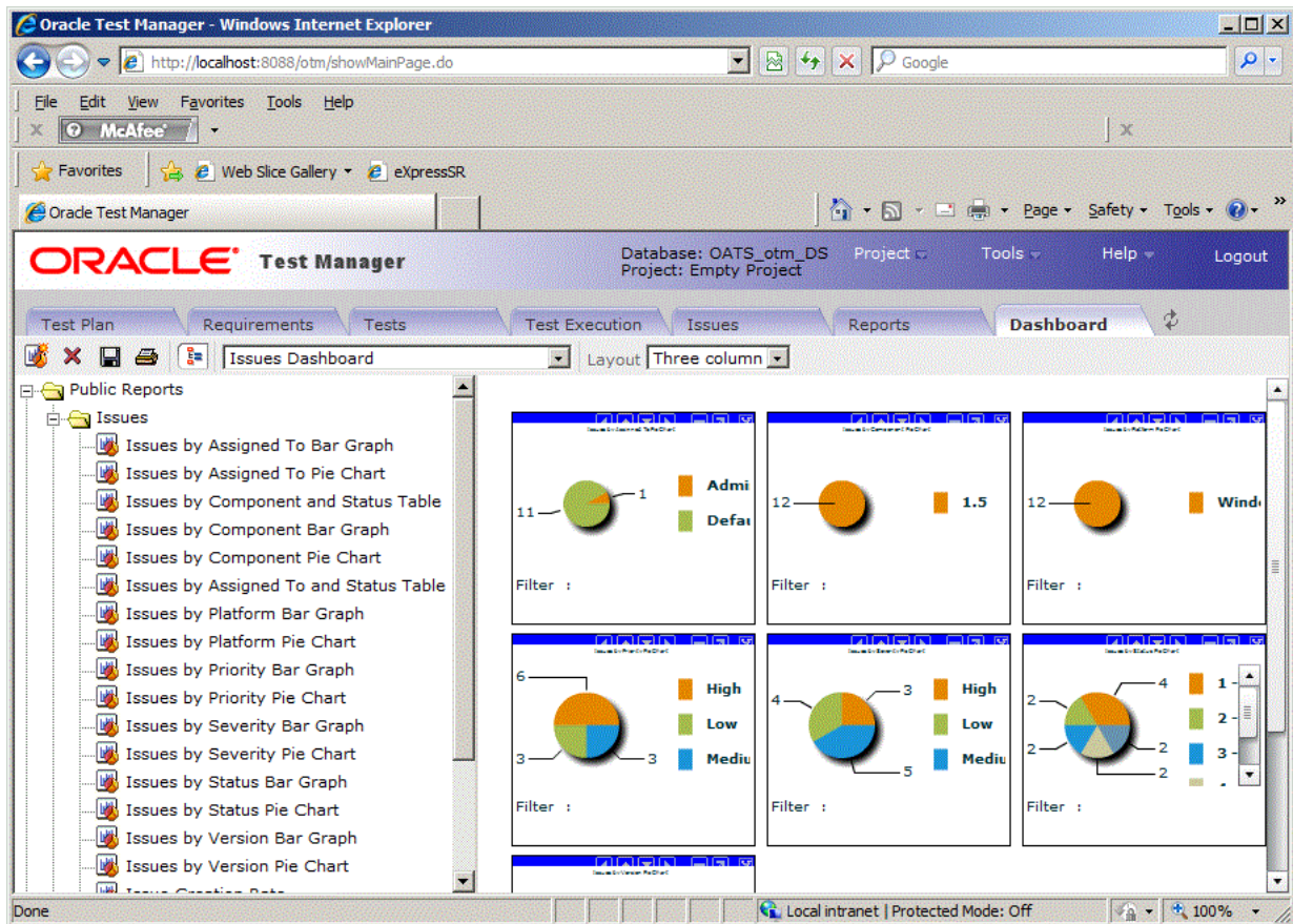
Figure 2–31 Dashboard Tab
