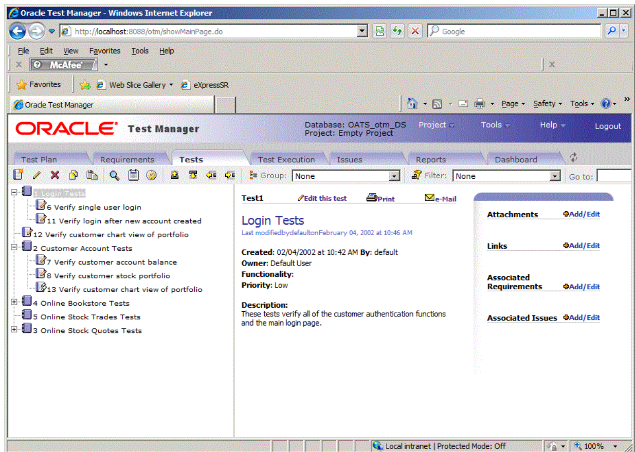
Figure 2–27 Tests Tab
