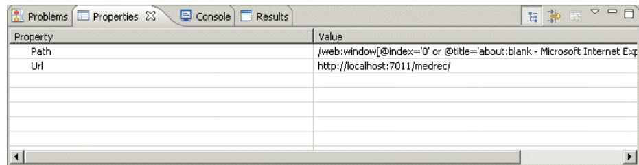
Figure 2–15 Properties View
