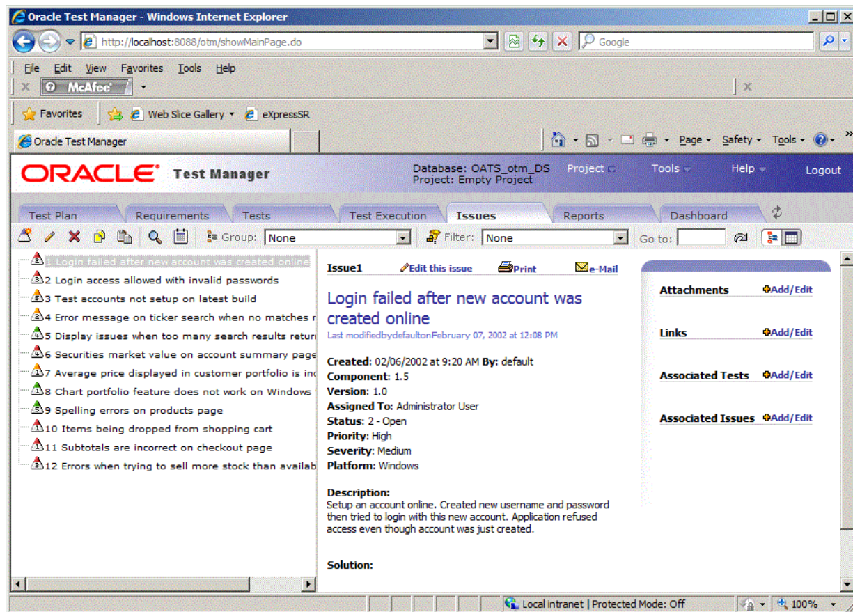
Figure 2–28 Issues Tab
