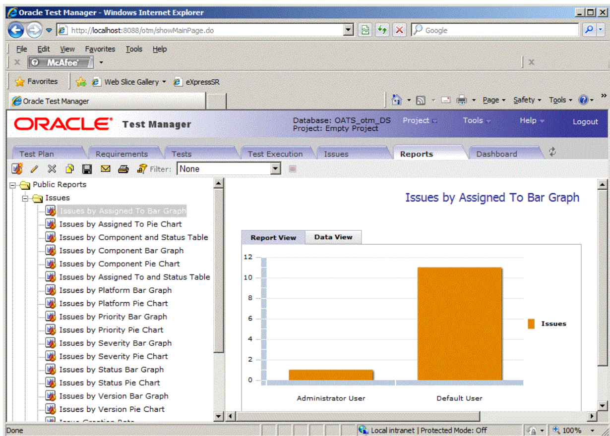
Figure 2–29 Reports Tab
