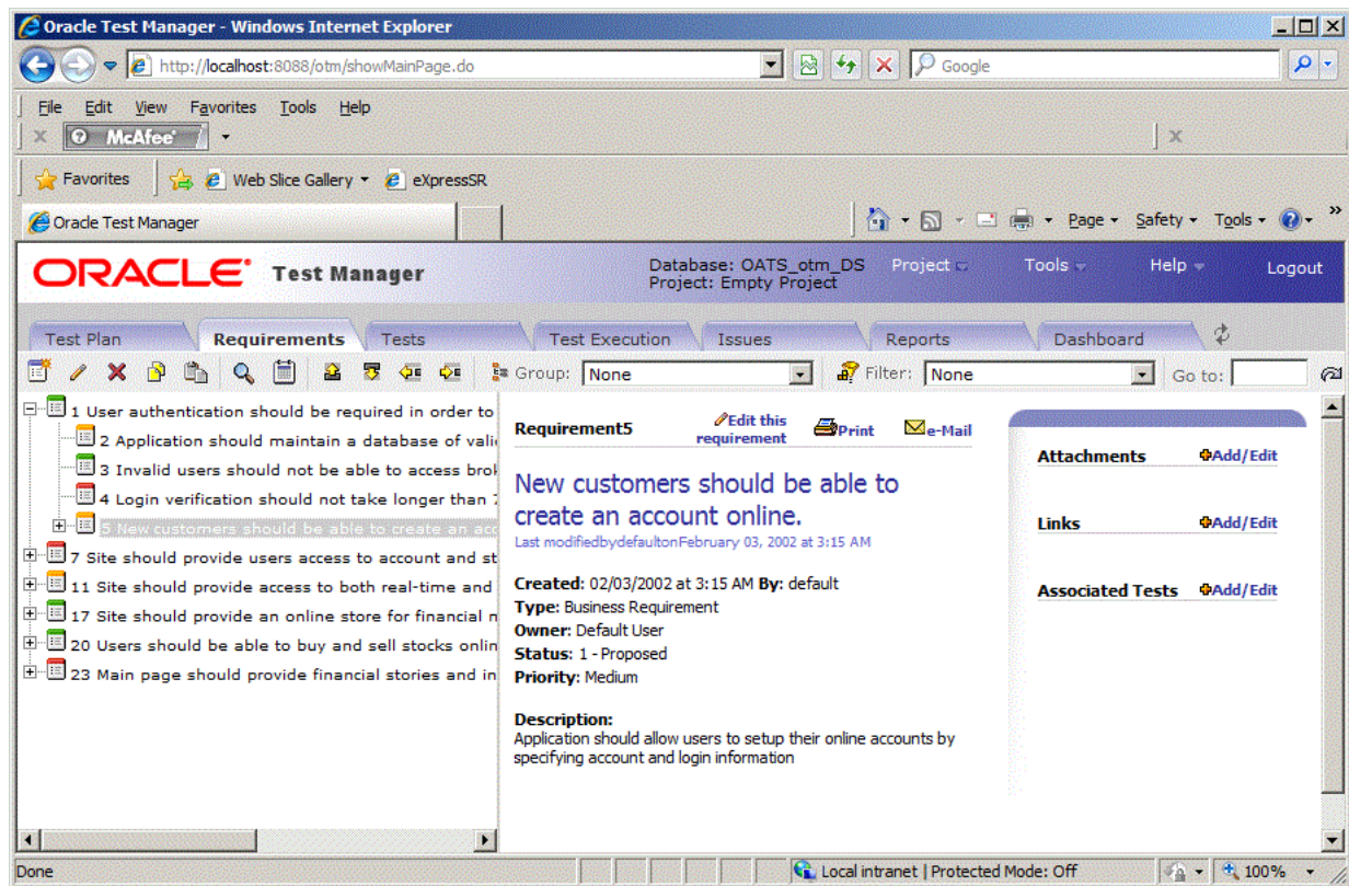
Figure 5-7 Requirements Tab
