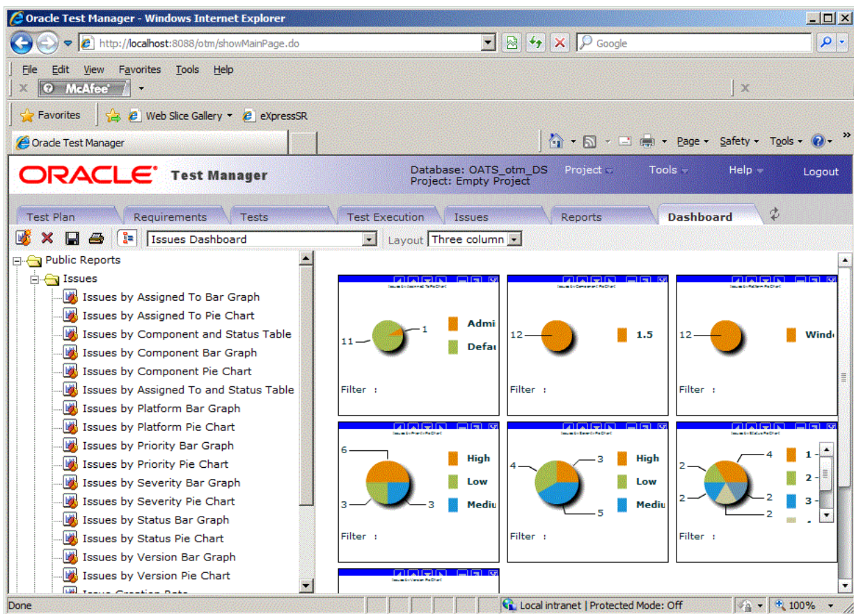
Figure 2–30 Dashboard Tab
