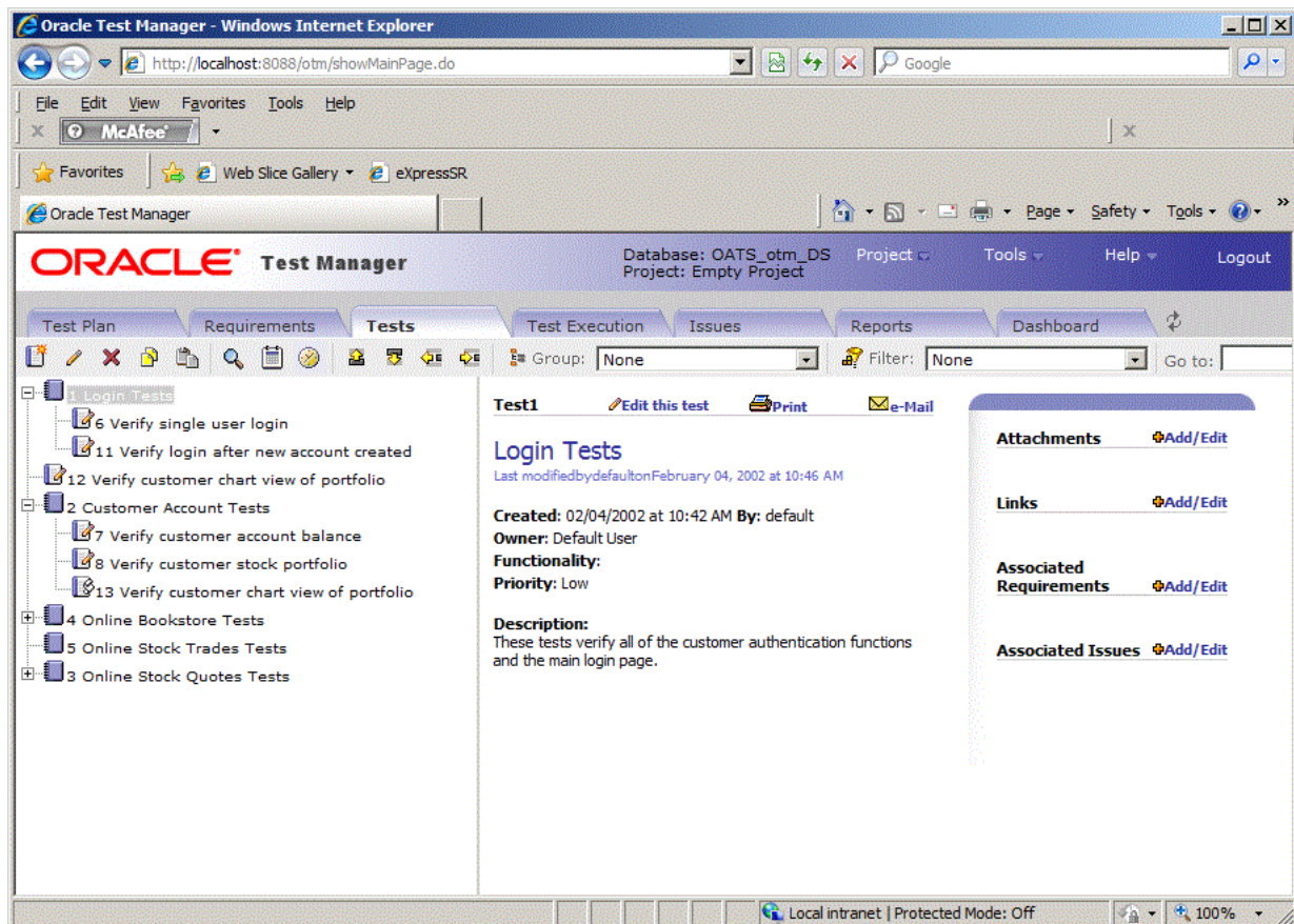
Figure 2–26 Tests Tab
