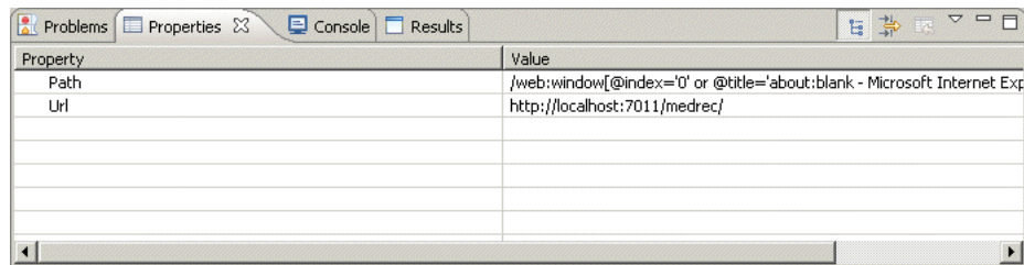
Figure 2–14 Properties View
