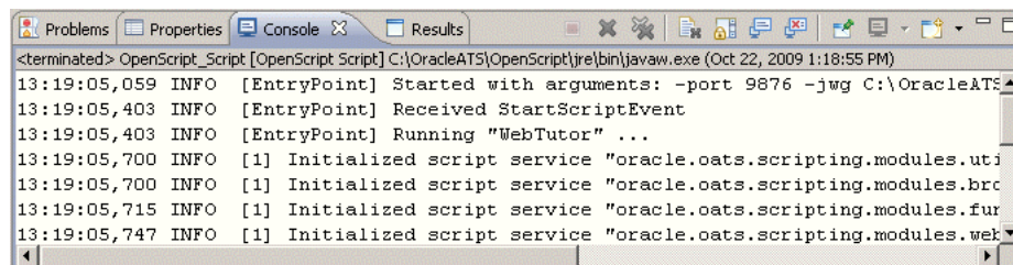
Figure 2–15 Console View
