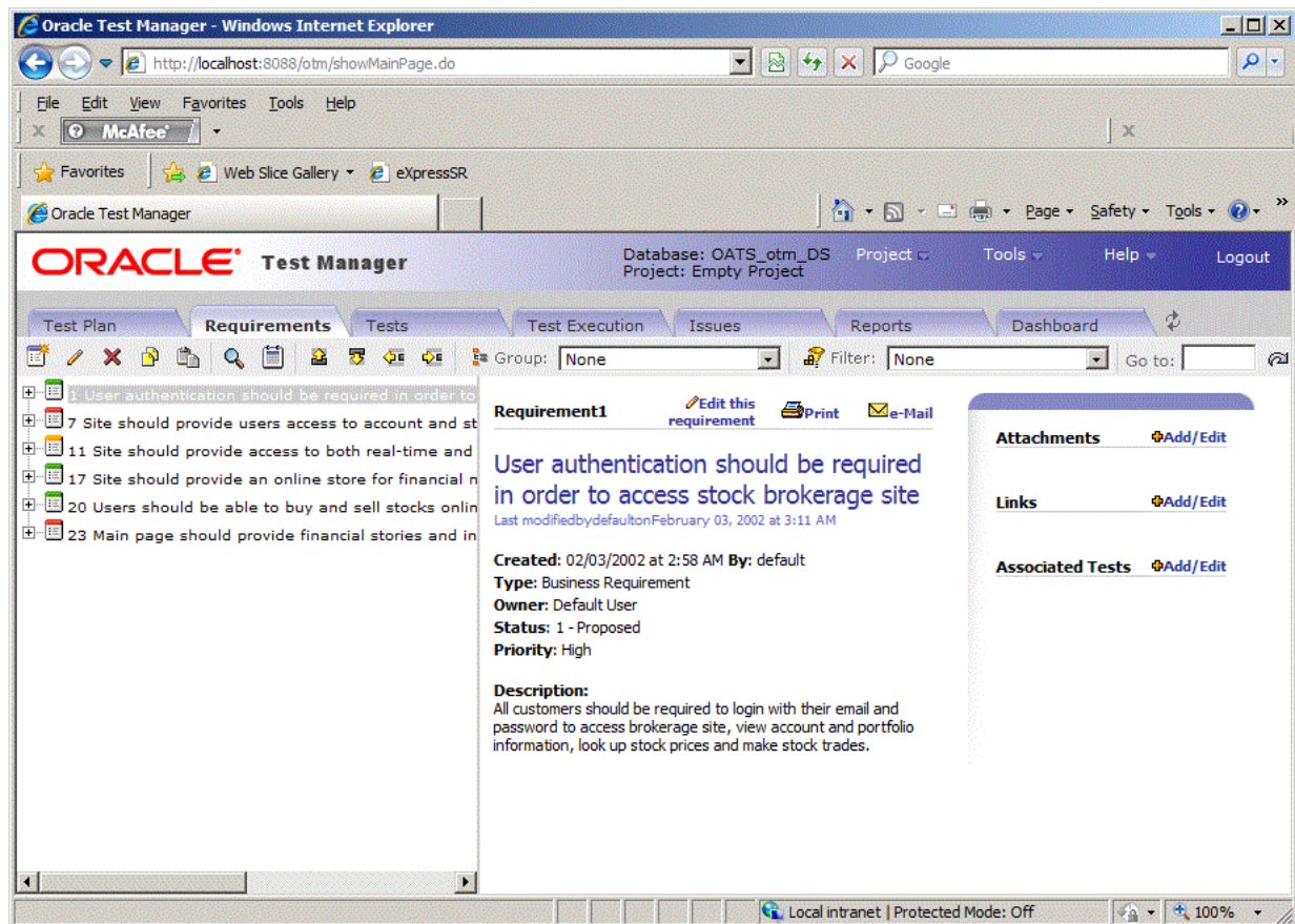
Figure 2-25 Requirements Tab
