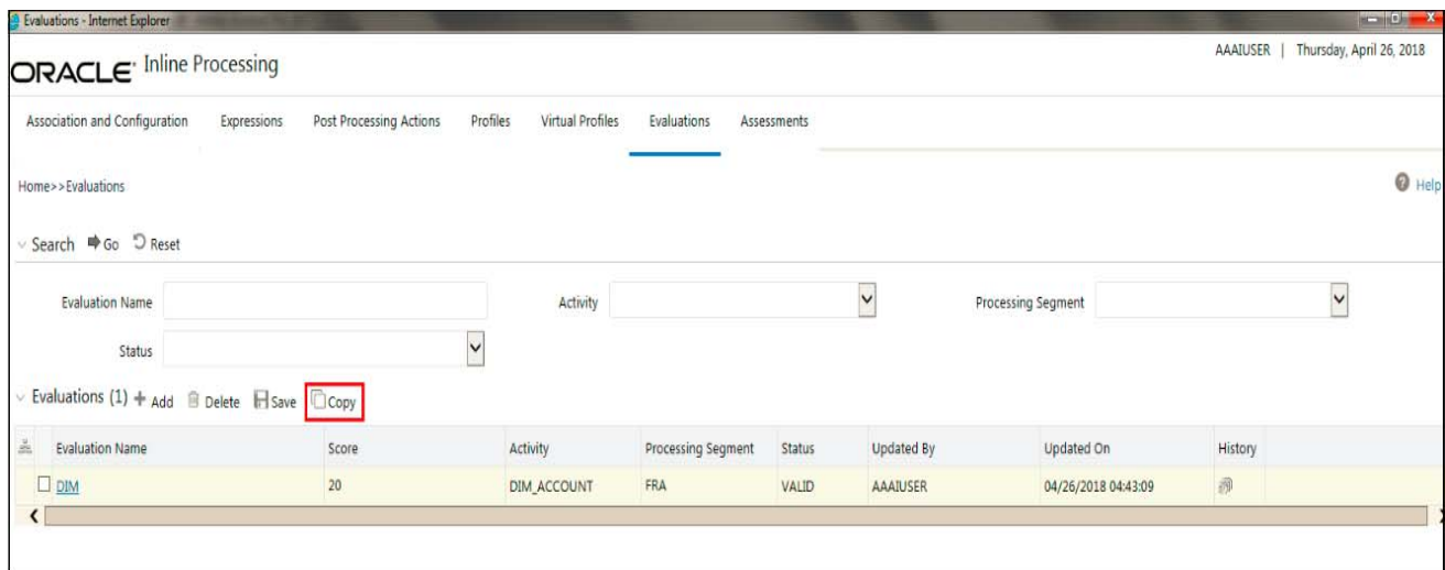
Figure 38. Copying Evaluation
