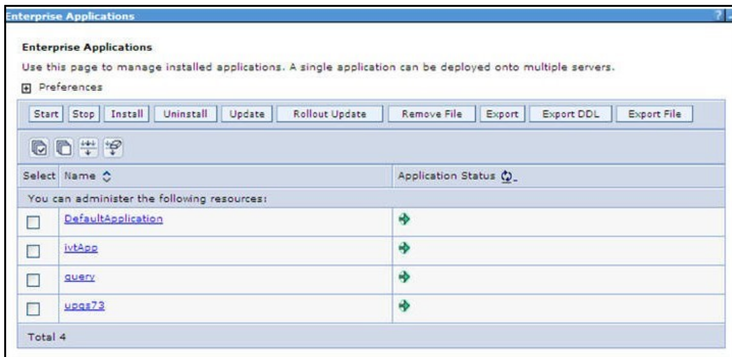
Figure 5–13 Enterprise Applications
