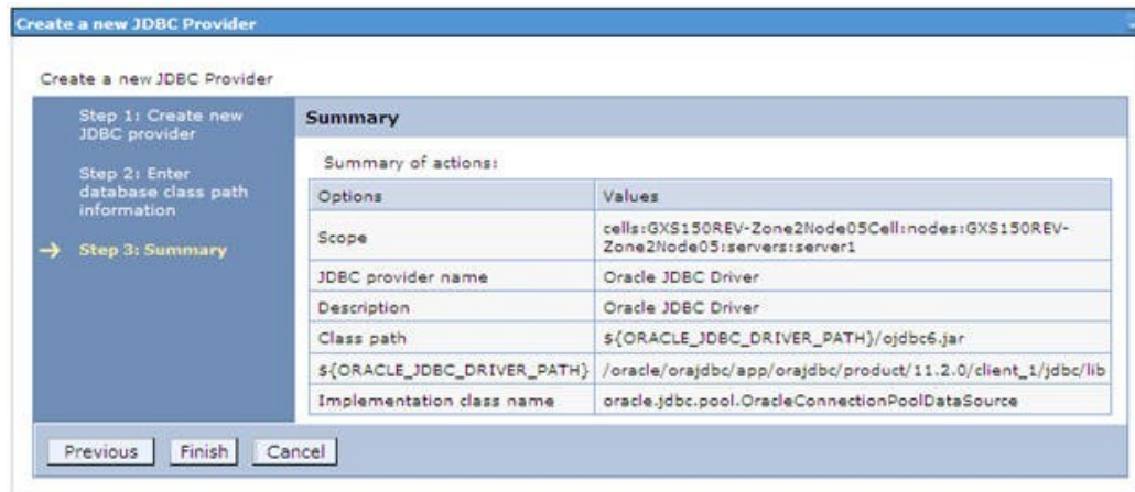
Figure 5–2 Summary
