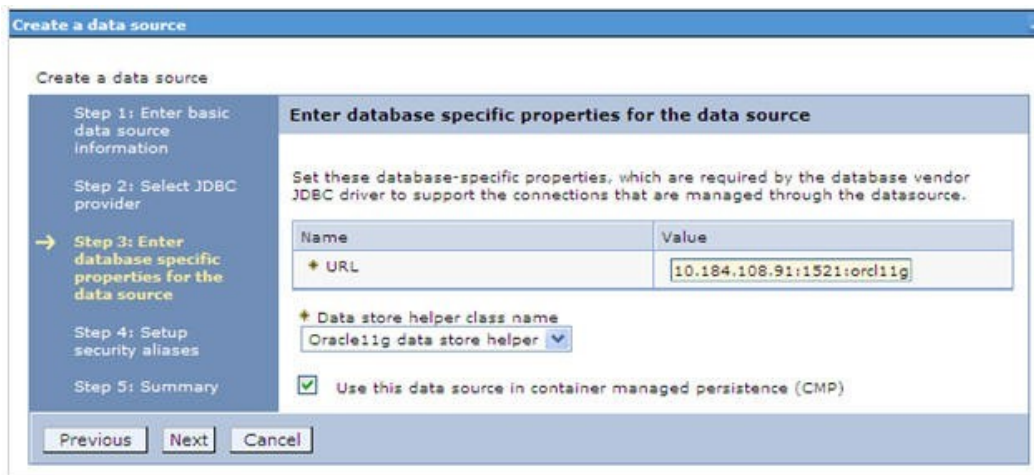
Figure C-5 Enter Database specific properties
