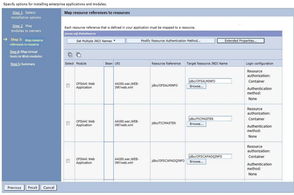
Figure D-8 Map Resource References to Resources
