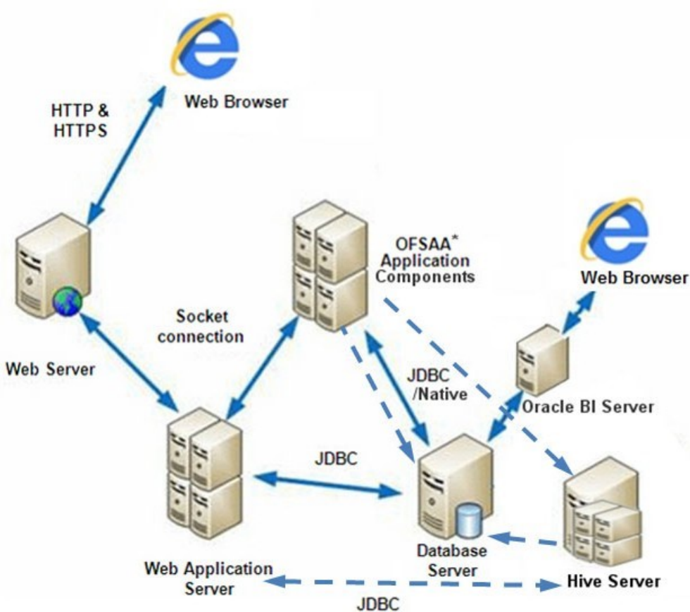
Figure 2-2 Deployment Topology
