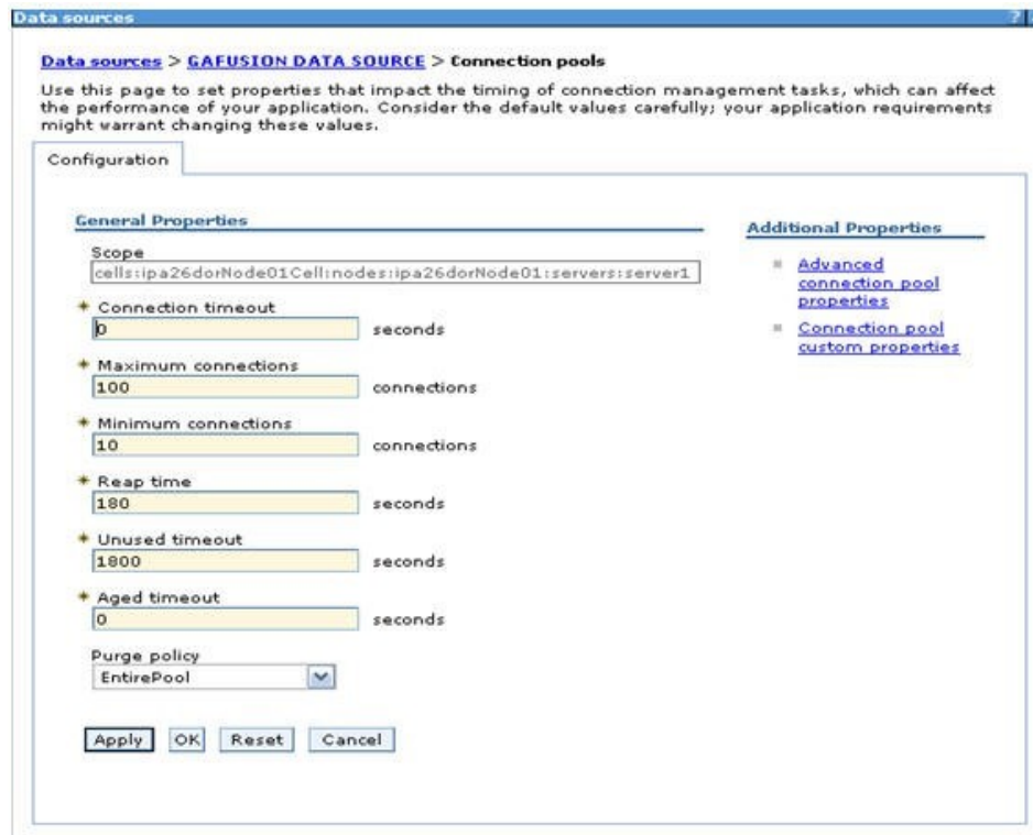
Figure C–8 Connection pools
