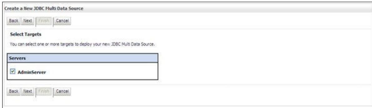
Figure 5–8 Select Targets
