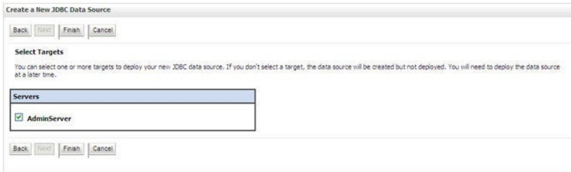
Figure C–15 Select Targets
