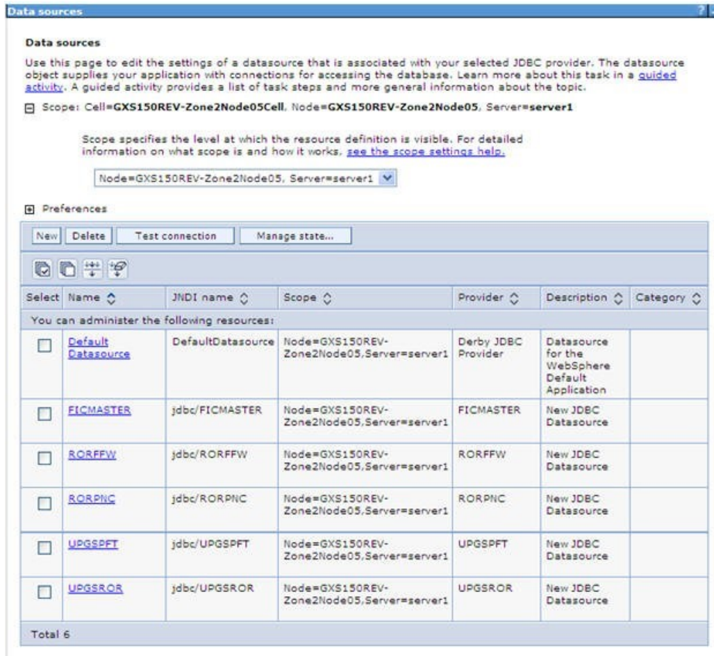
Figure C-1 Data Sources
