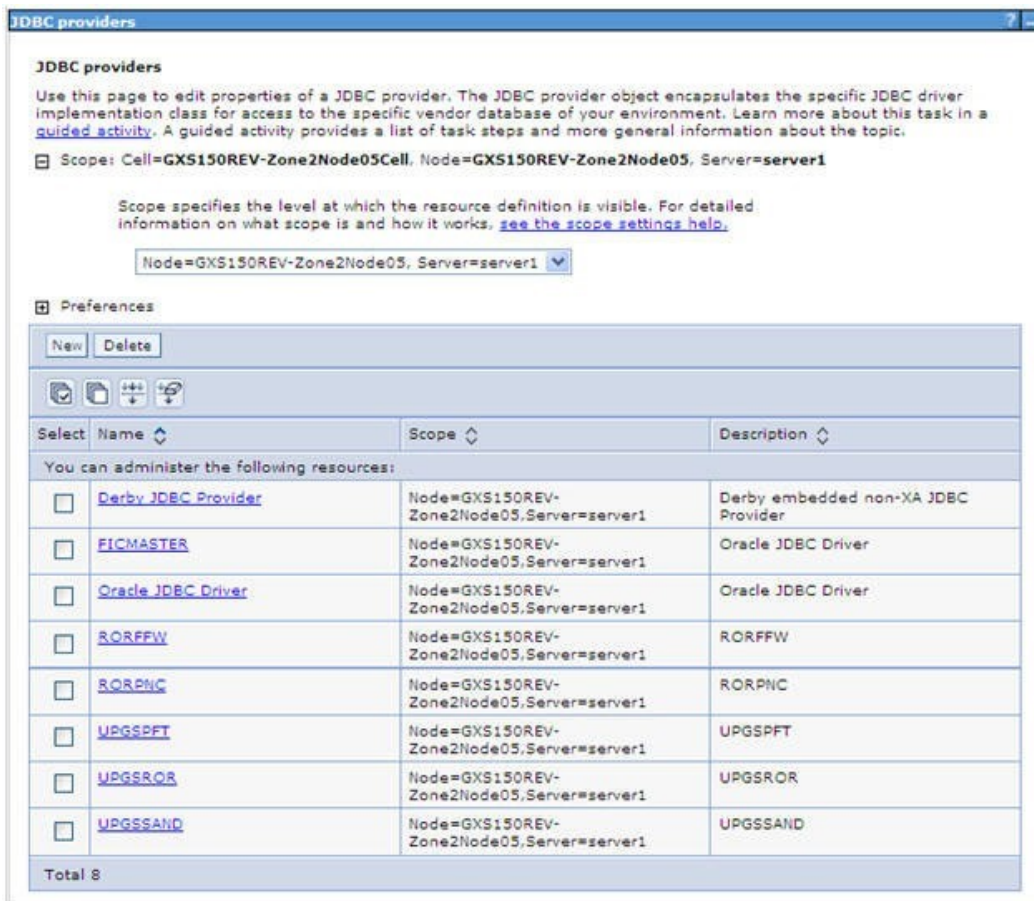
Figure 5–1 JDBC Providers
