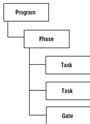
Figure 19–1 Program hierarchy
