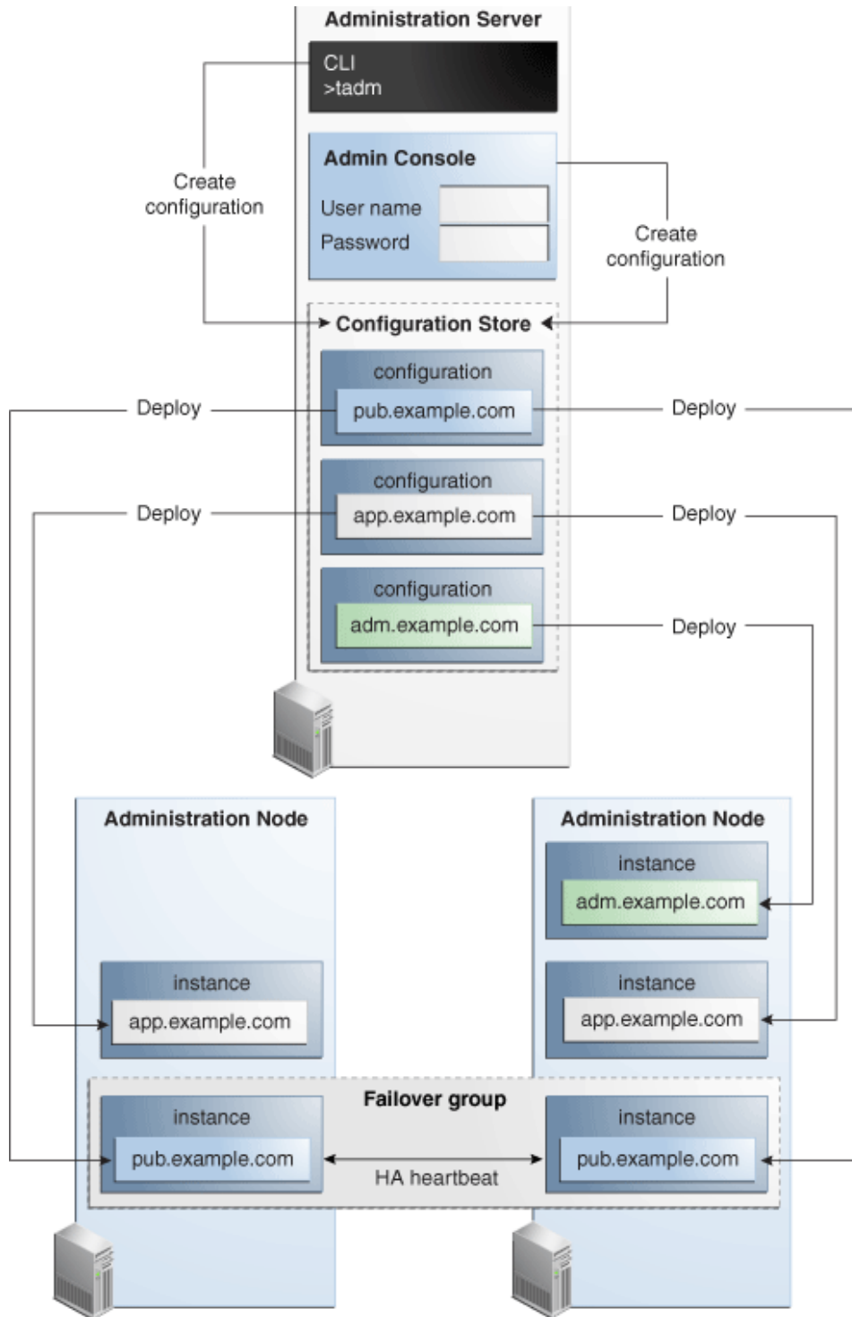
Figure 1-1 Administration Framework of Oracle Traffic Director
