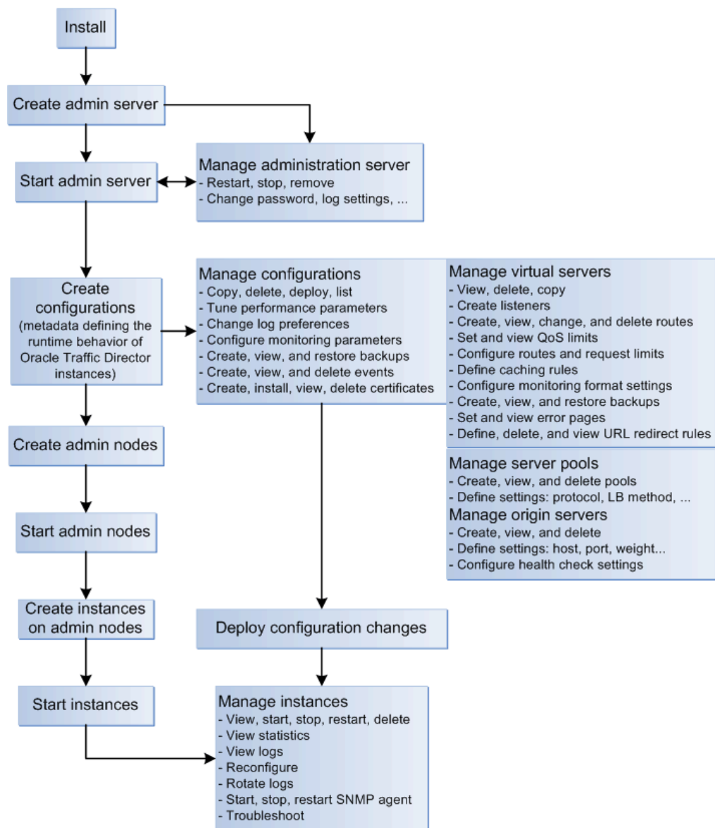
Figure 1-2 Oracle Traffic Director Administration Workflow
