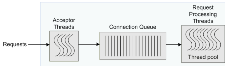
Figure 14-1 Connection Handling in Oracle Traffic Director
