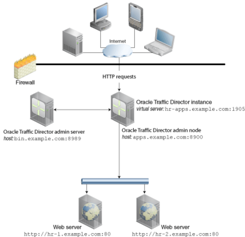
Figure 1-3 Oracle Traffic Director Deployment Example
