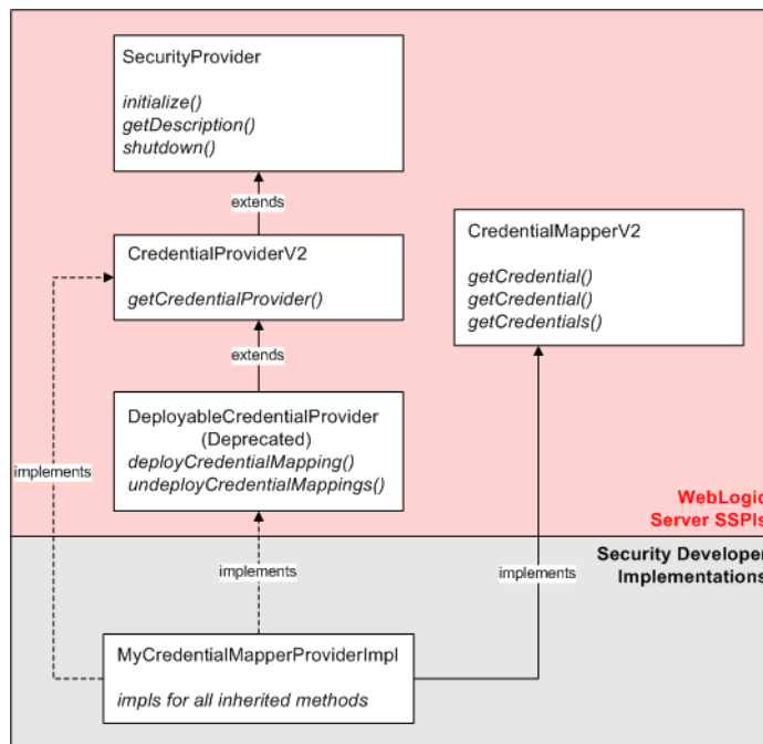
Figure 3–3 Credential Mapping SSPIs and a Single Runtime Class
