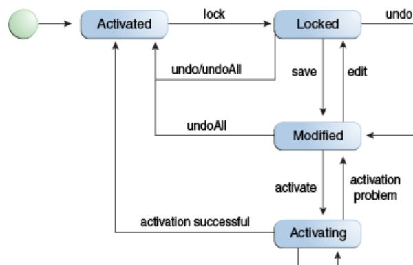
Figure 4-4 Configuration Management State Diagram
