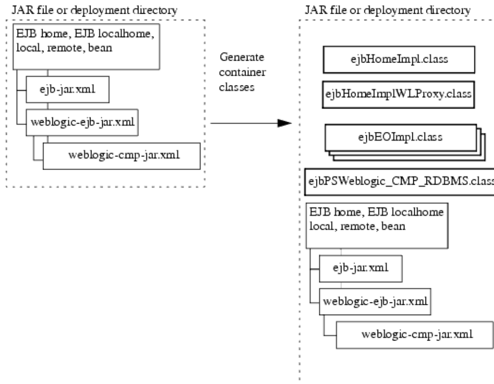
Figure 4–2 Generating EJB Container Classes
