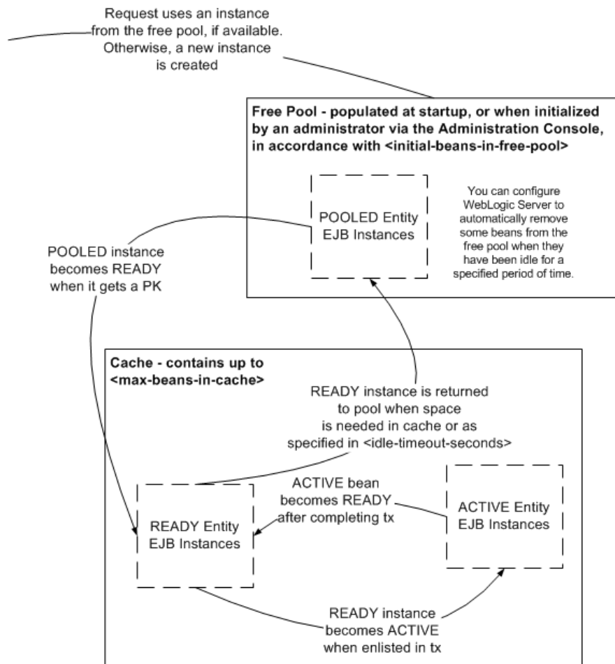
Figure 6–1 Entity Bean Life Cycle
