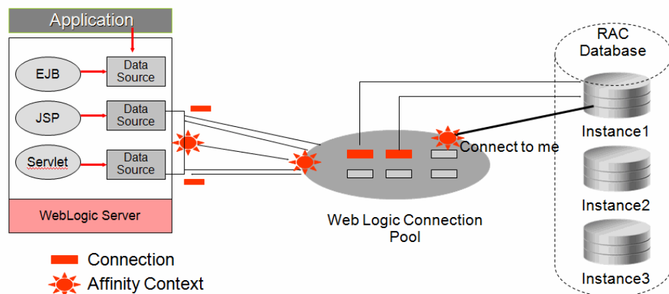
Figure 6-4 Session Affinity
