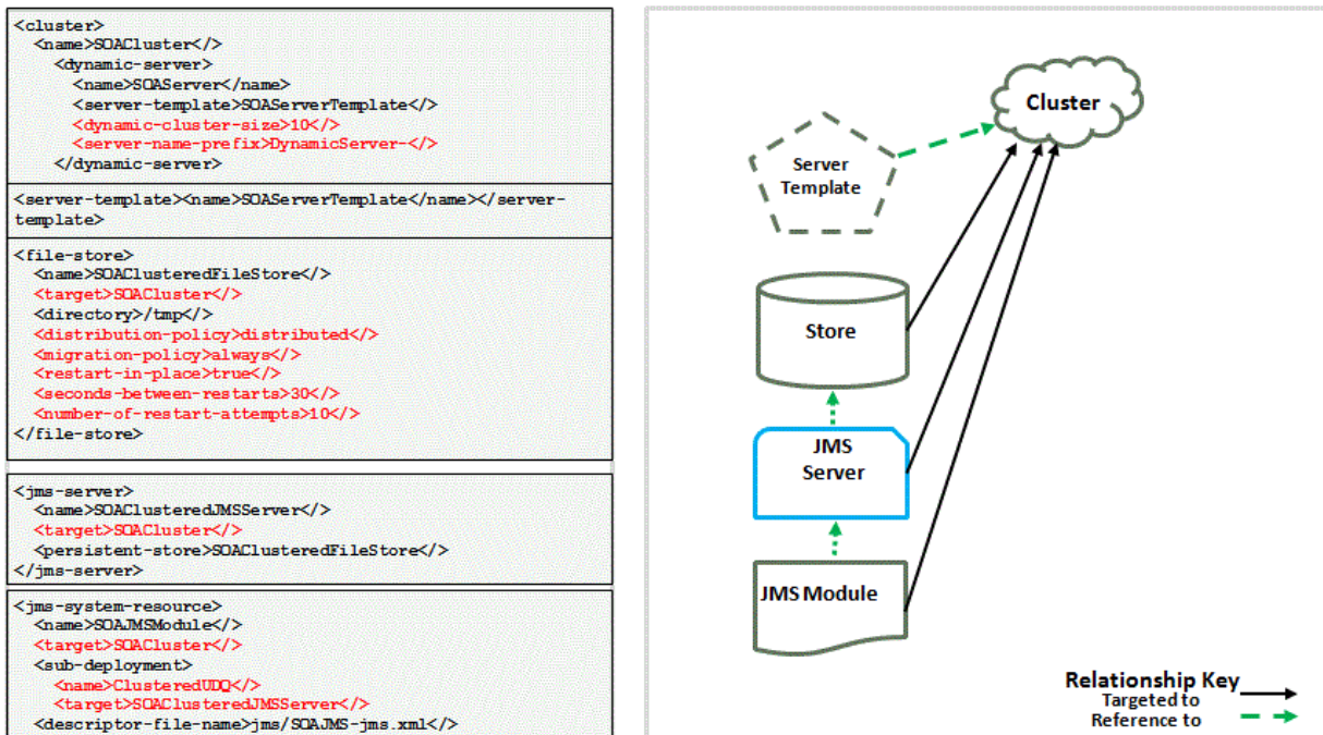
Figure 5-1 Dynamic Clustered JMS
