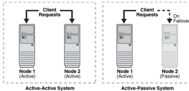
Figure 13–2 Failover Modes
