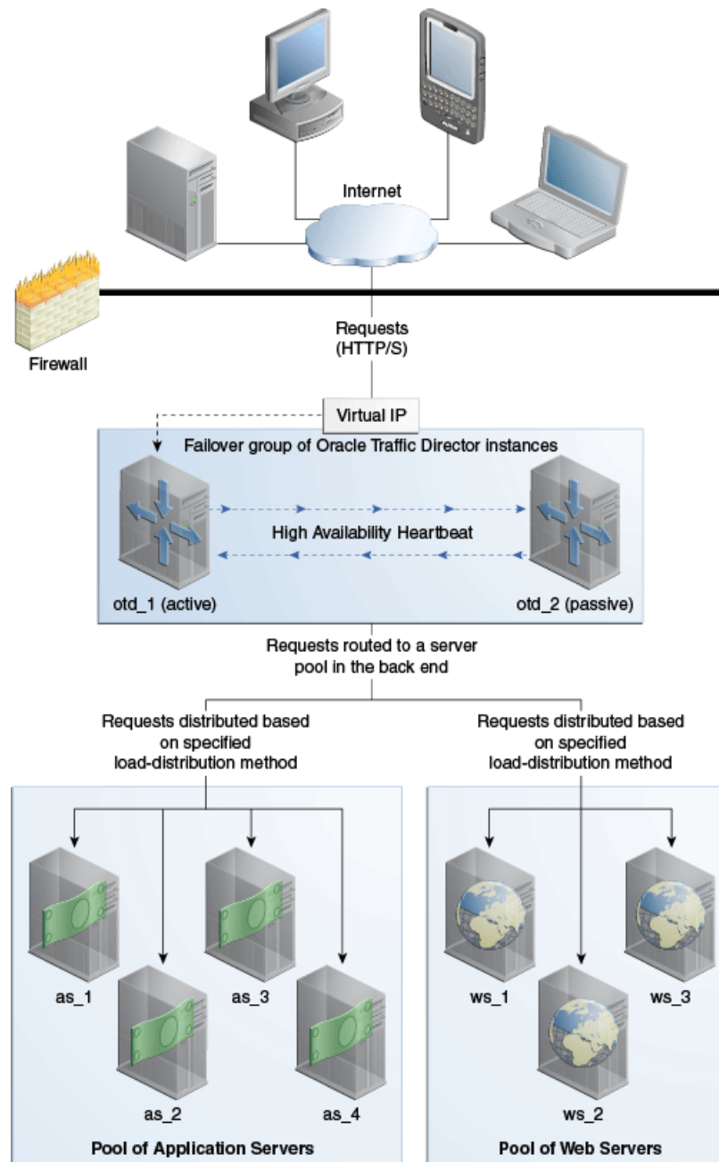
Figure 13–1 Oracle Traffic Director Network Topology: Active-Passive Failover Mode
