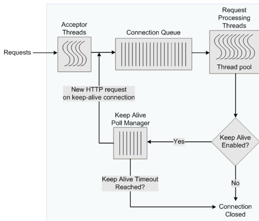
Figure 14–2 Connection Handling in Oracle Traffic Director with Keep Alive Enabled
