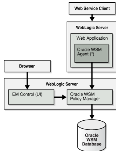
Figure 3-2 OWSM Agent and Policy Manager Interaction
