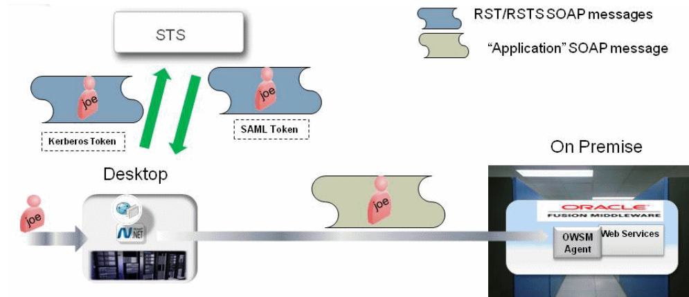
Figure 2–2 STS Token Exchange
