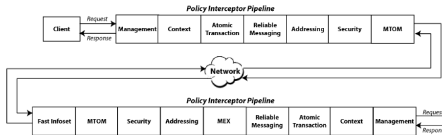
Figure 3-5 Policy Interceptors Acting on Messages Between a Client and Web Service (SOAP)
