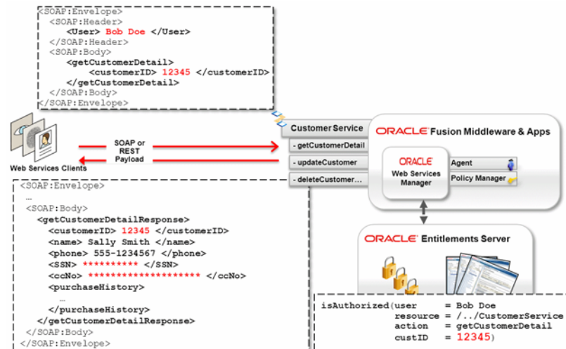
Figure 2–3 Masking Sensitive Data
