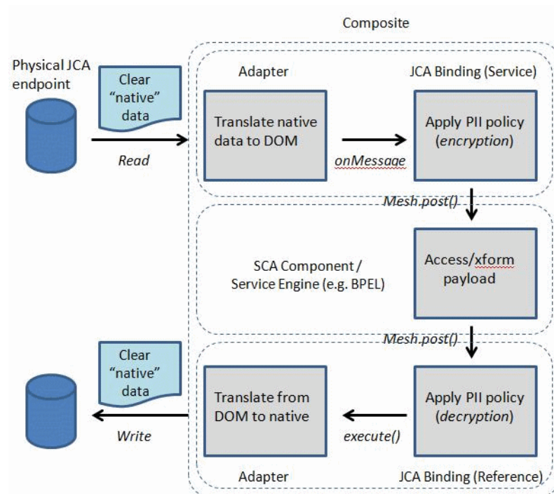
Figure 2-7 JCA Adapter PII Use Case
