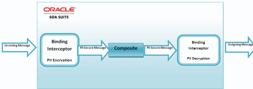
Figure 2–6 Single SOA Composite Use Case
