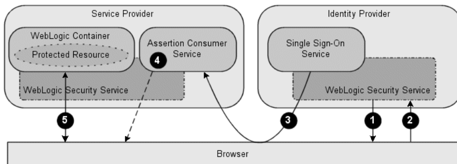
Figure 5–10 Identity Provider Initiated Single Sign-On
