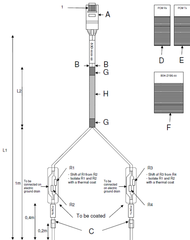
Figure 22- Cable for Falco: sample configuration for unprotected links
