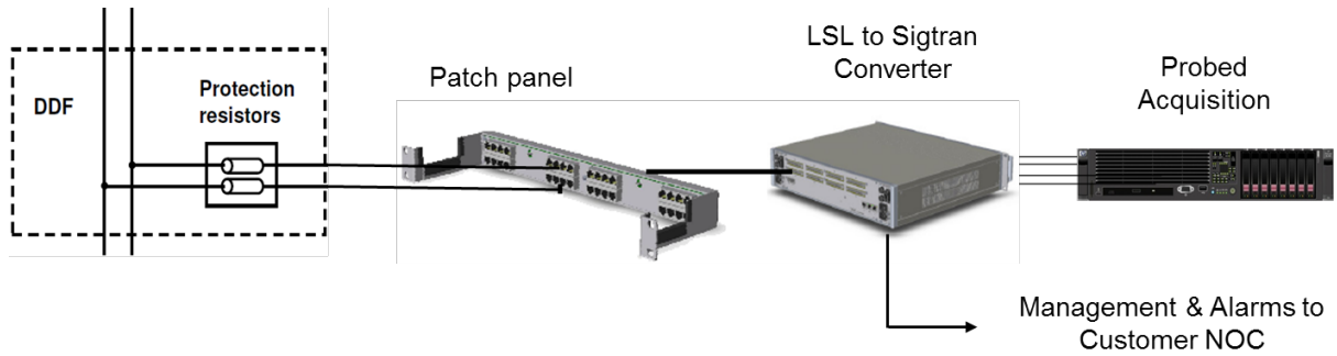
Figure 5 – HSL/LSL to SIGTRAN Converters - connectivity
