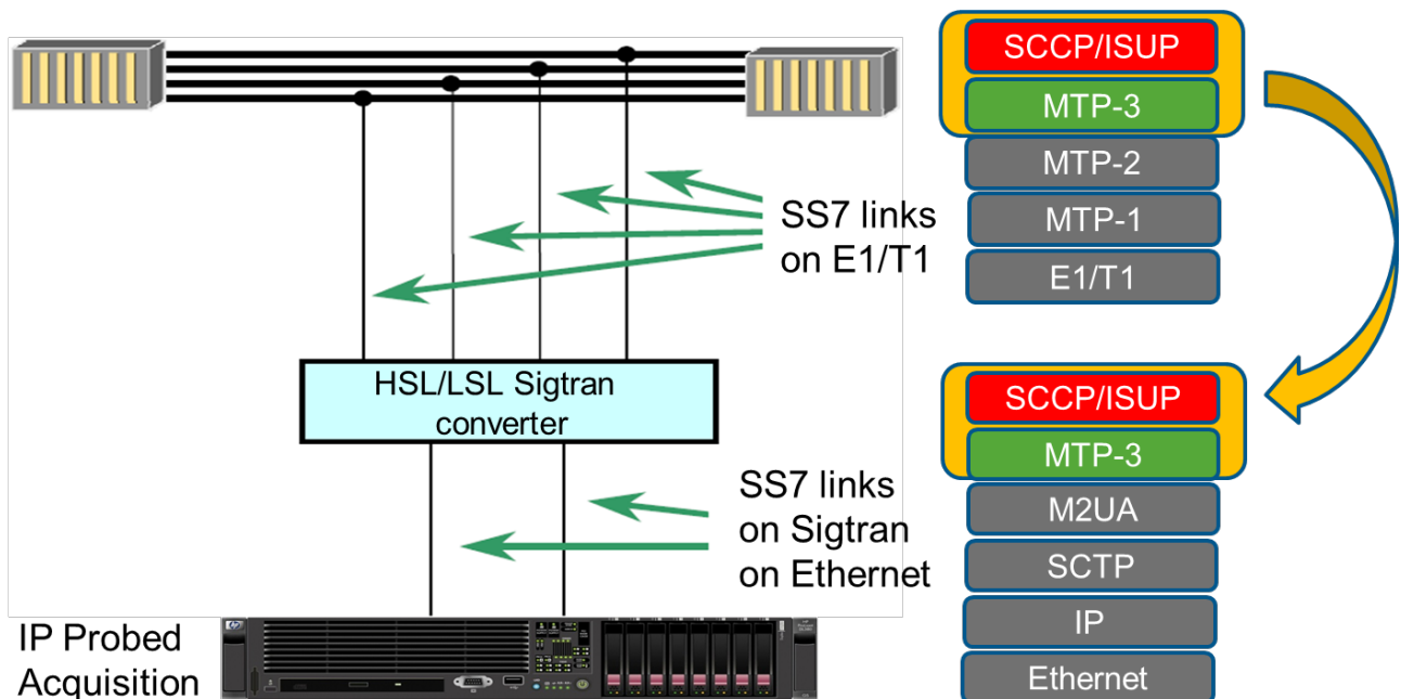
Figure 6 – HSL/LSL to SIGTRAN Converters layers
