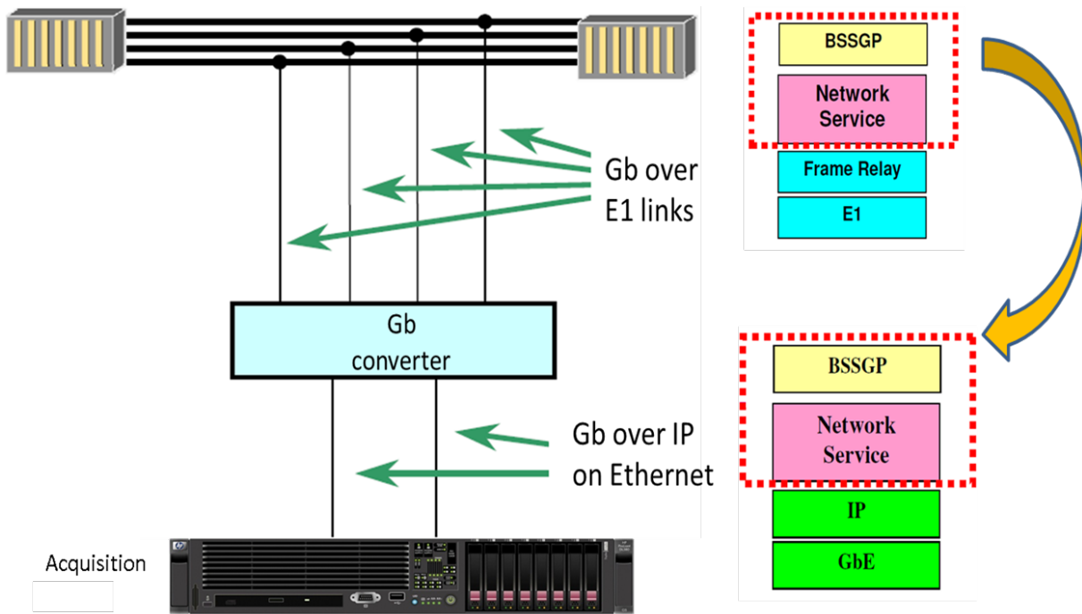
Figure 7 – GboE1 to GboIP Converters – layers
