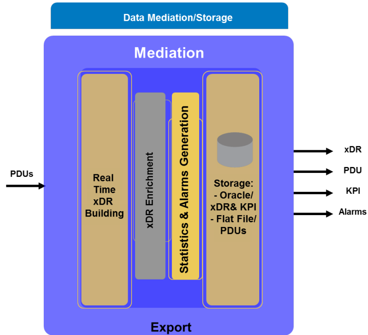
Figure 14 – Mediation Subsystem overview
