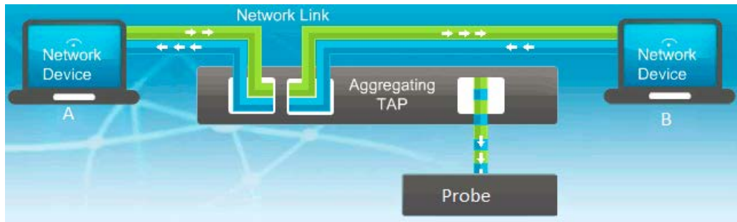
Figure 10 – Link Aggregation mode
