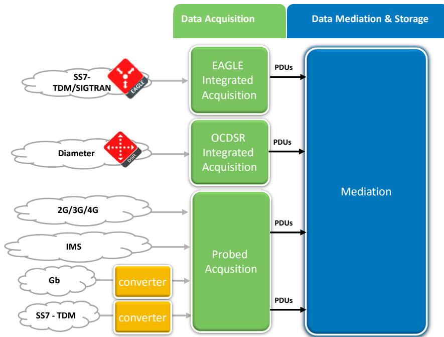
Figure 4 – Acquisition Configurations
