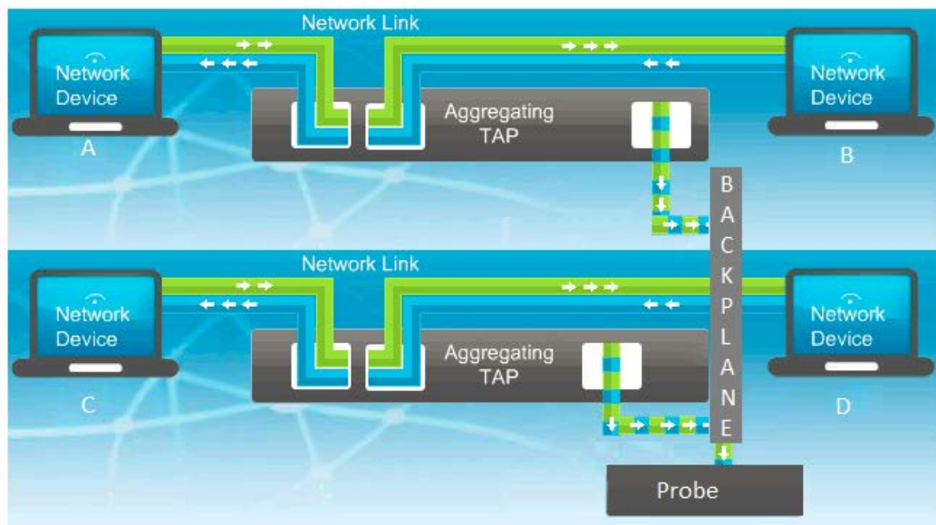
Figure 11 – Backplane Aggregation mode
