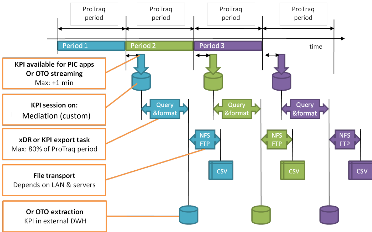
Figure 17 – Data Record and KPI Latency for applications and feeds
