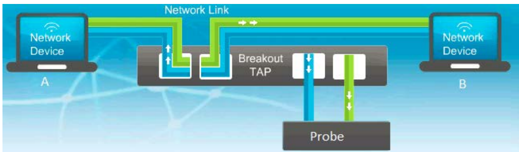
Figure 9 – Breakout mode
