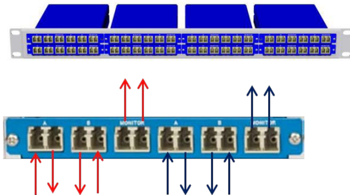
Figure 12 – Passive optical TAP
